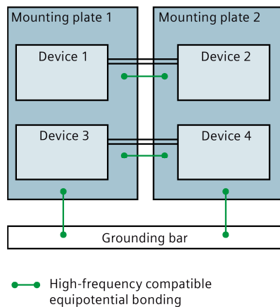
Figure 3-2 High-frequency compatible equipotential bonding in the control cabinet
