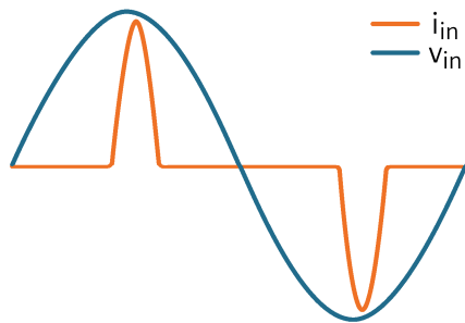
Figure 4-2 Typical progression of the input current of a single-phase converter
