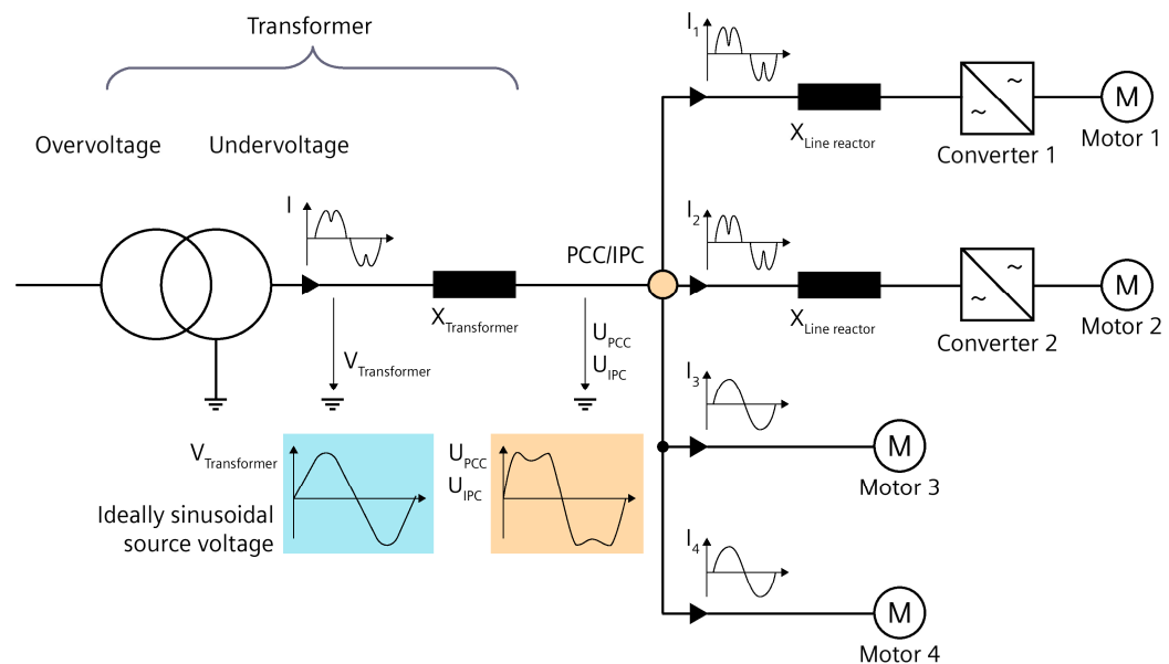
Figure 4-1 A low-voltage network supplied via a transformer with sinusoidal source voltage
