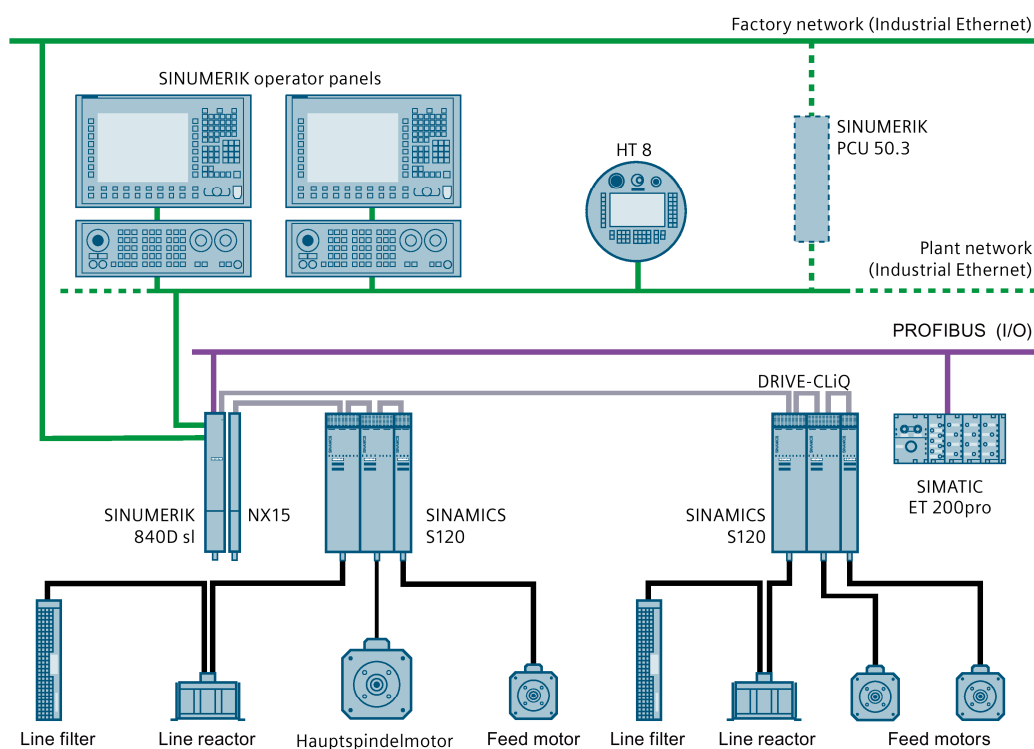
Figure 1-1 2 SINAMICS S120 power drive systems with higher-level SINUMERIK control (the SINUMERIK is not part of the power drive system)
