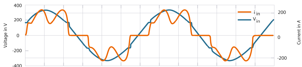
Figure 4-3 Typical progression of the input current of a three-phase converter
