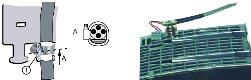
① Shield clamp
