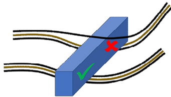
Figure 2-4 Laying single cores of the mains power input
