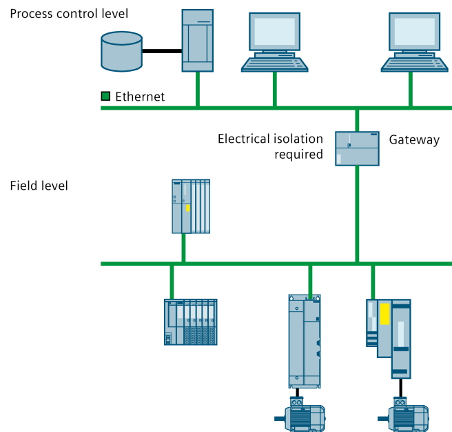
Figure 4-5 Electrical isolation between the process control level and field level
