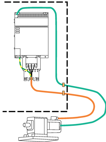
Figure 3-5 Example of an uninterrupted cable routing from the motor to the converter
