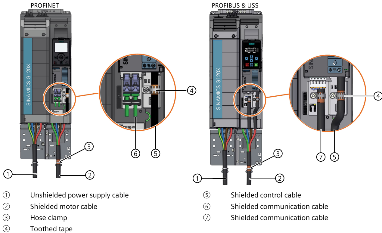
Figure 2-7 Connect cable shields (example for converter G120X IP20 FSD)
