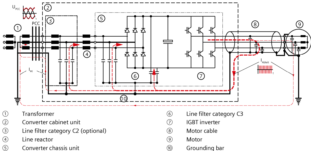
Figure 4-4 Reduction of high-frequency interference with line filters
