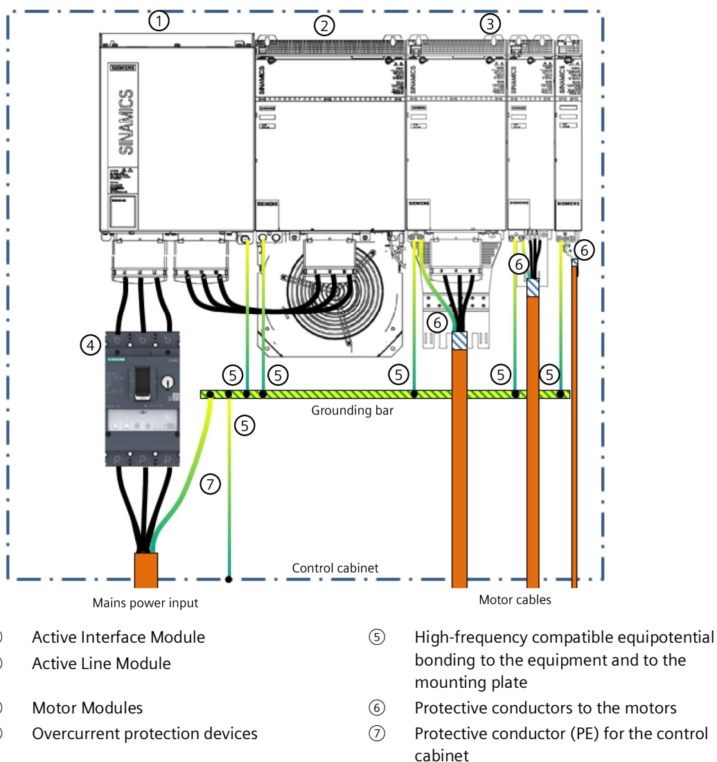
Figure 3-1 Protective connection concept, SINAMICS S120 Booksize (example)
