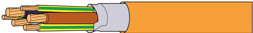
Figure 2-8 Shielded, symmetrically arranged three-phase cable with 3 protective conductors, e. g. PROTOFLEX EMV-FC 2XSLCY-J 0.6/1 kV from Prysman.
