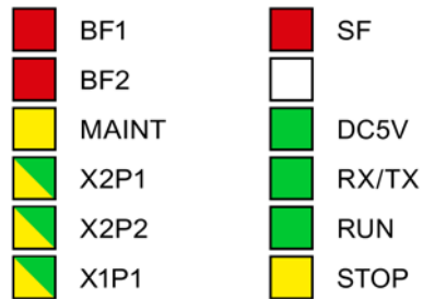
Figure 4-1 LED du CP 343-1 Advanced
