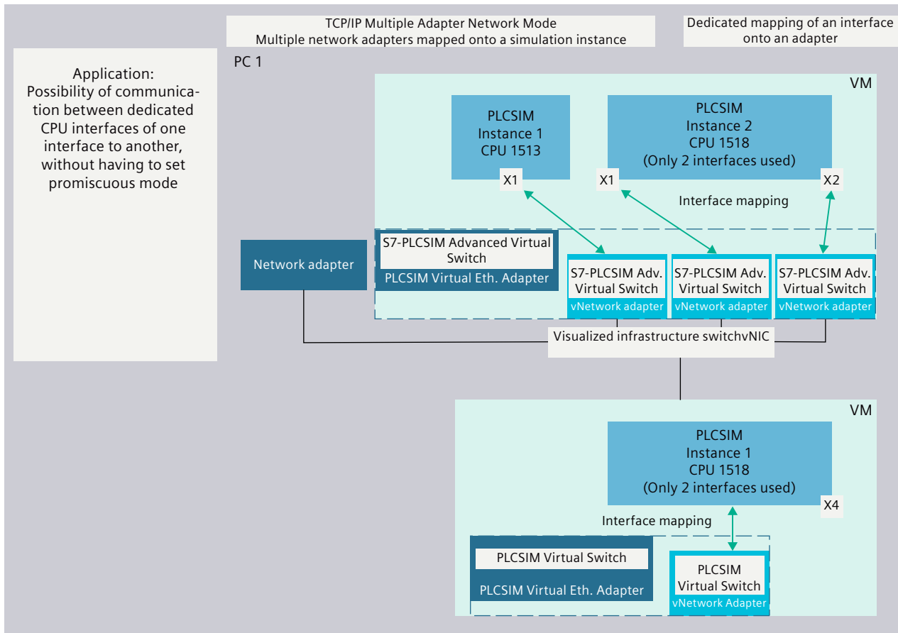
Figure 4-8 Application 2
