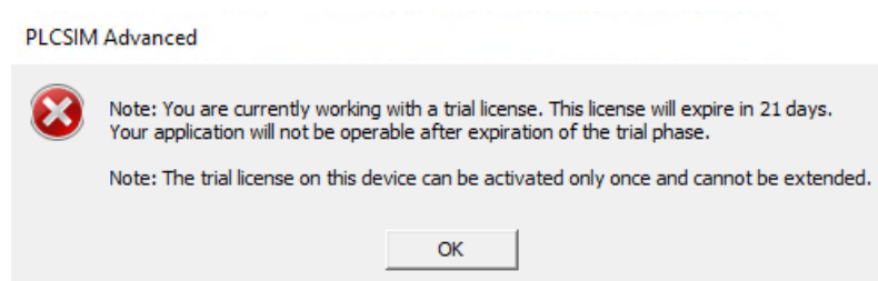
Figure 3-2 Trial License
