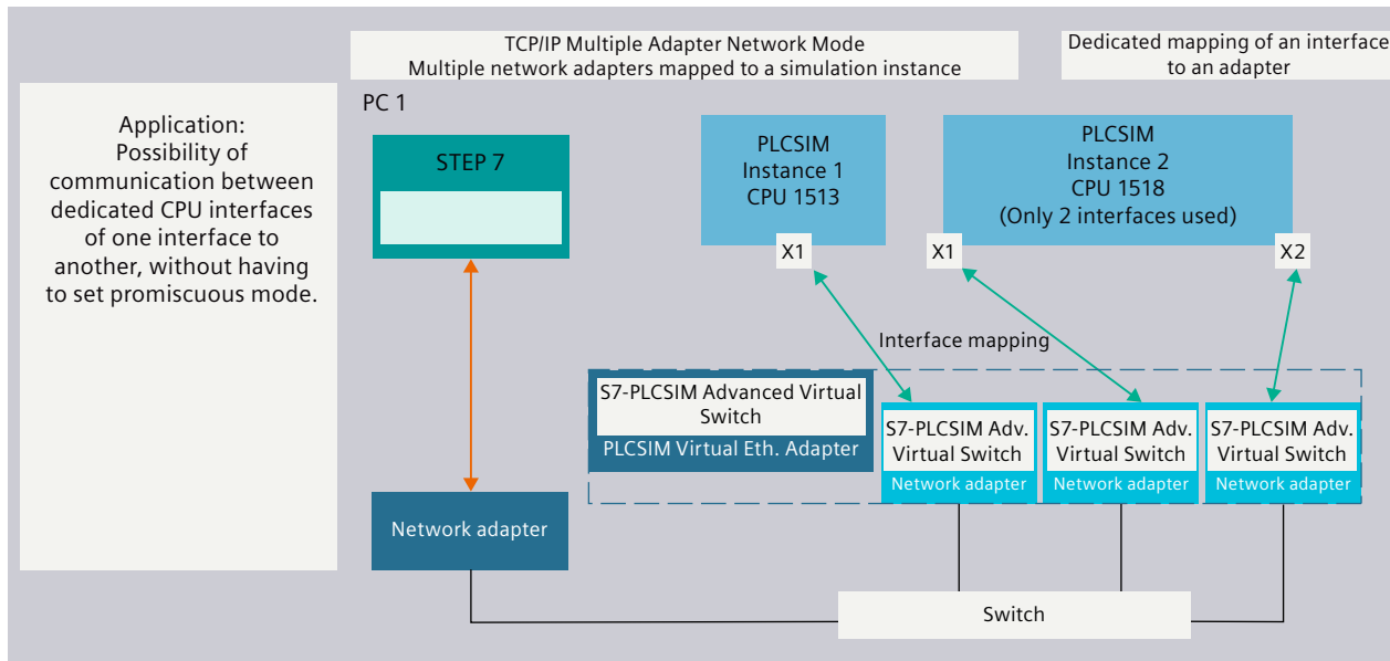
Figure 4-7 Application 1
