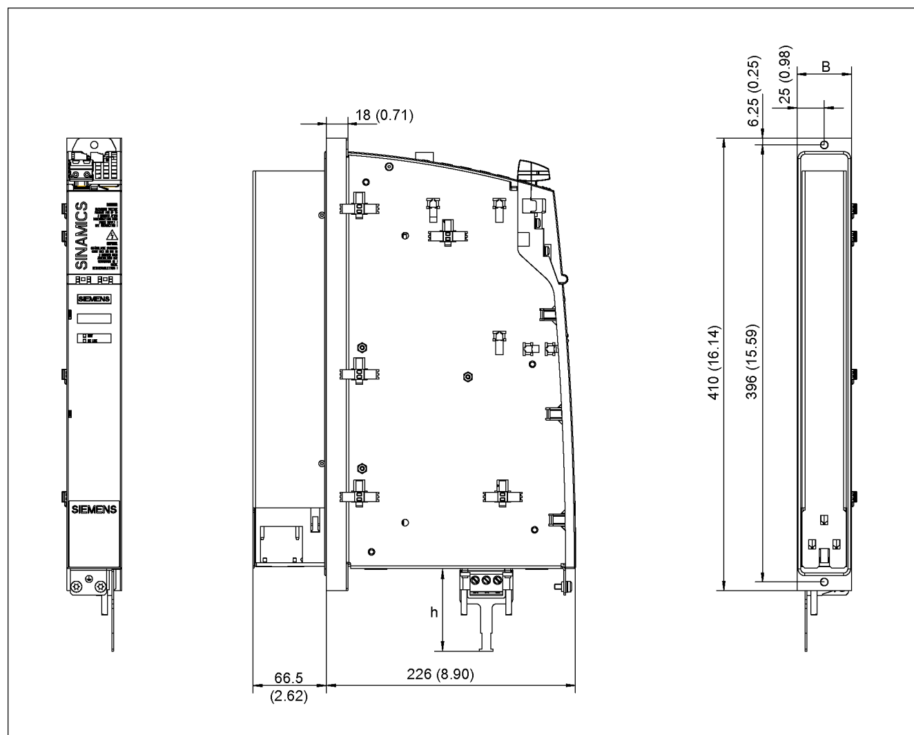
Figure 3-34 Dimension drawing of Smart Line Module with external air cooling (5 kW and 10 kW)
