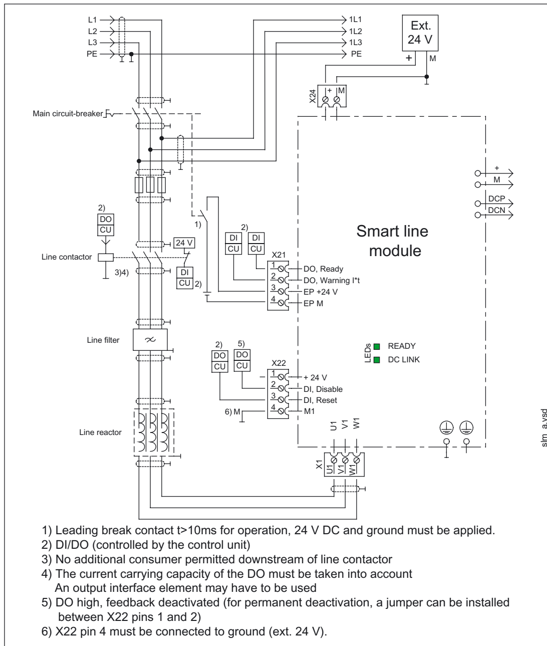
Figure 3-26 Example connection of Smart Line Module
