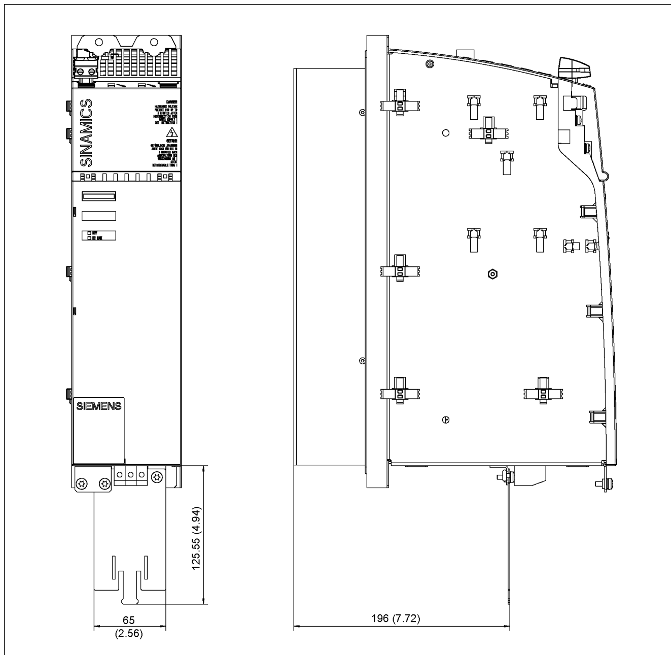
Figure 6-7 Dimension drawing of shielded terminal plate on a 100 mm module with external air cooling
