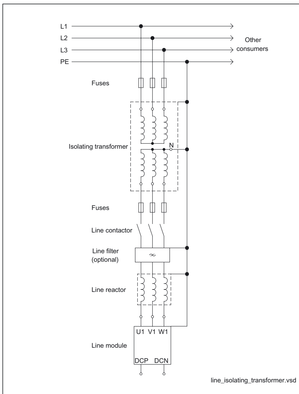
Figure 2-5 Isolating transformer
