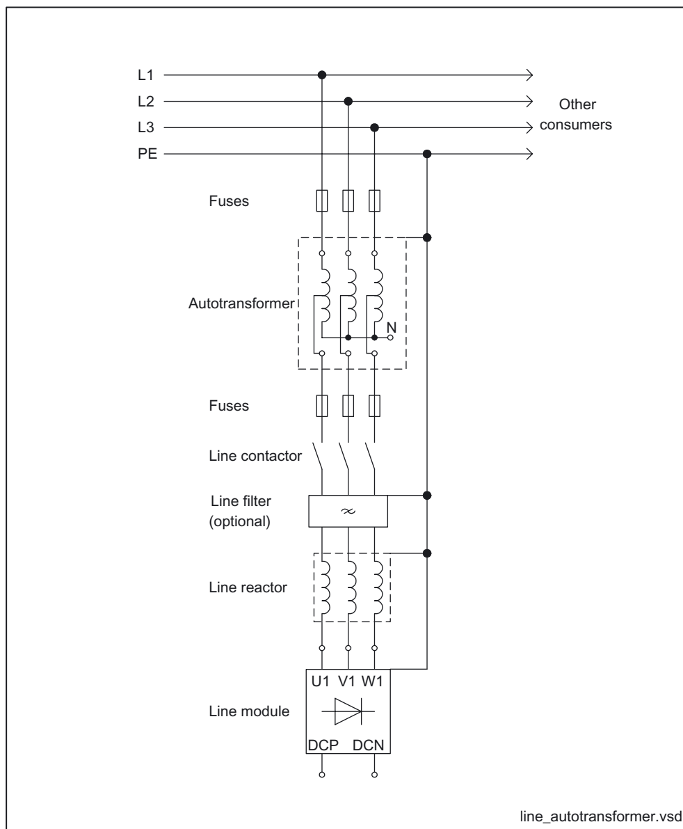
Figure 2-4 Autotransformer
