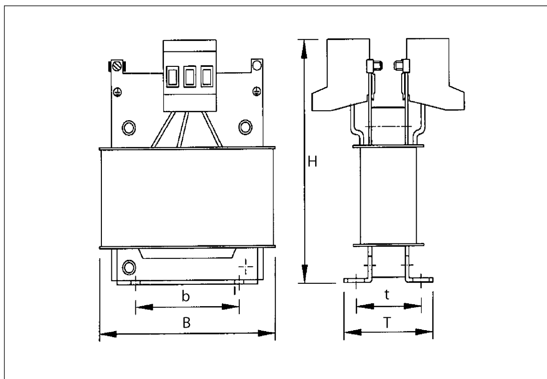
Figure 2-12 Dimension drawing of line reactor for Smart Line Module
