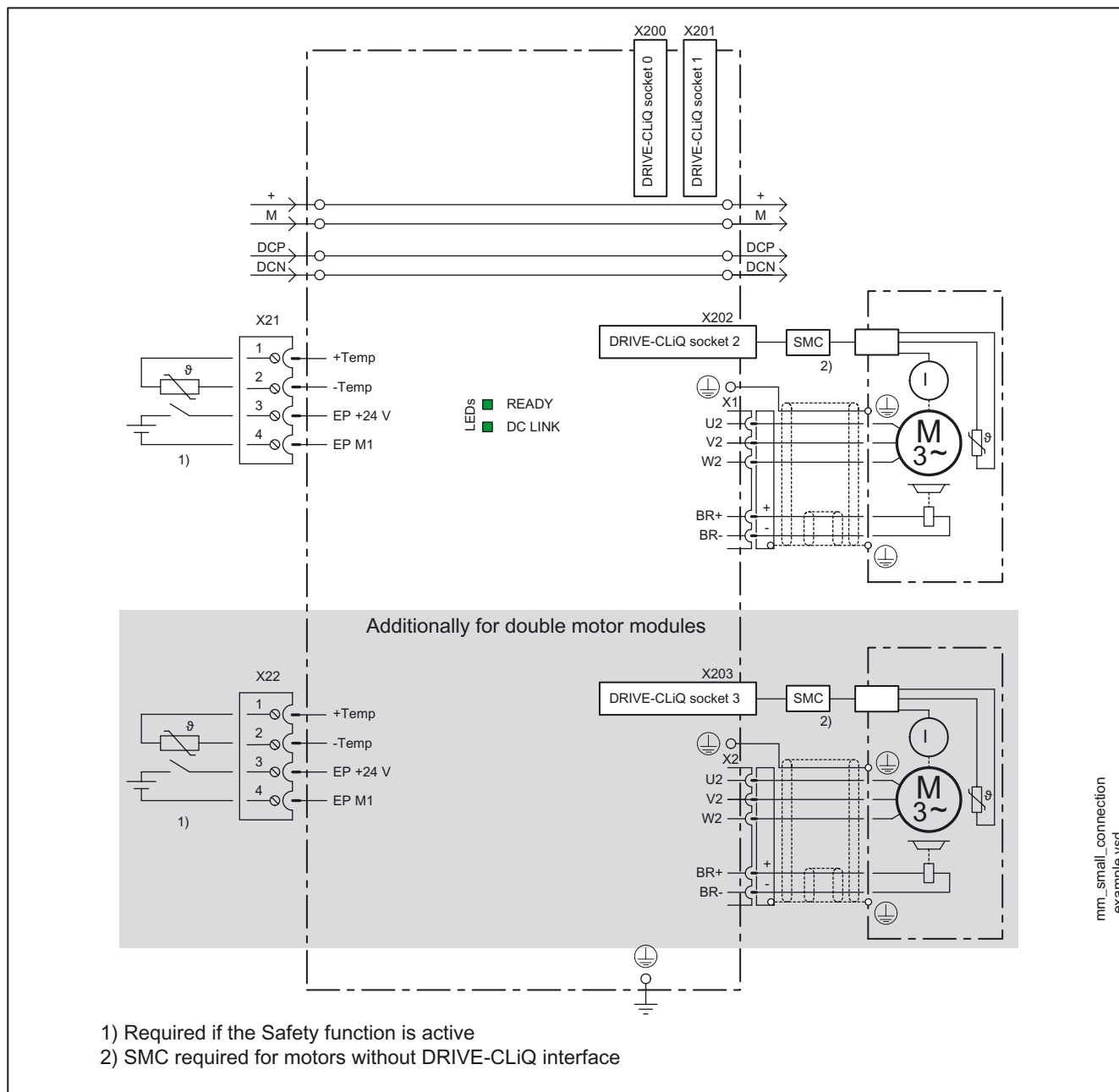
Figure 4-20 Example connection of motor modules 3 A to 30 A and 2x3 A to 2x18 A
