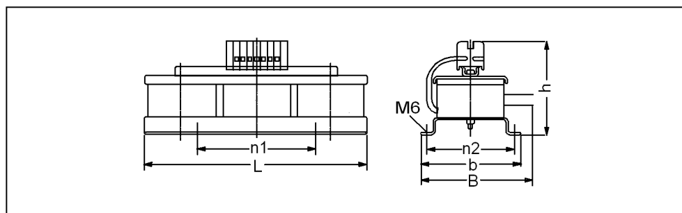
Figure 2-11 Dimension drawing of line reactor
