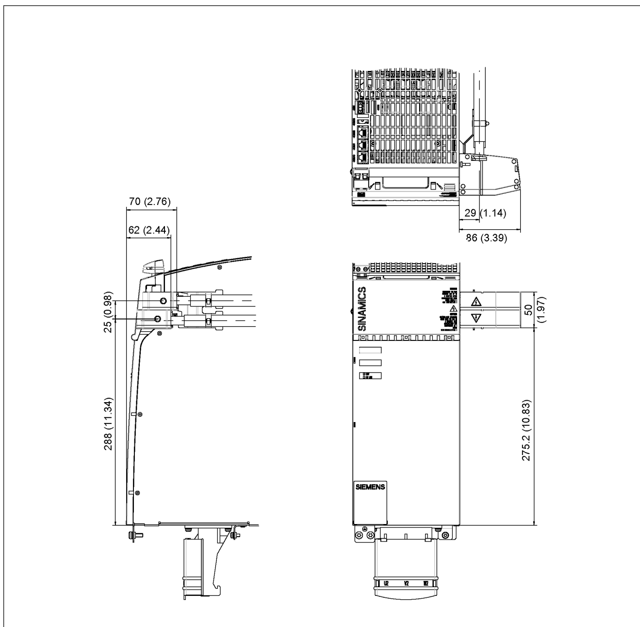
Figure 6-15 Dimension drawing of 150 mm module with DC link adapter for two-row configuration (35 mm 2 to 95 mm 2 )
