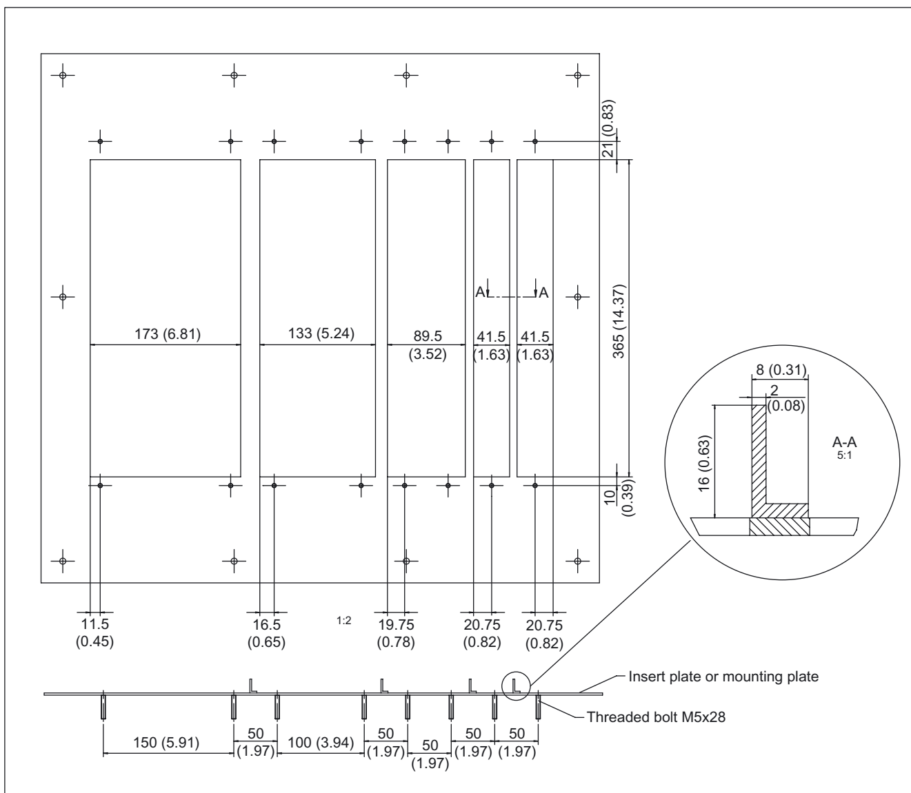
Figure 3-18 Example: mounting plate with a drive line-up
