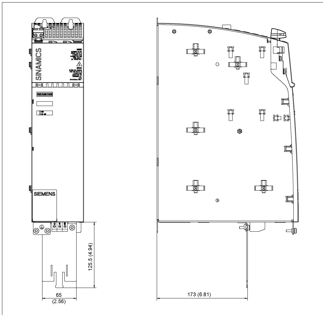
Figure 6-3 Dimension drawing of shielded terminal plate on a 100 mm module with internal air cooling
