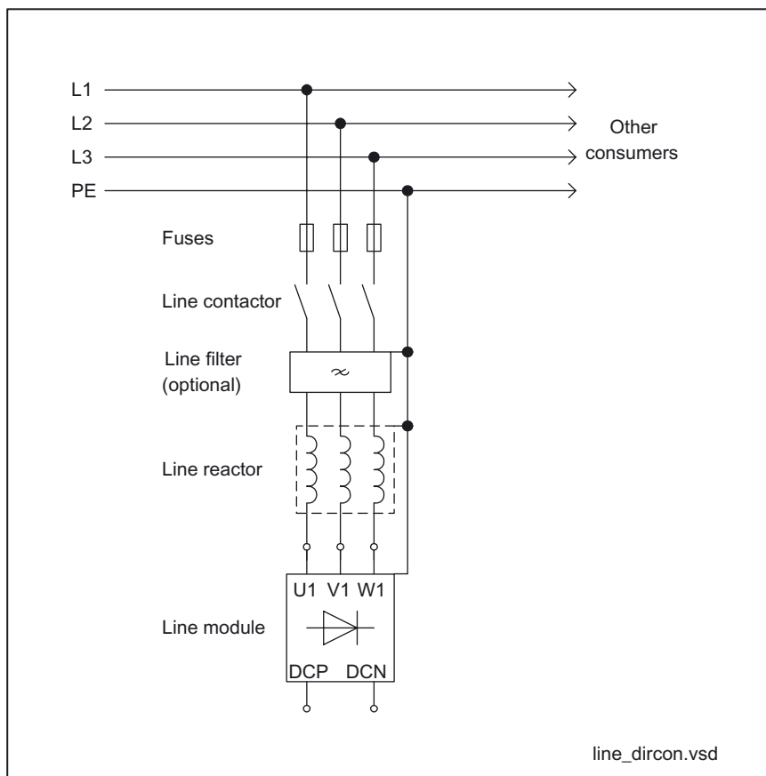
Figure 2-3 Direct operation on the supply network
