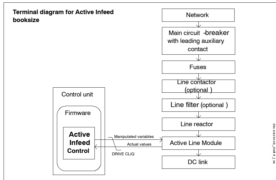
Fig. 1-1 Schematic structure of Active Infeed (booksize)
