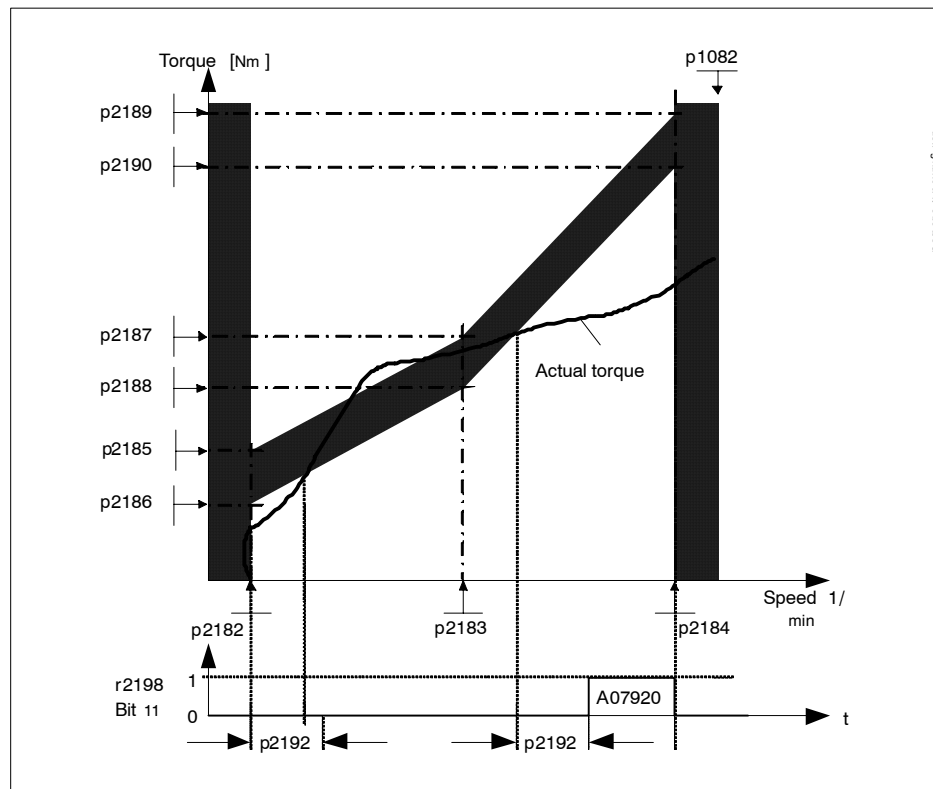
Fig. 4-3 Load monitoring
