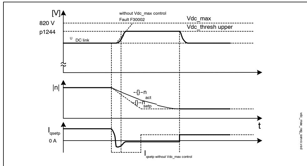
Fig. 3-20 Switching Vdc_max control on/off
