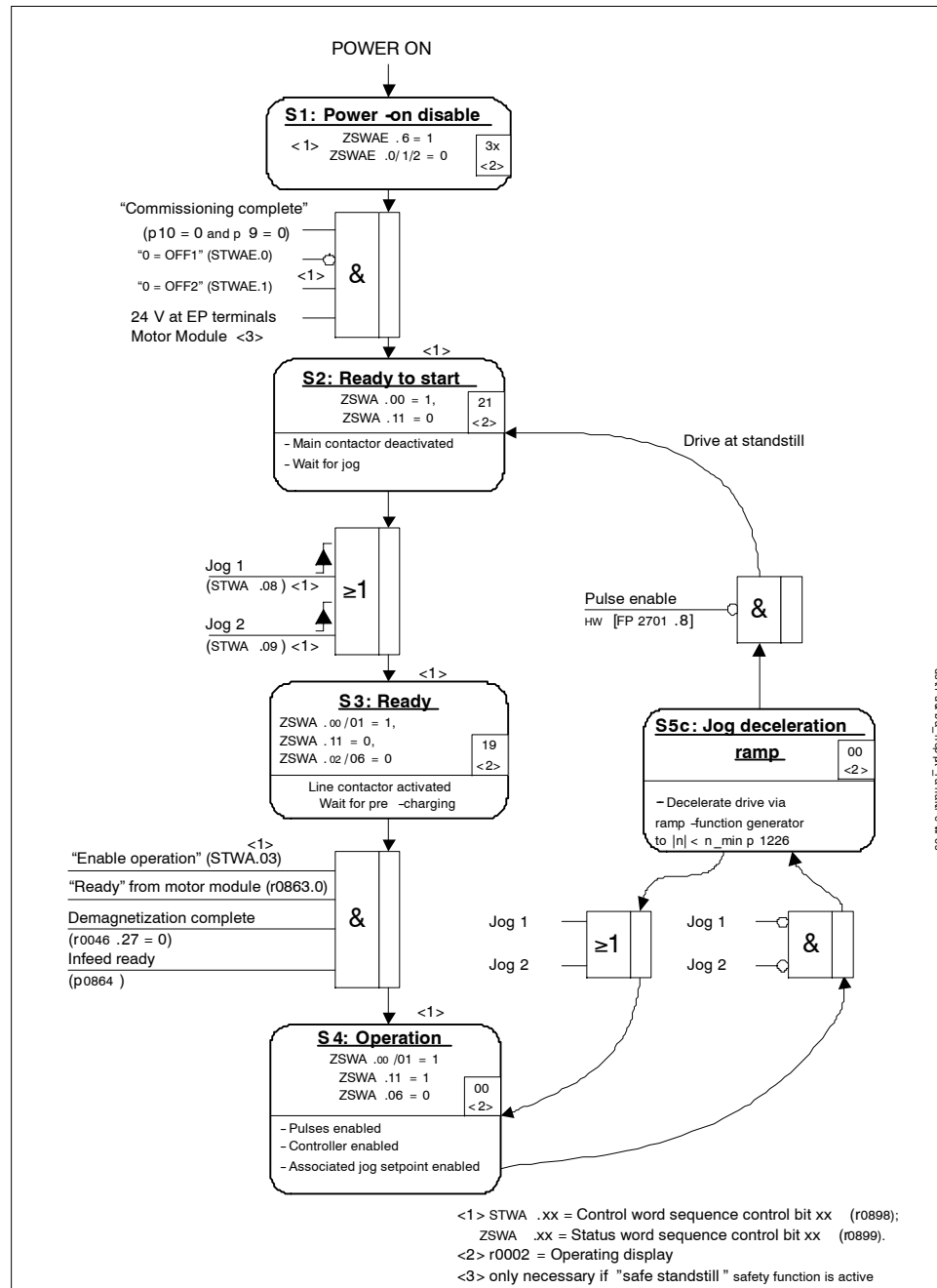
Fig. 2-4 Jog sequence
