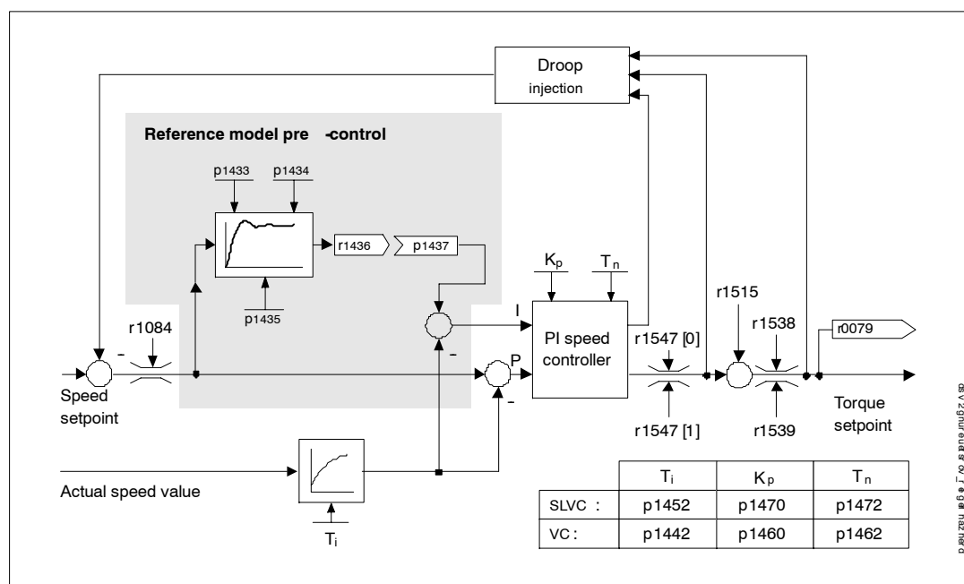
Fig. 3-30 Reference model
