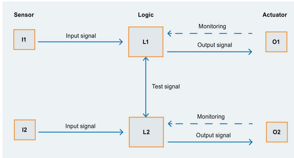
Figure 5-14 Designated architecture for Category 3
