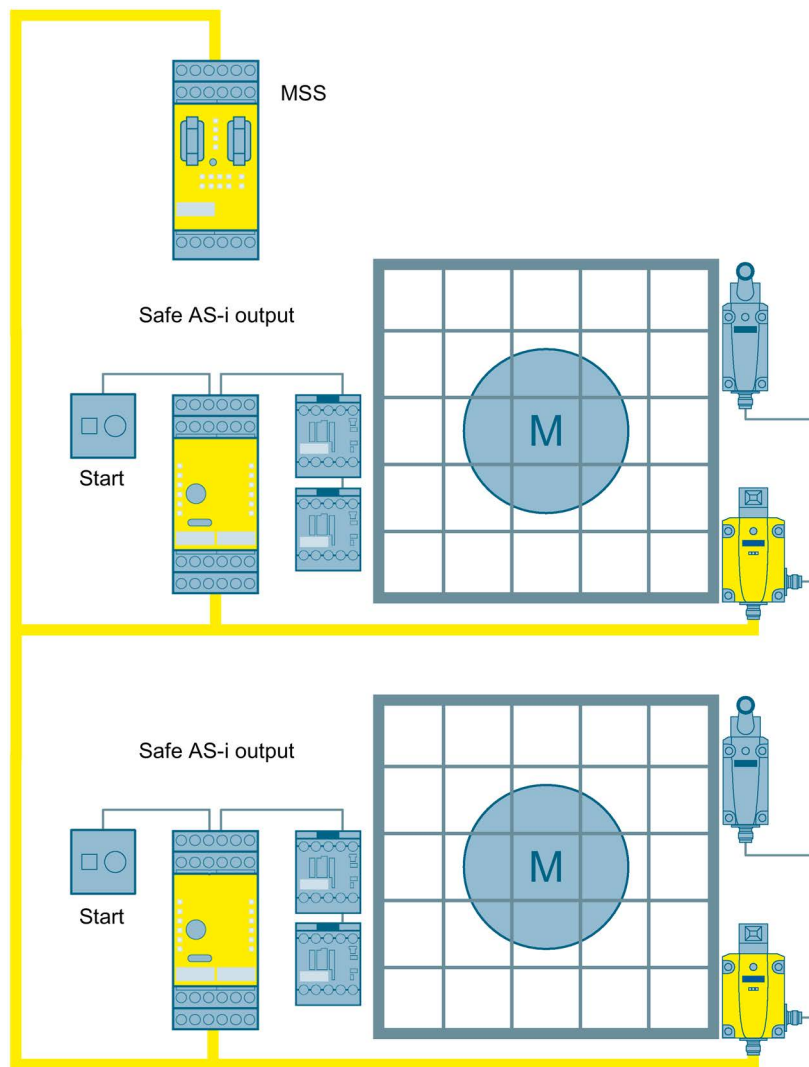
Figure 3-15 Protective door monitoring via AS-i to SIL 3 or PL e with a Modular Safety System
