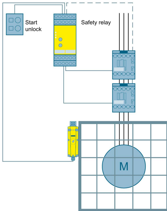
Figure 3-18 Protective door monitoring with tumbler to SIL 2 or PL d with a safety relay
