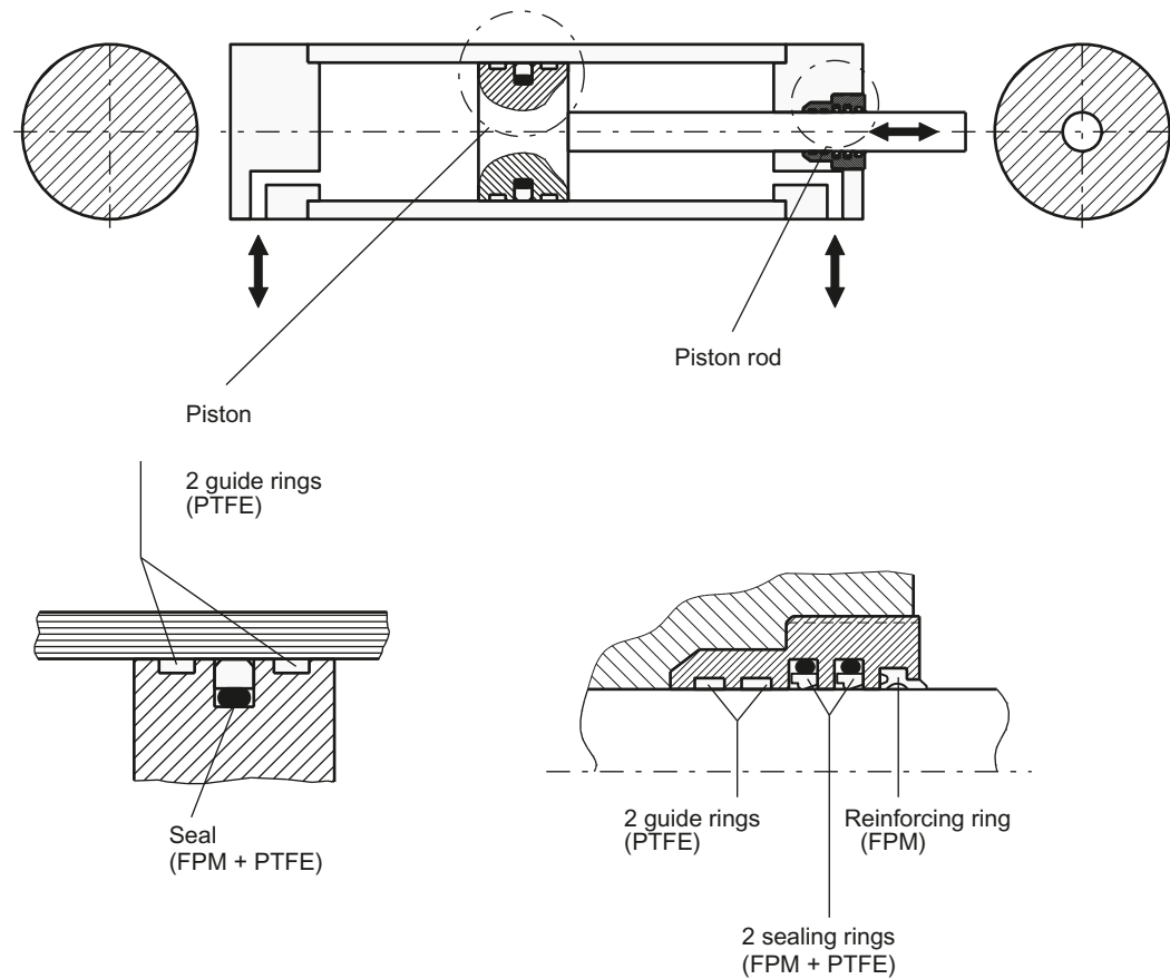
FPM Fluororubber PTFE Polytetrafluoroethylene (Teflon)≠ Figure A-20 Cylinder
