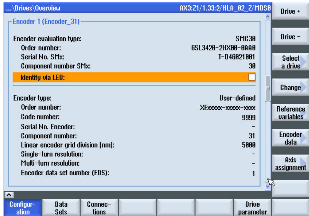
Figure 5-17 Encoder overview
