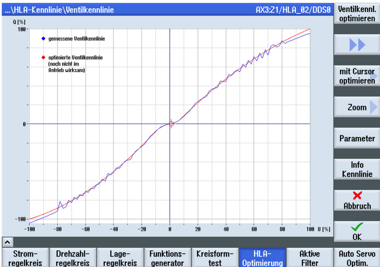
Figure 5-32 Graphically tuning the valve characteristic
