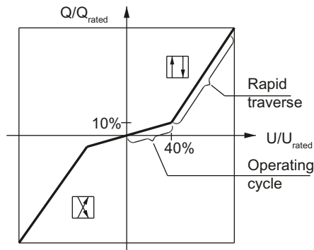
Figure A-8 Flow rate characteristic with transition point, example 40 % transition
