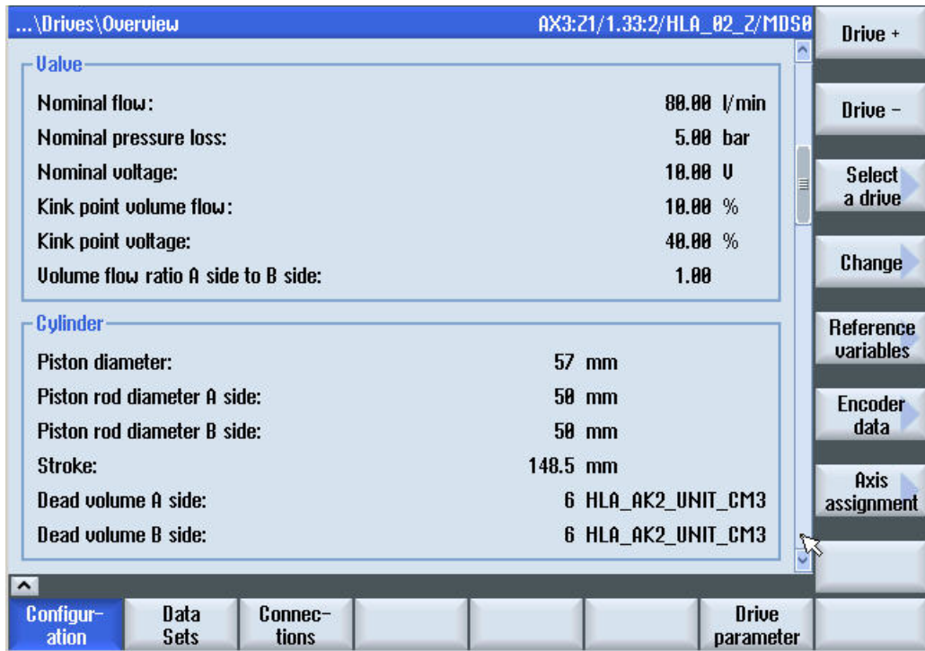
Figure 5-16 Valve/cylinder overview
