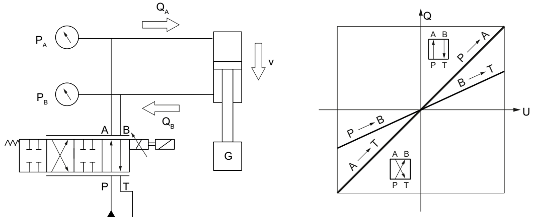
Figure 4-3 Asymmetrical characteristics
