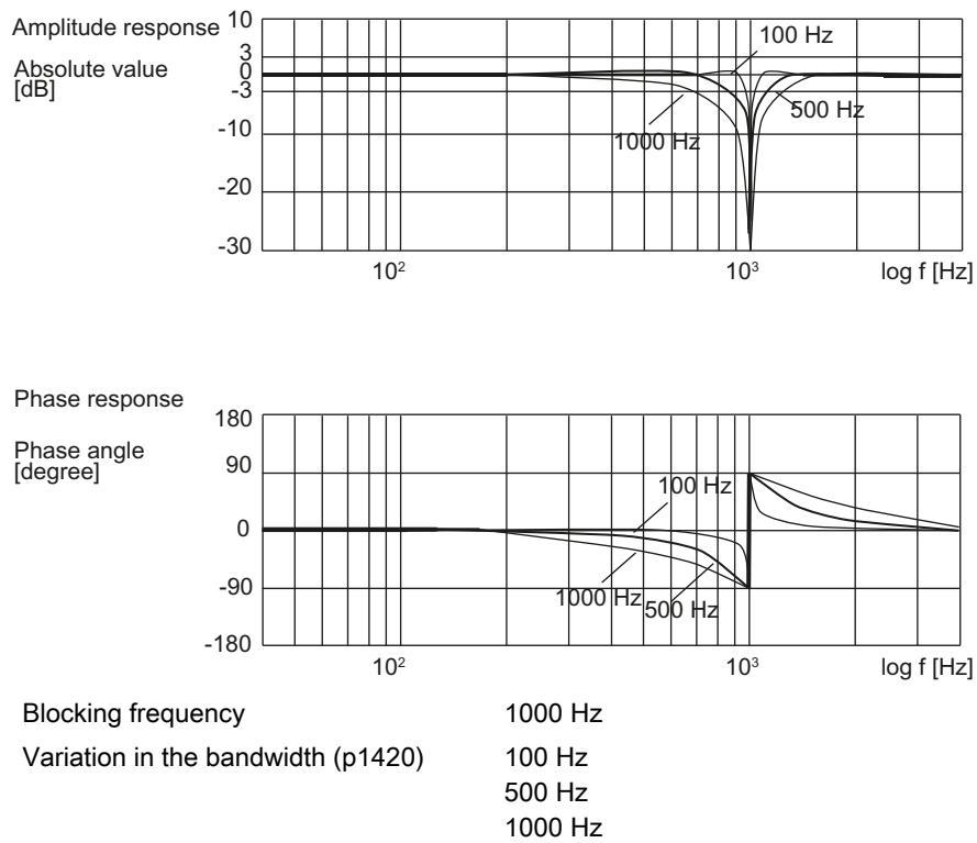
Figure 6-5 Frequency response of the non-damped bandstop filter
