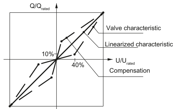
Figure A-10 Electrical valve transition point compensation
