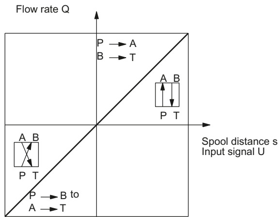
Figure A-6 Linear flow rate characteristic
