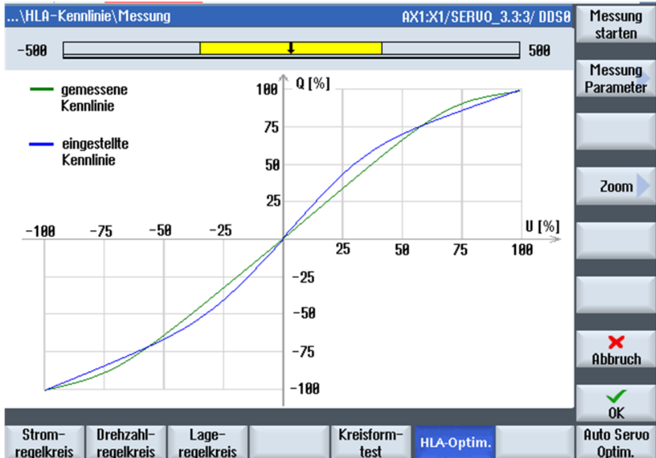
Figure 5-28 Characteristic: Measurement
