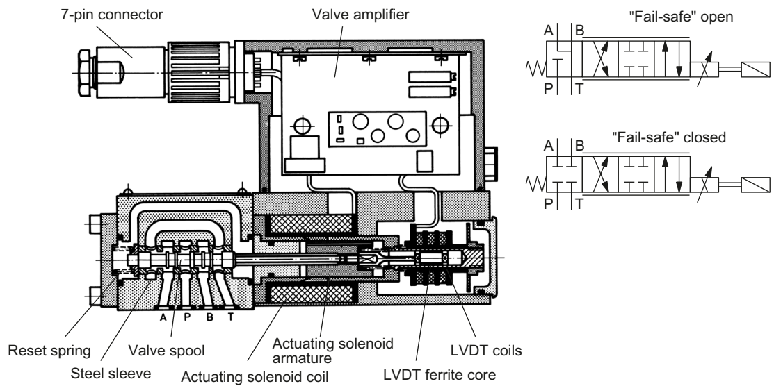
Figure A-13 Directly-controlled servo solenoid valve
