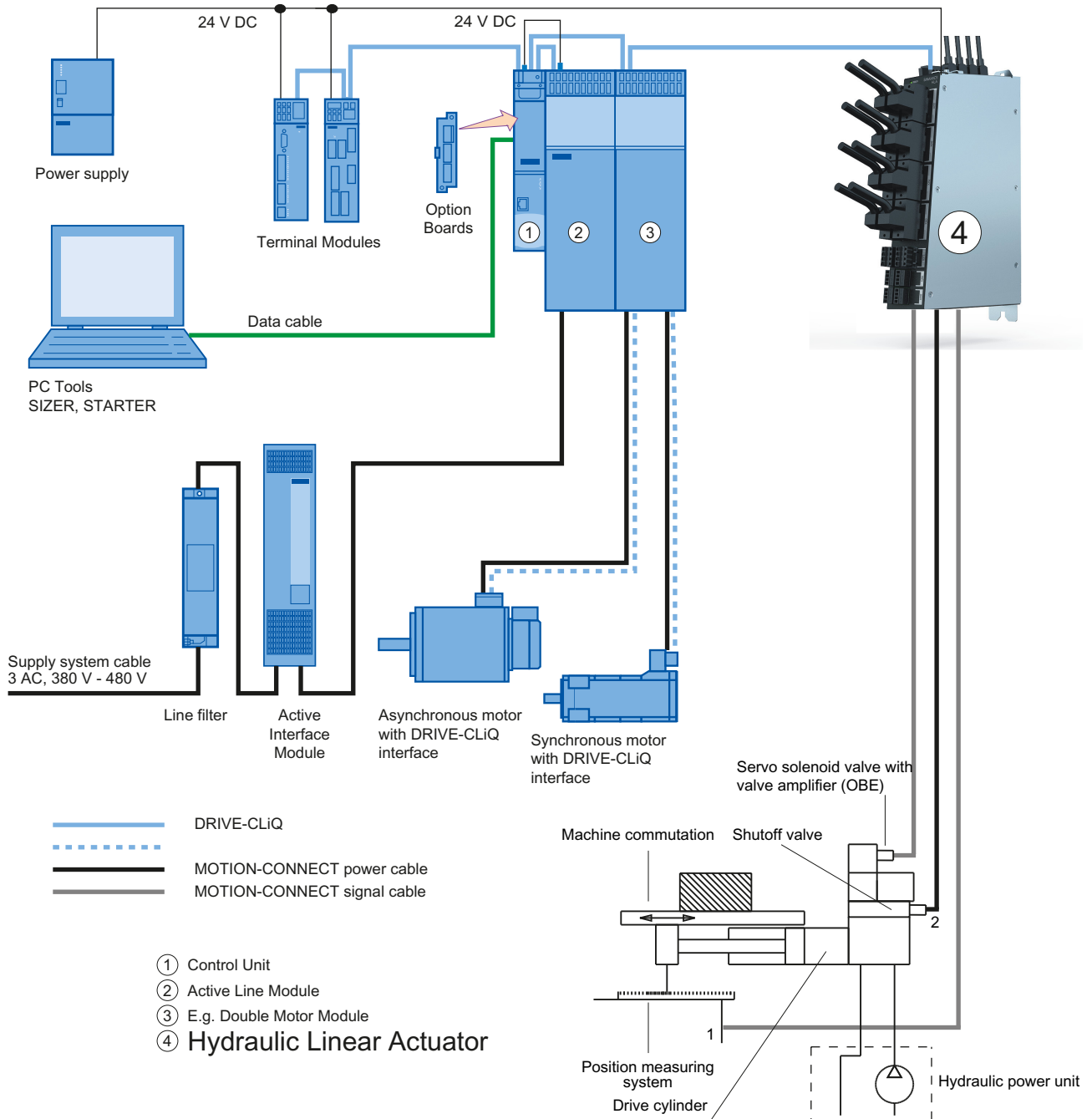
Figure 3-1 Example of a SINAMICS drive system with electrical and hydraulic components
