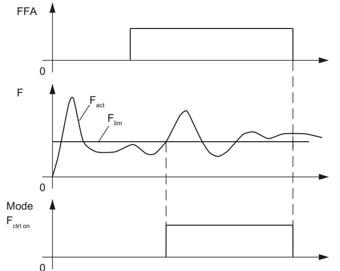
Figure 6-11 Deselecting force control by deactivating the "Travel to fixed stop" function.
