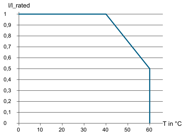
Figure 5-2 Derating for PDC600(F) as a function of the ambient temperature
