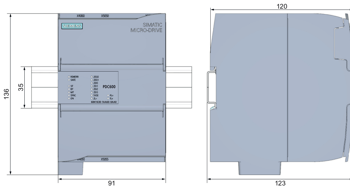
Figure B-1 Dimension drawings of SIMATIC MICRO-DRIVE PDC600(F), front and side view (as examples, depending on mounting rail type used)
