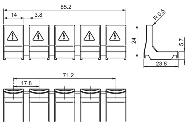
Figure 8-1 5ST3655-0HG
