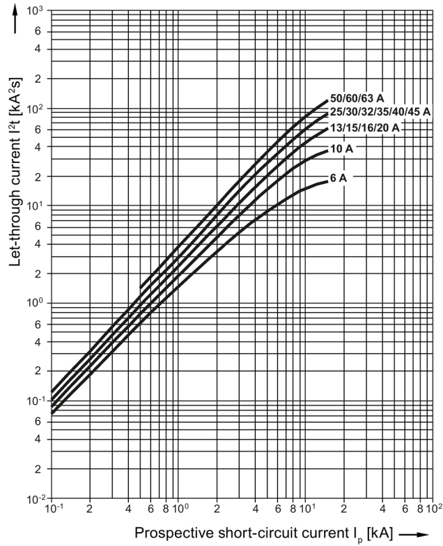
Characteristic B
