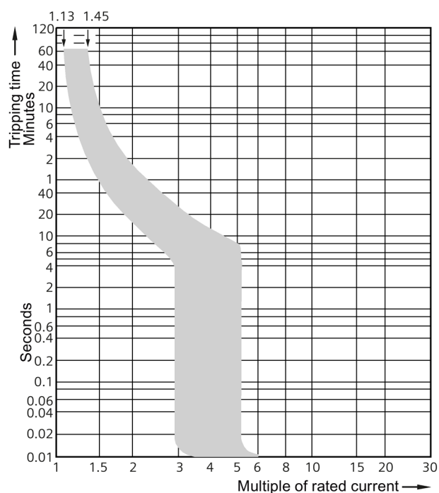
Tripping characteristic B
