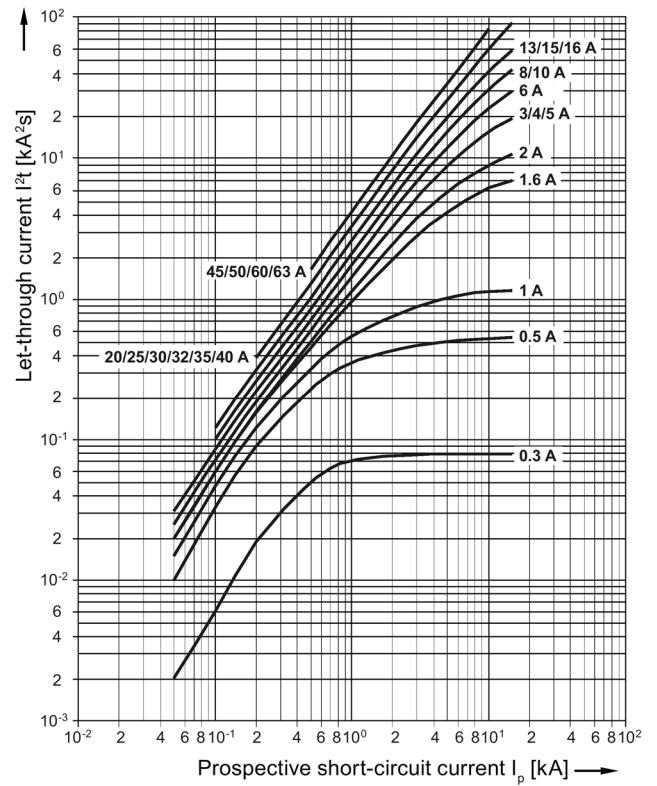
Characteristic C
