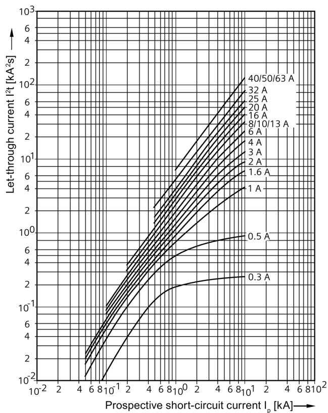
Characteristic D
