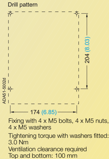
Inverter frame size C with gland plate
