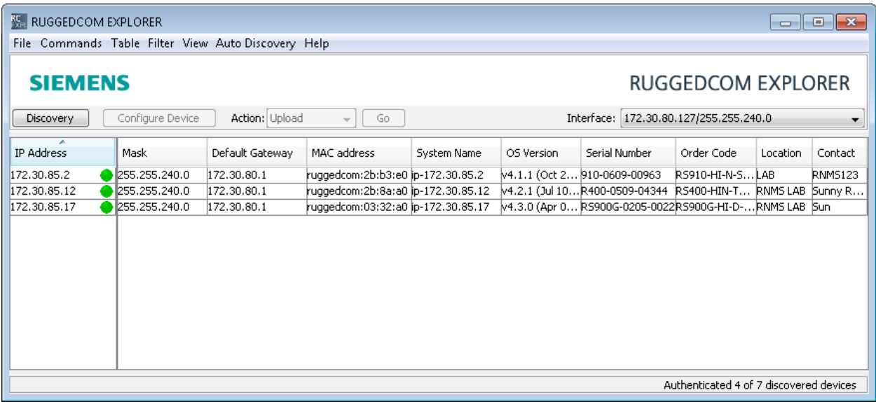
Figure 5: Main Window
