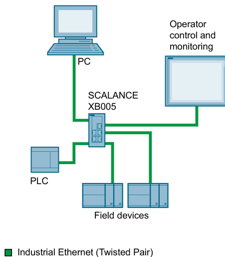
Figure 2-1 Example of an electrical star topology with SCALANCE XB005
