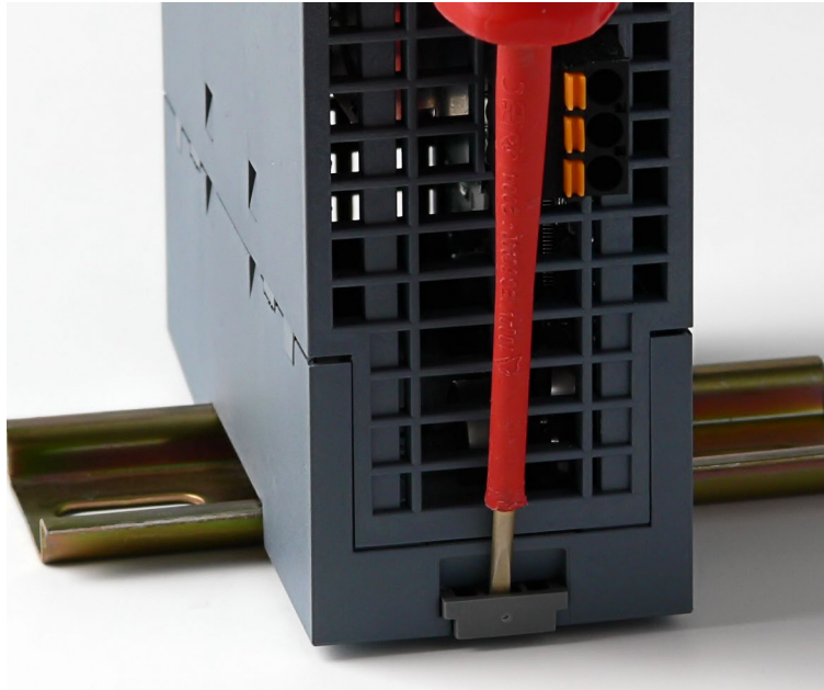
Figure 4-3 Removal from a 35 mm DIN rail
