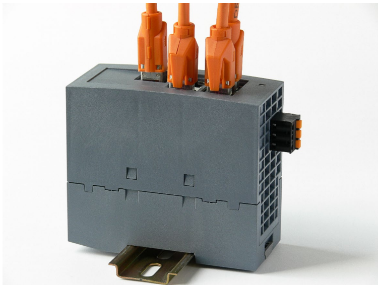
Figure 4-2 SCALANCE XB-000 mounted on the 35 mm DIN rail
