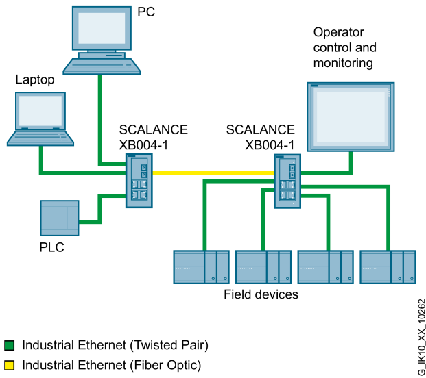
Figure 2-2 Example of an electrical/optical star topology with SCALANCE XB004-1
