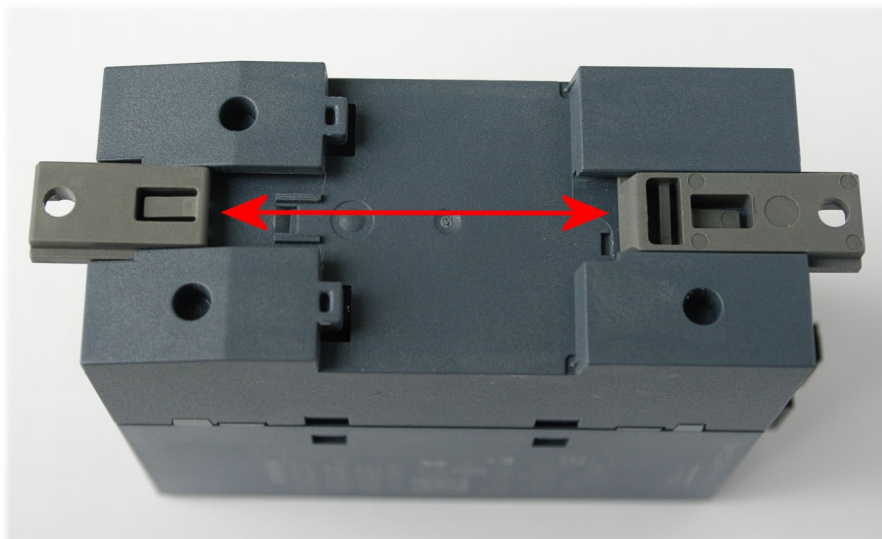
Figure 4-4 Preparation for wall mounting
