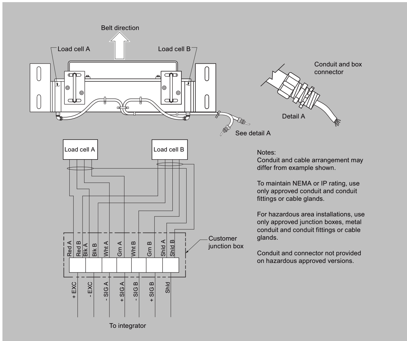
MSI/MMI connections
