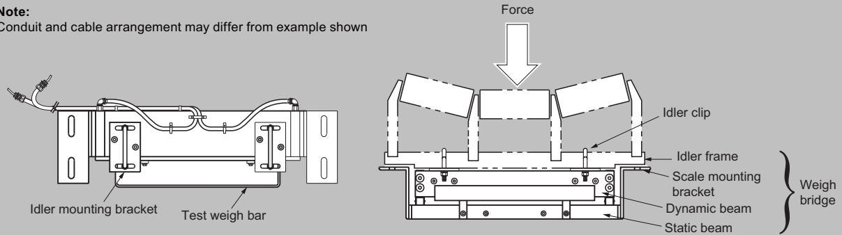
MSI/MMI mounting
