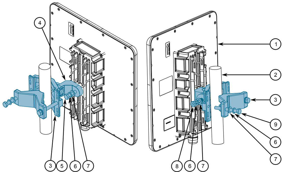
Figure 5: Mounting the Subscriber Unit to a Small Pole
