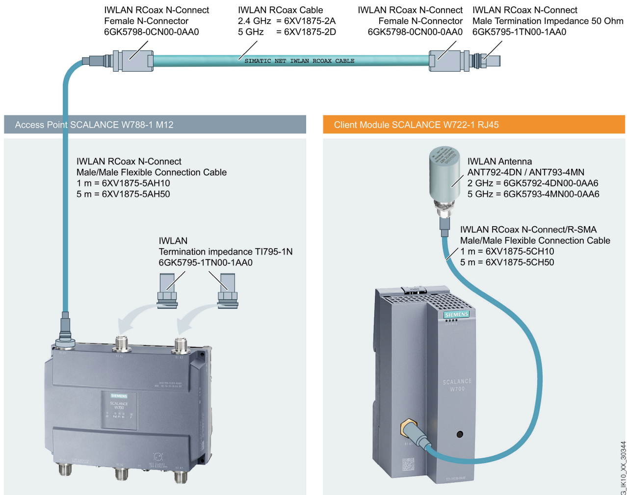
Figure 5-1 SCALANCE W788-1PRO with connected, flexible cable and RCoax connector, beside it an R-SMA terminator 50 \Omega .
