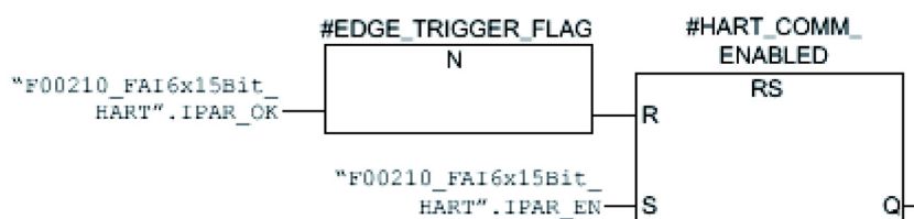
Figure 5-1 Example of enabling HART communication
