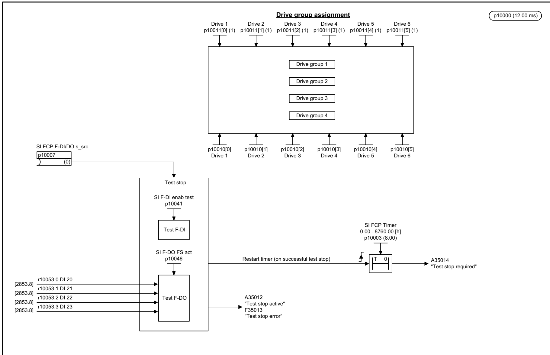
Fig. 2-105 2848 – TM54F configuration, F-DI/F-DO test
