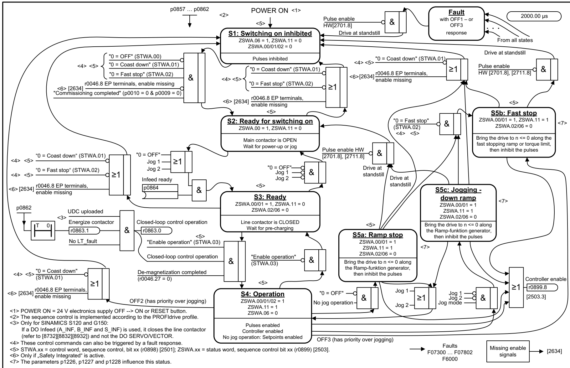
Fig. 2-80 2610 – Sequencer
