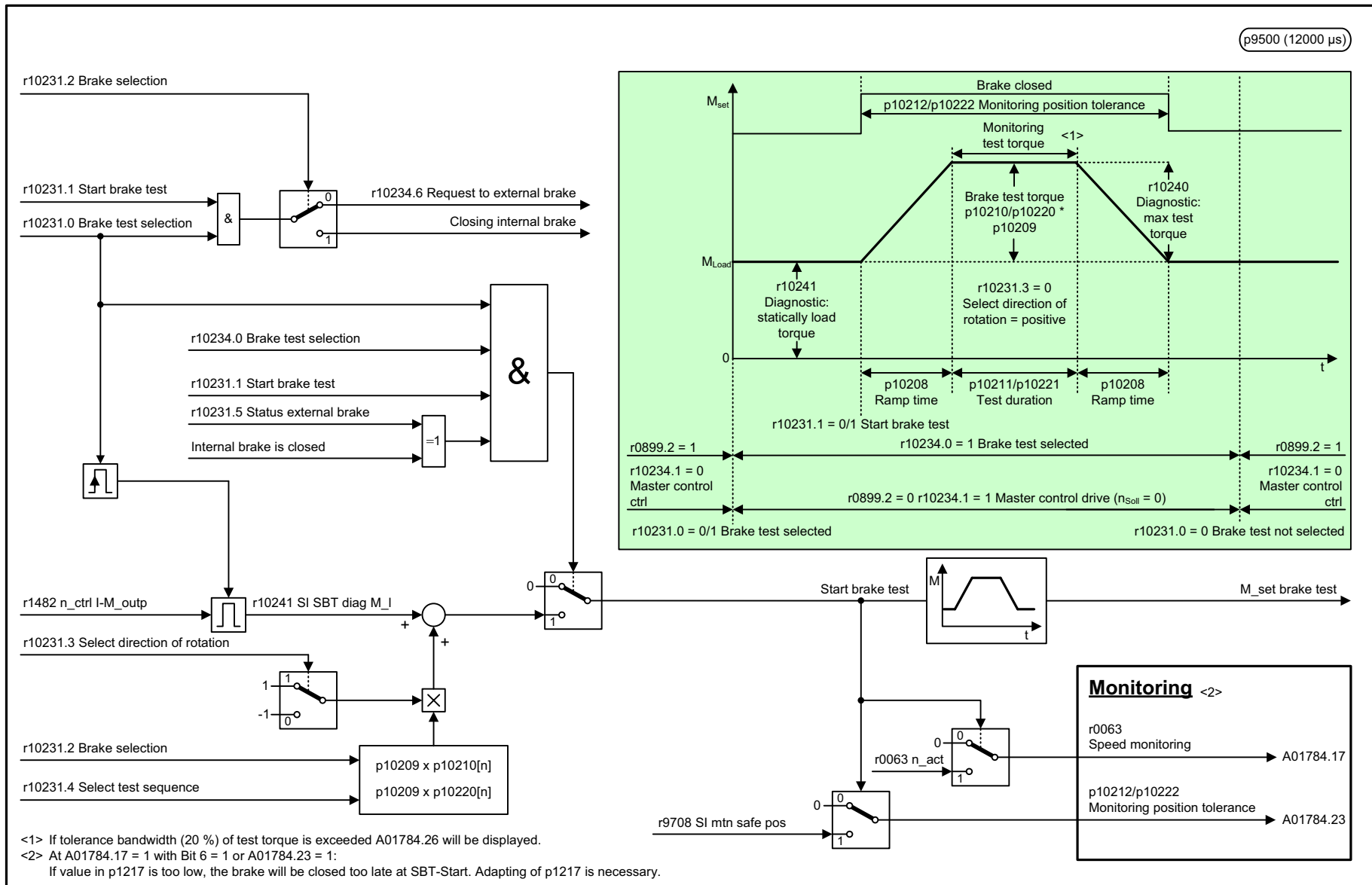
Fig. 2-99 2836 – SBT (Safe Brake Test)
