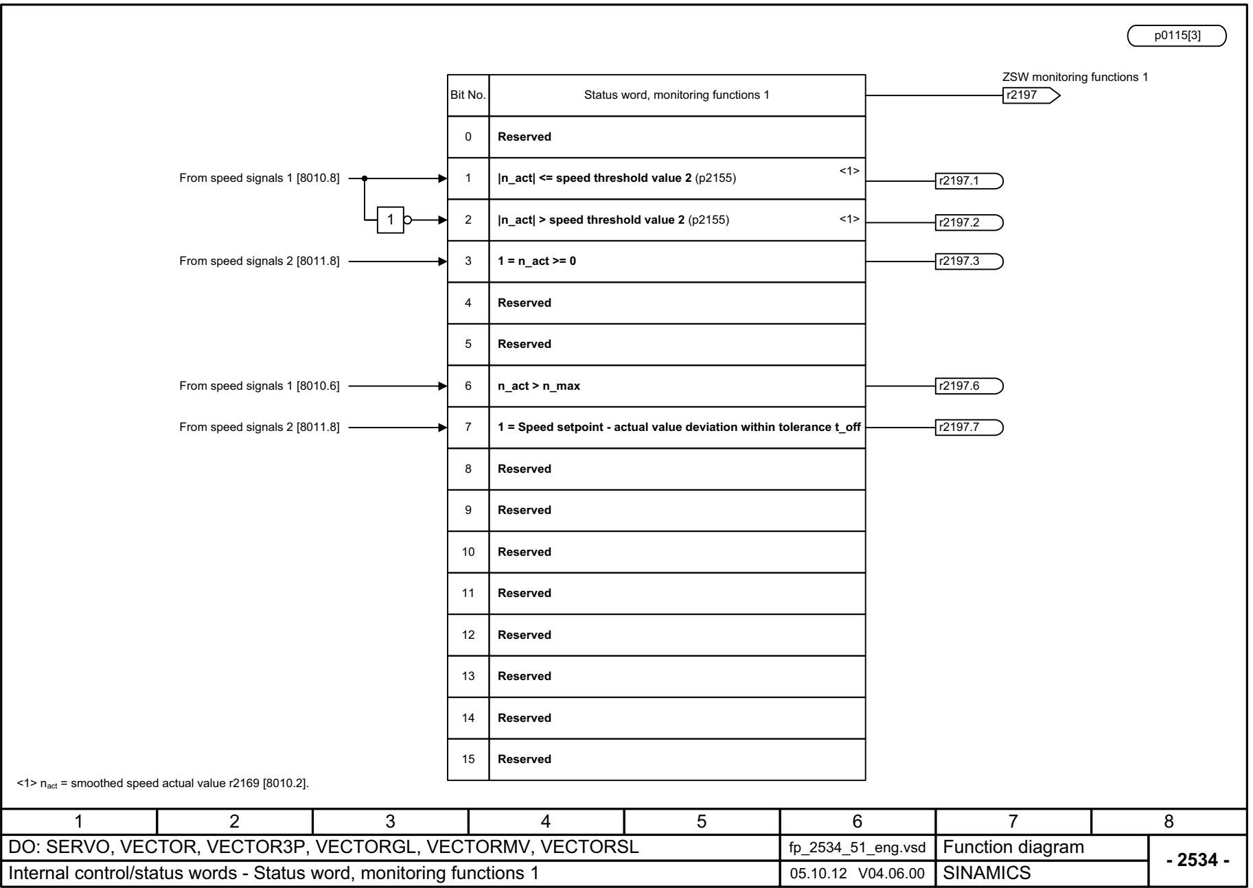
Fig. 2-75 2534 – Status word, monitoring functions 1
