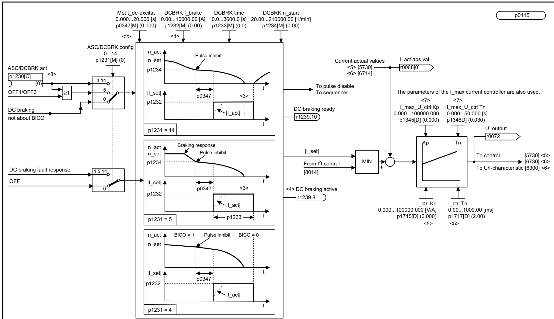
Fig. 2-149 7017 – DC braking (p0300 = 1xx)
