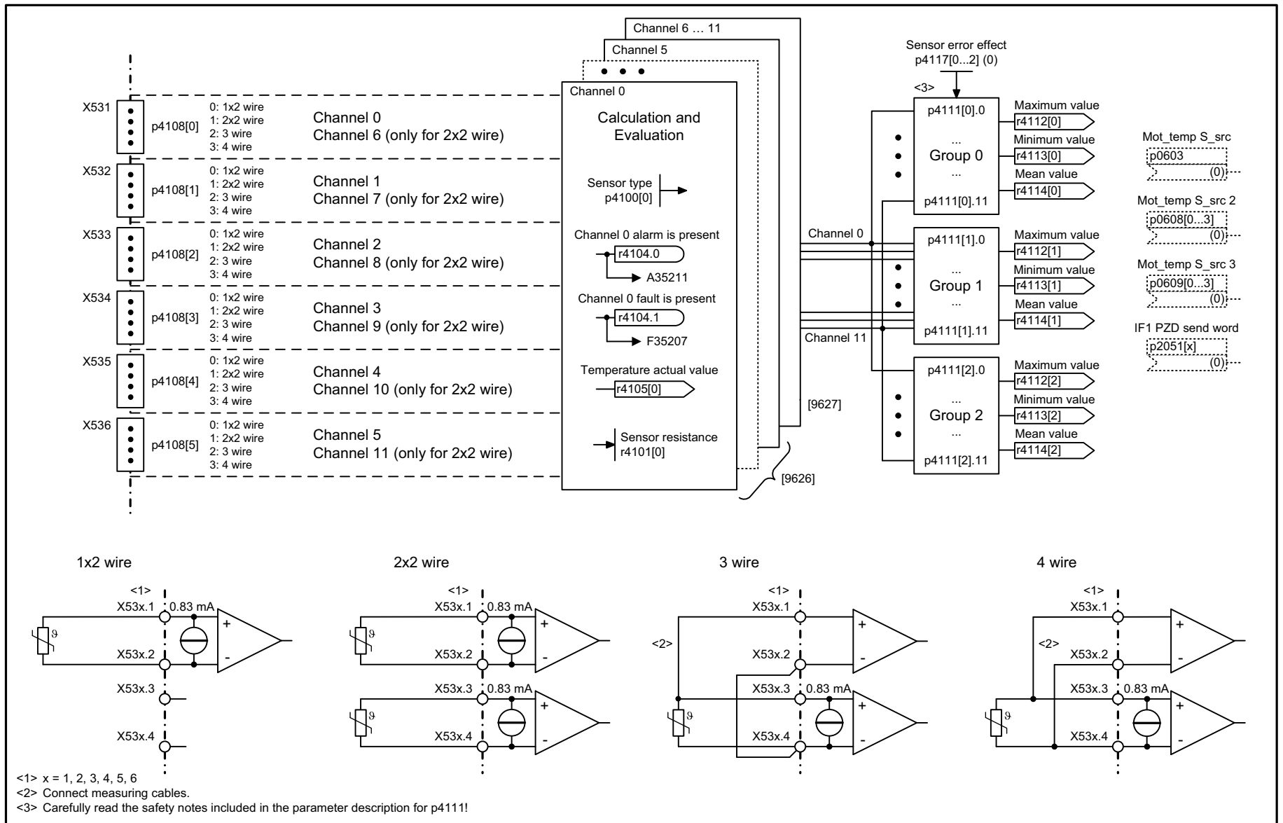
Fig. 2-199 9625 – Temperature evaluation structure (channel 0 ... 11)
