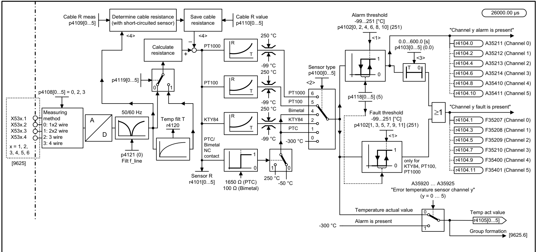
Fig. 2-200 9626 – Temperature evaluation 1x2, 3, 4-wire (channel 0 ... 5)
