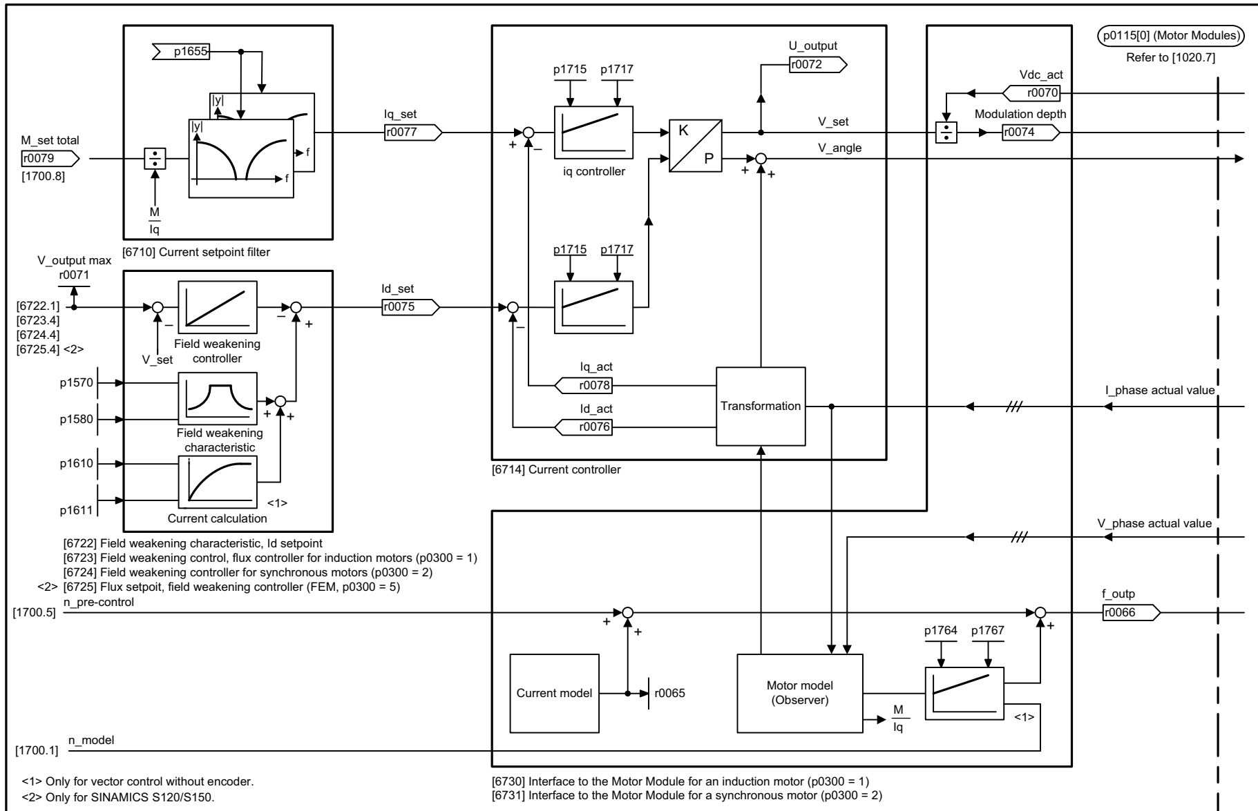
Fig. 2-12 1710 – Vector control, current control
