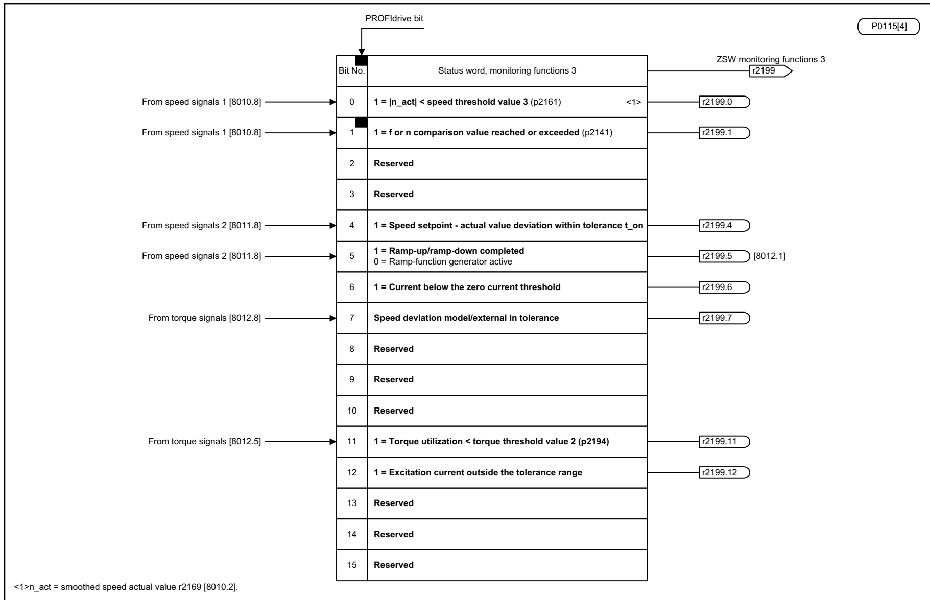
Fig. 2-77 2537 – Status word, monitoring functions 3
