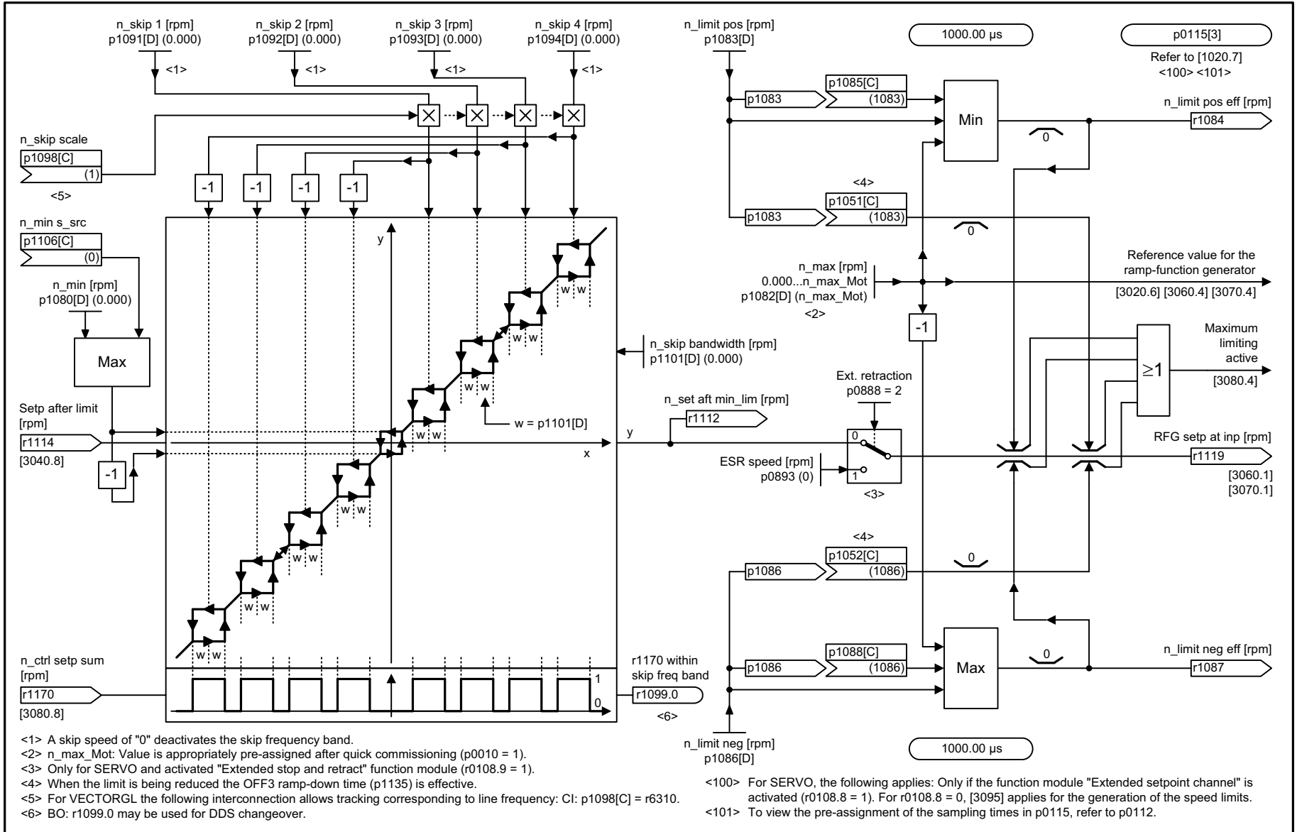
Fig. 2-118 3050 – Skip frequency bands and speed limitations
