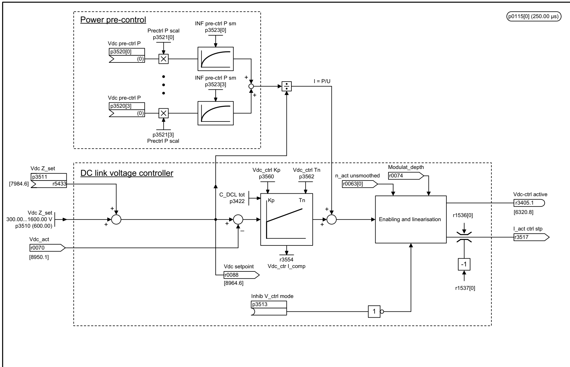
Fig. 2-156 7960 – DC-link voltage controller (r0108.16 = 1)
