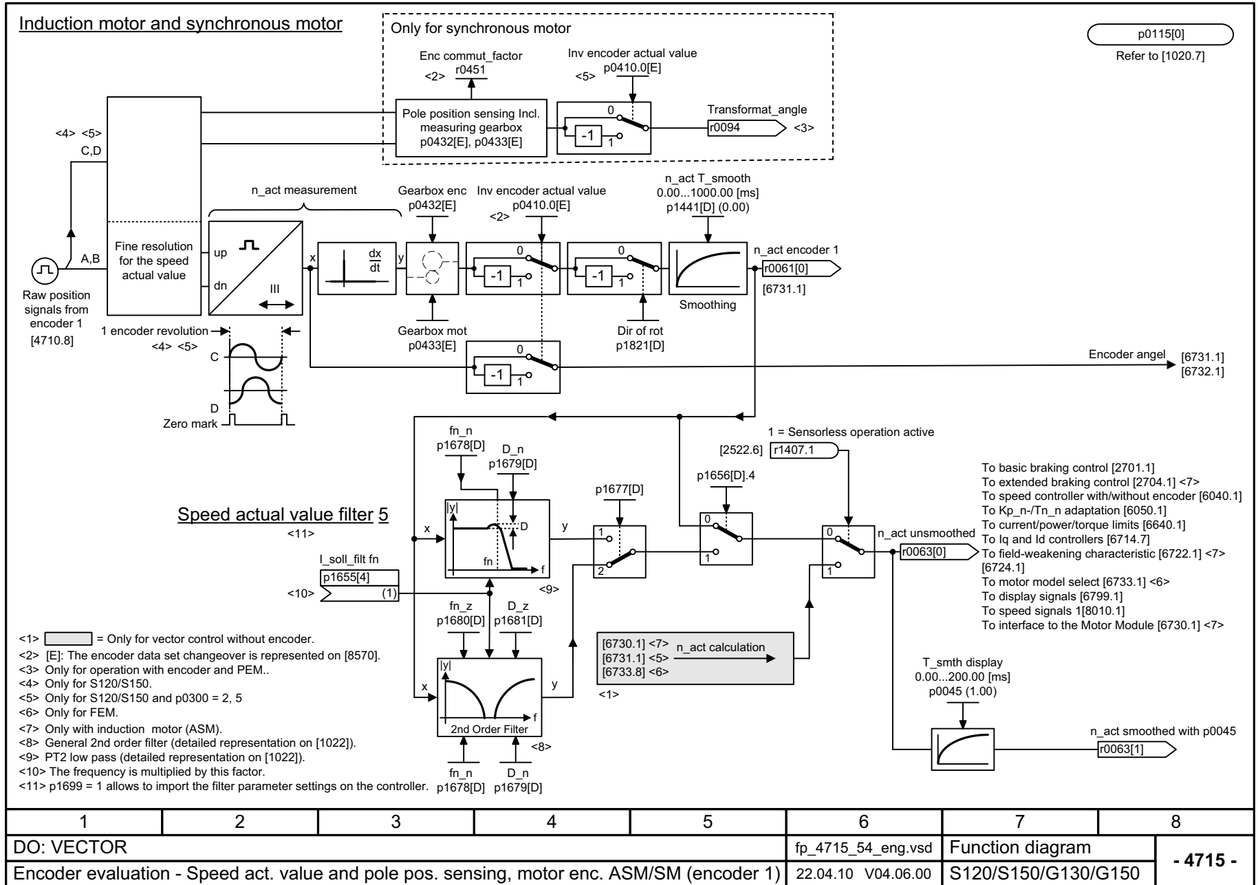
Fig. 2-123 4715 – Actual speed value and pole position sensing, motor encoder ASM/SM (encoder 1)
