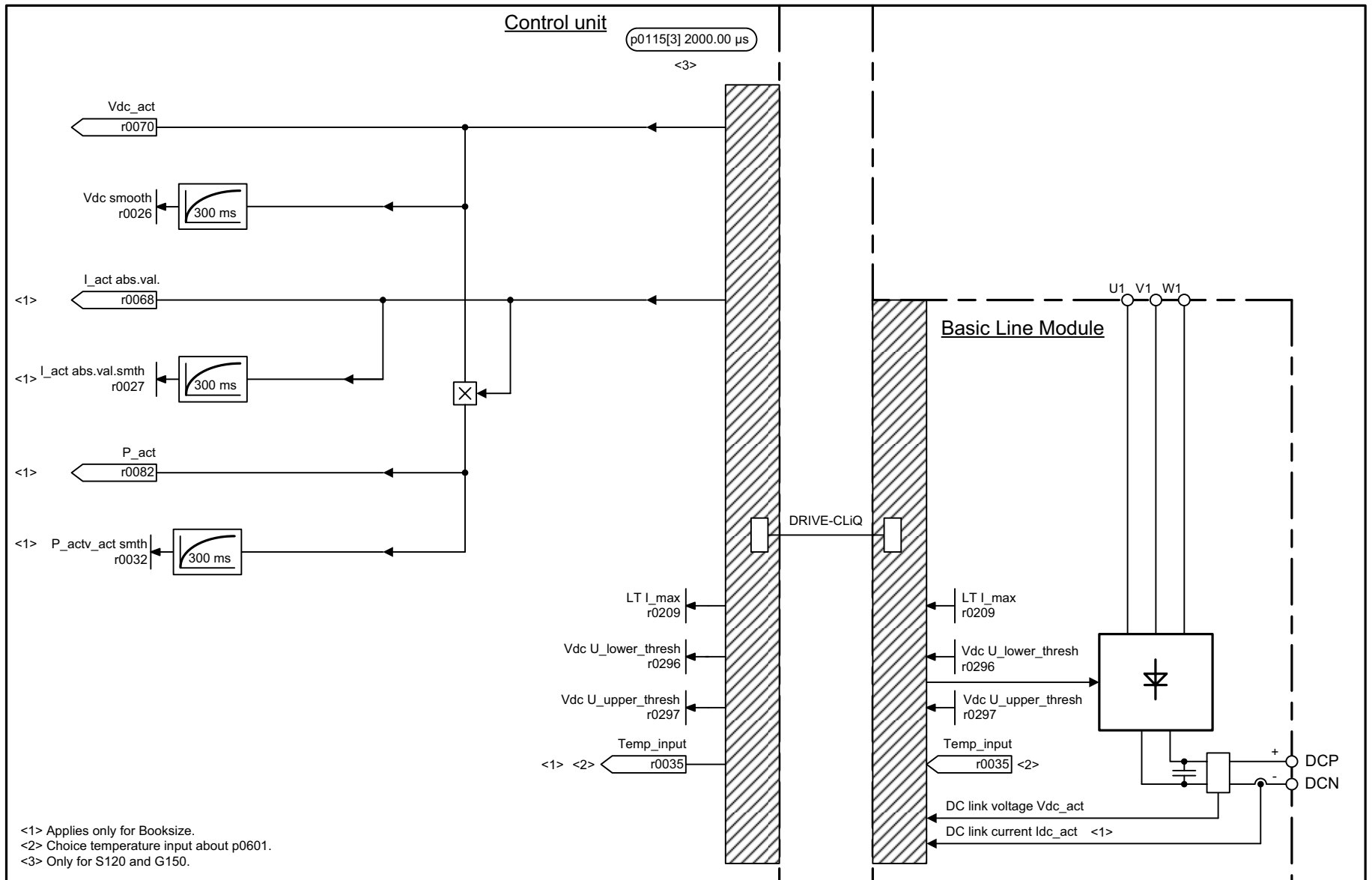
Fig. 2-178 8750 – Interface to the Basic Infeed power unit (control signals, actual values)
