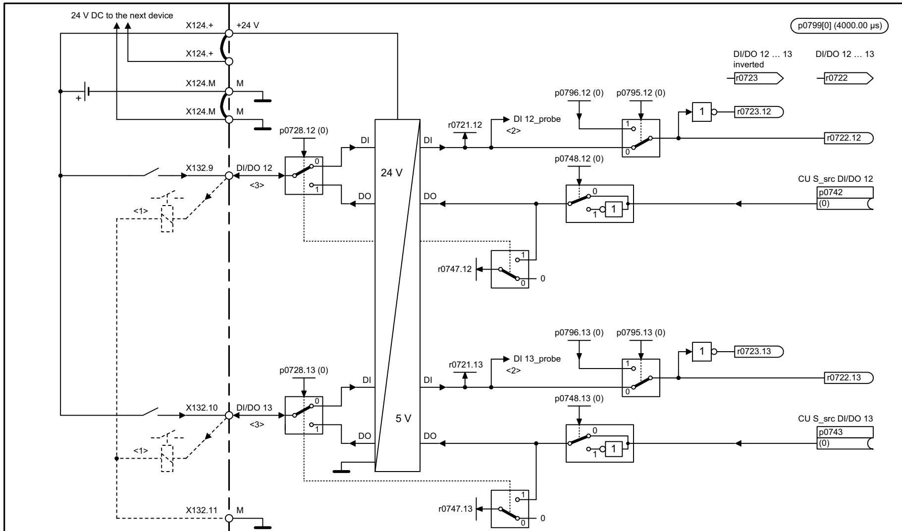
Fig. 2-22 2132 – Digital inputs/outputs, bidirectional (DI/DO 12 ... DI/DO 13)
