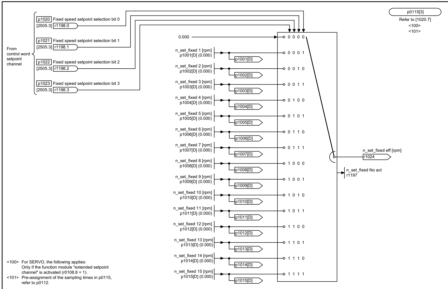
Fig. 2-114 3010 – Fixed speed setpoints
