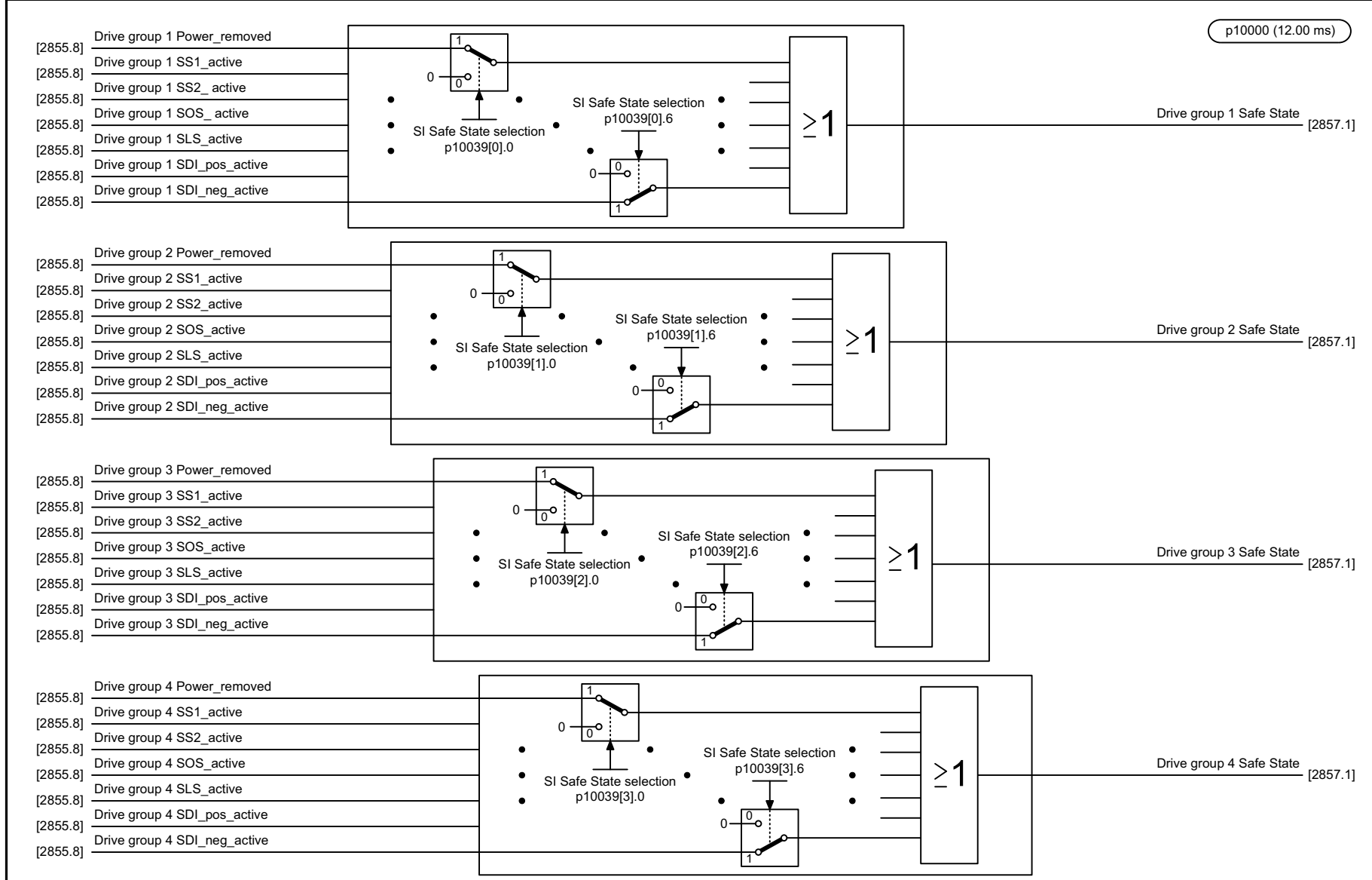
Fig. 2-110 2856 – TM54F Safe State selection
