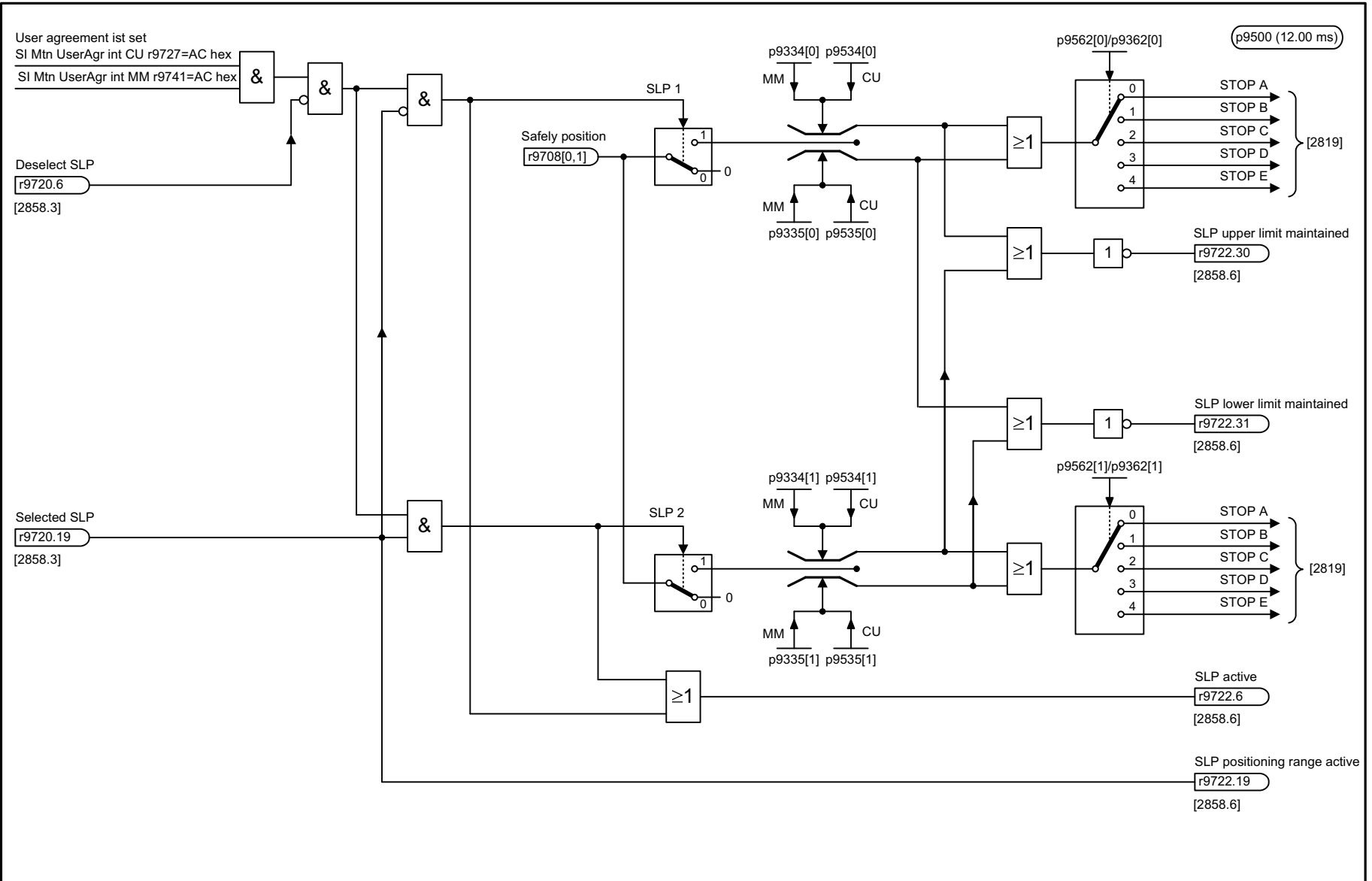
Fig. 2-96 2822 – SLP (Safely-Limited Position)
