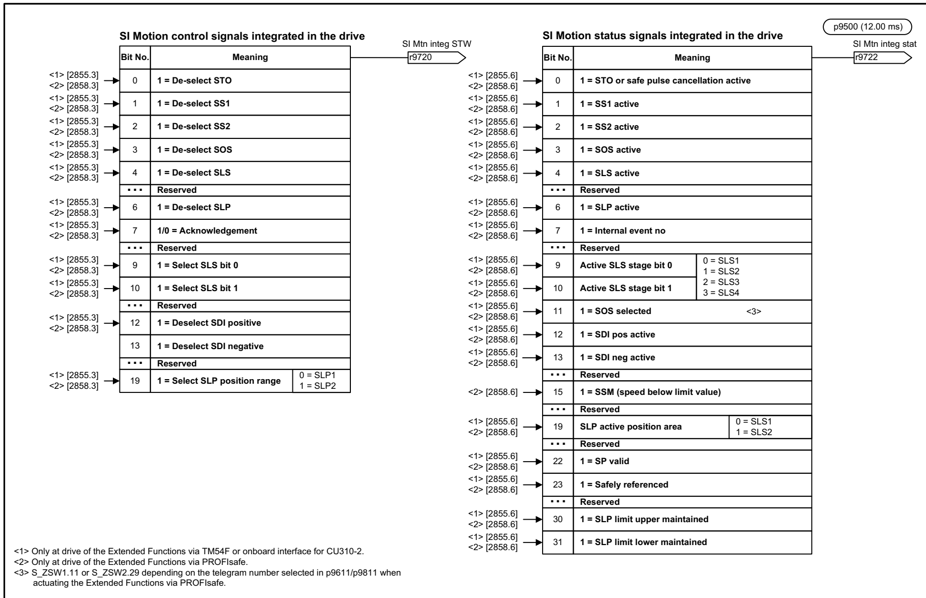
Fig. 2-101 2840 –SI Motion drive-integrated control signals/status signals
