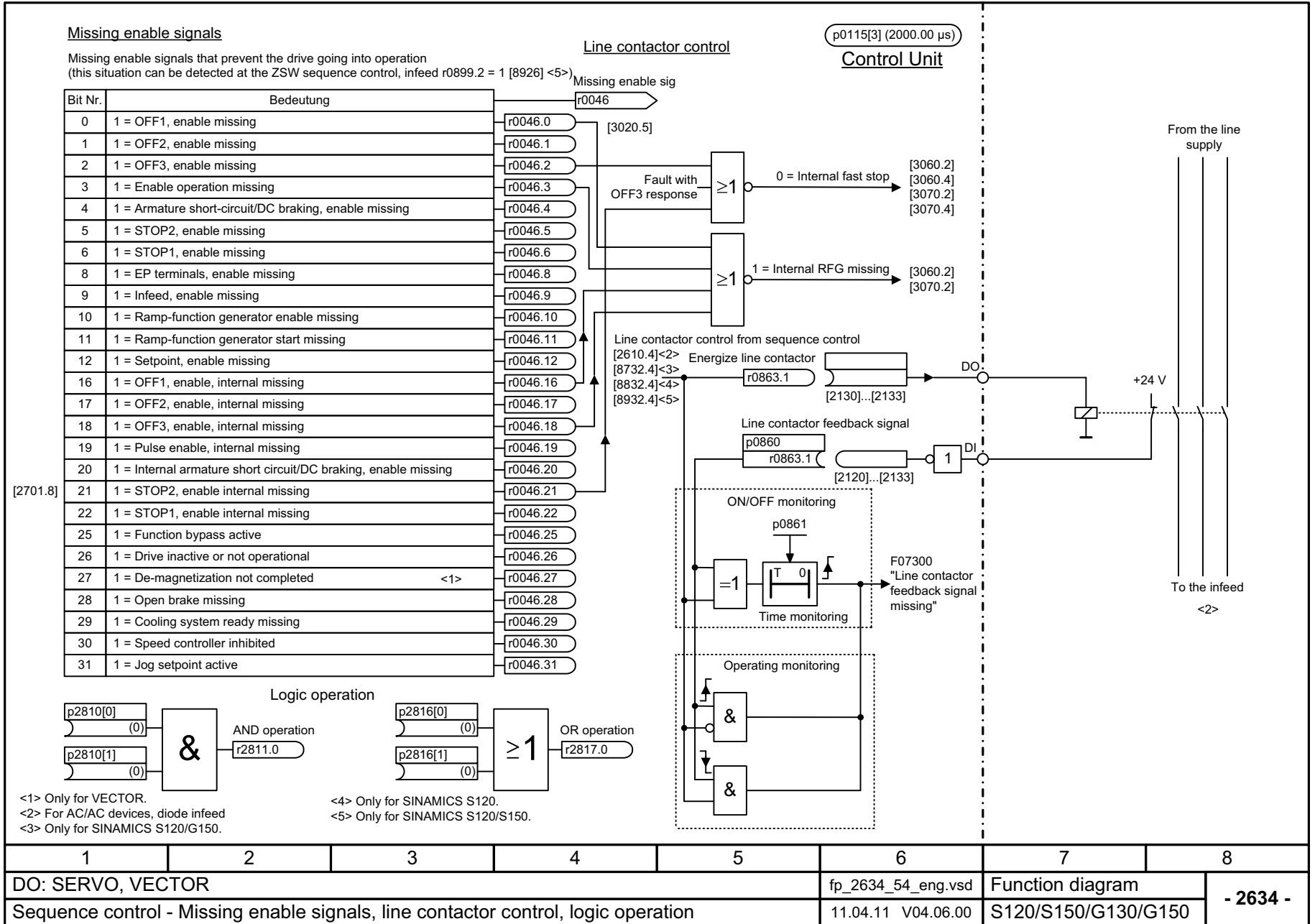
Fig. 2-81 2634 – Missing enable signals, line contactor control, logic operation
