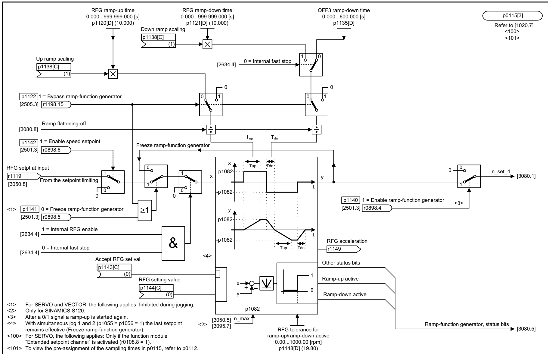
Fig. 2-119 3060 – Basic ramp-function generator
