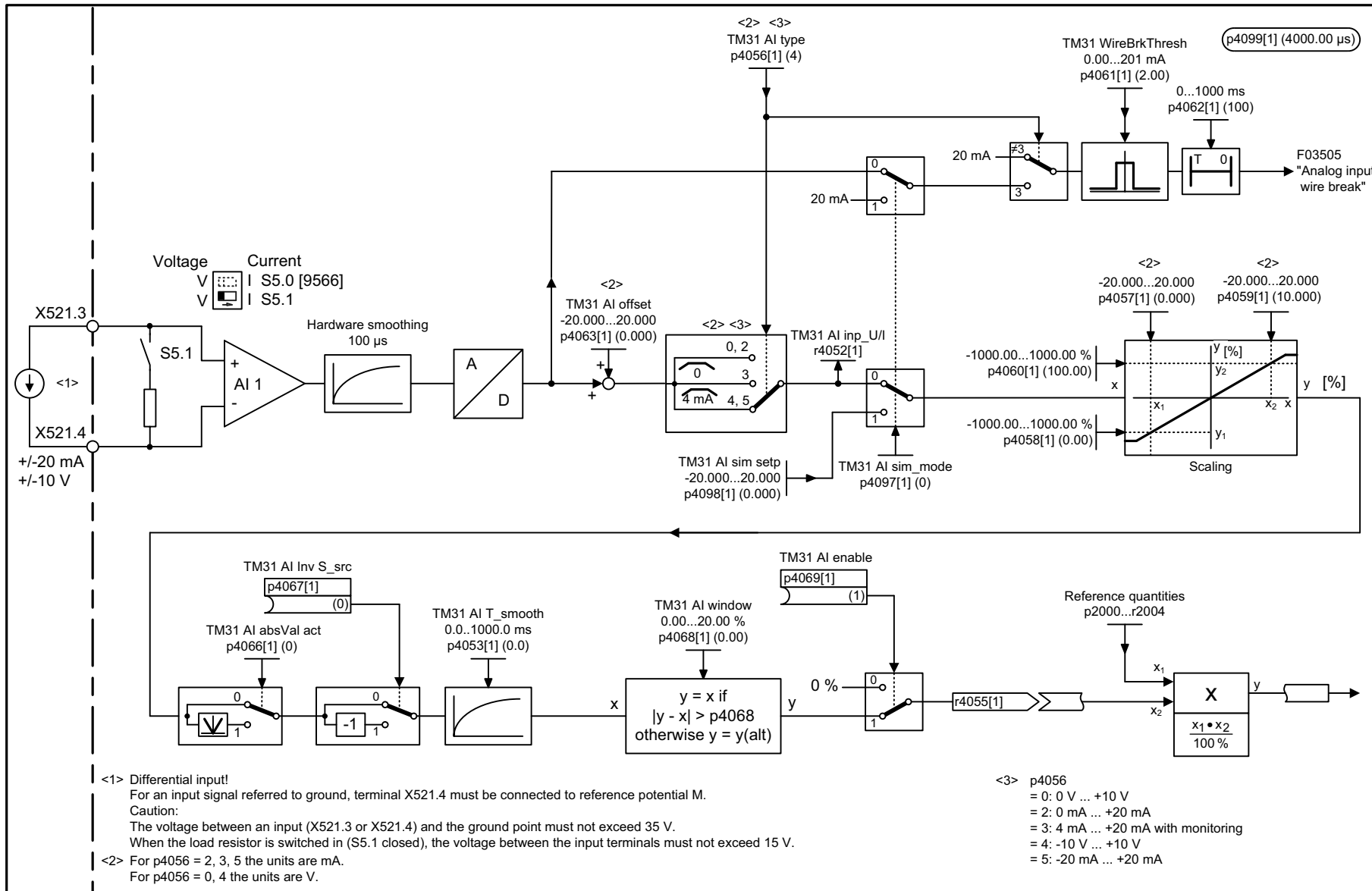
Fig. 2-196 9568 – Analog input 1 (AI 1)
