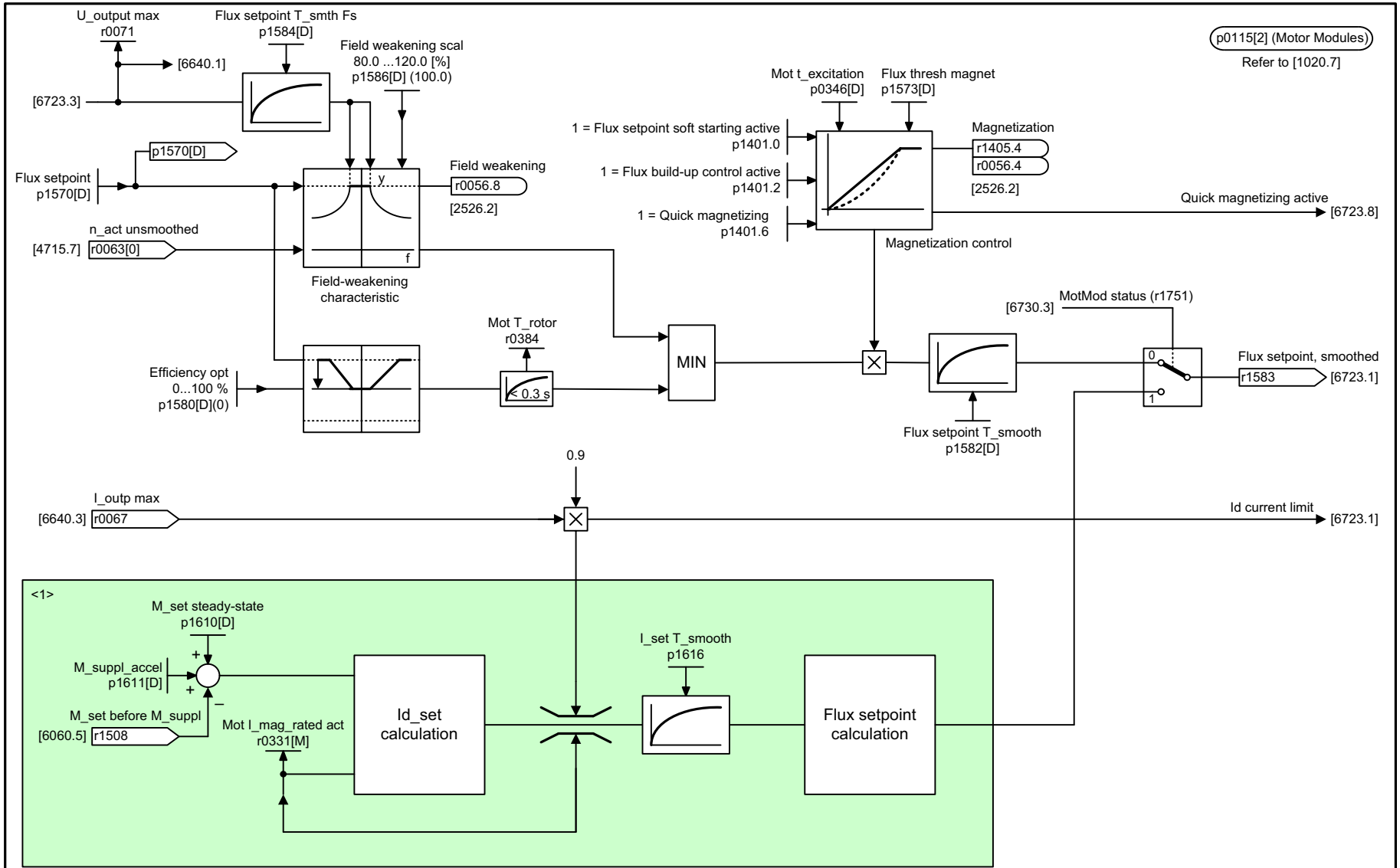
Fig. 2-140 6722 – Field weakening characteristic, Id setpoint (ASM, p0300 = 1)
