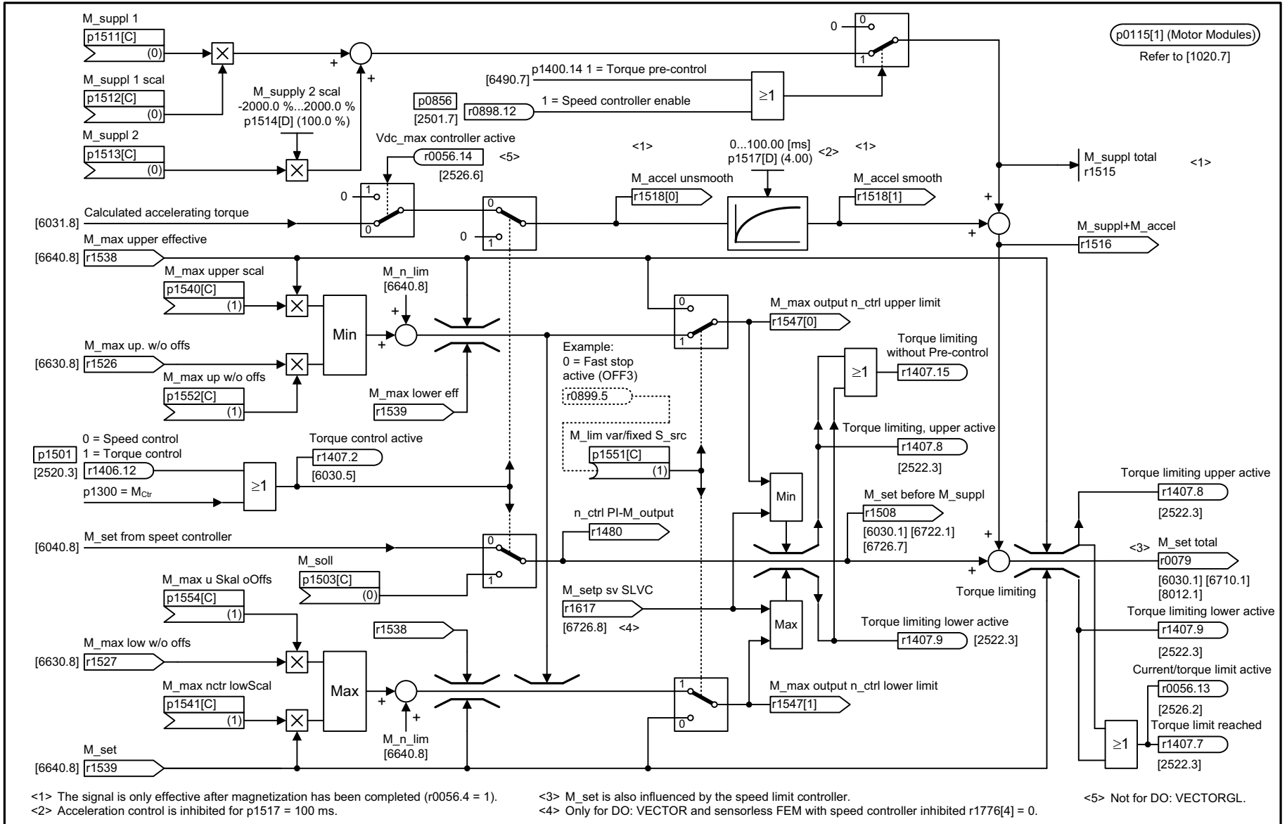
Fig. 2-128 6060 – Torque setpoint
