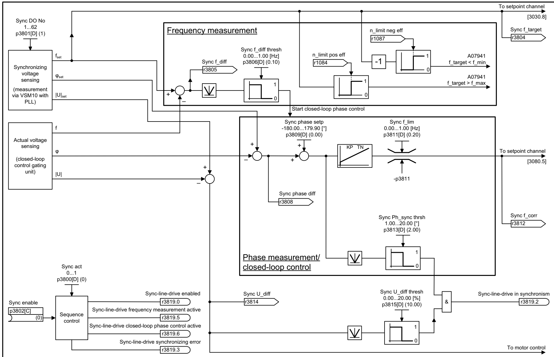
Fig. 2-150 7020 – Synchronization
