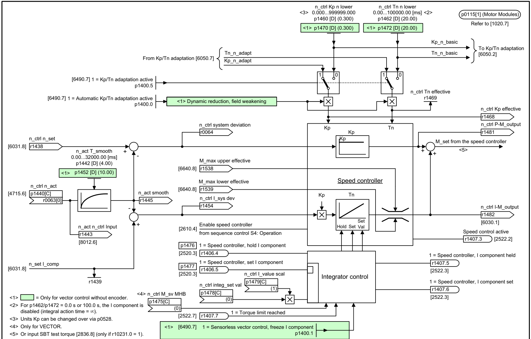
Fig. 2-126 6040 – Speed controller with/without encoder
