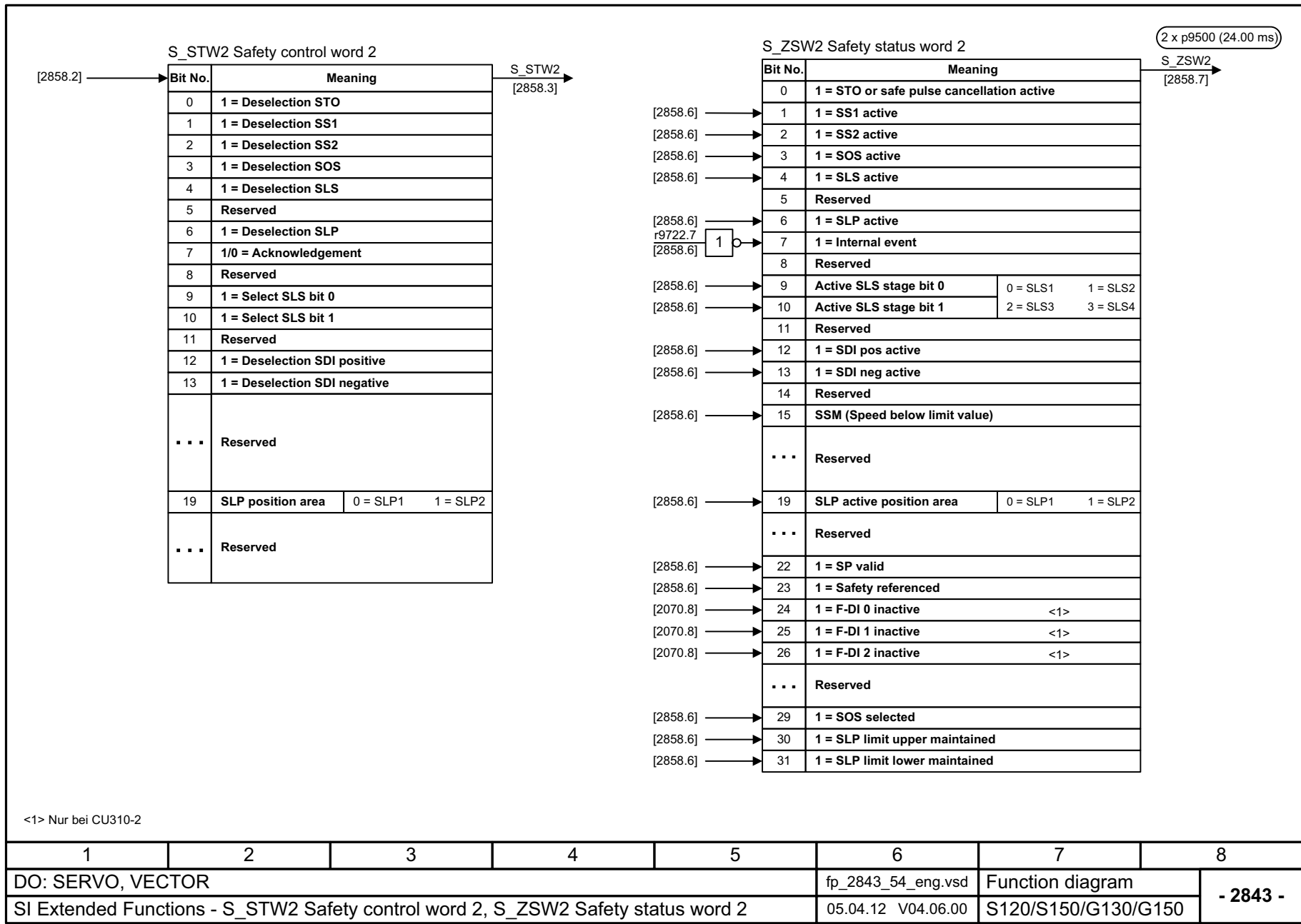
Fig. 2-103 2843 – S_STW2 Safety control word 2, S_ZSW2 Safety status word 2
