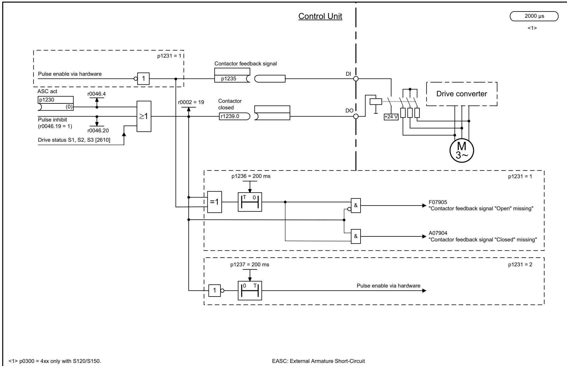
Fig. 2-147 7014 – External Armature Short-Circuit (EASC, p0300 = 2xx or 4xx)
