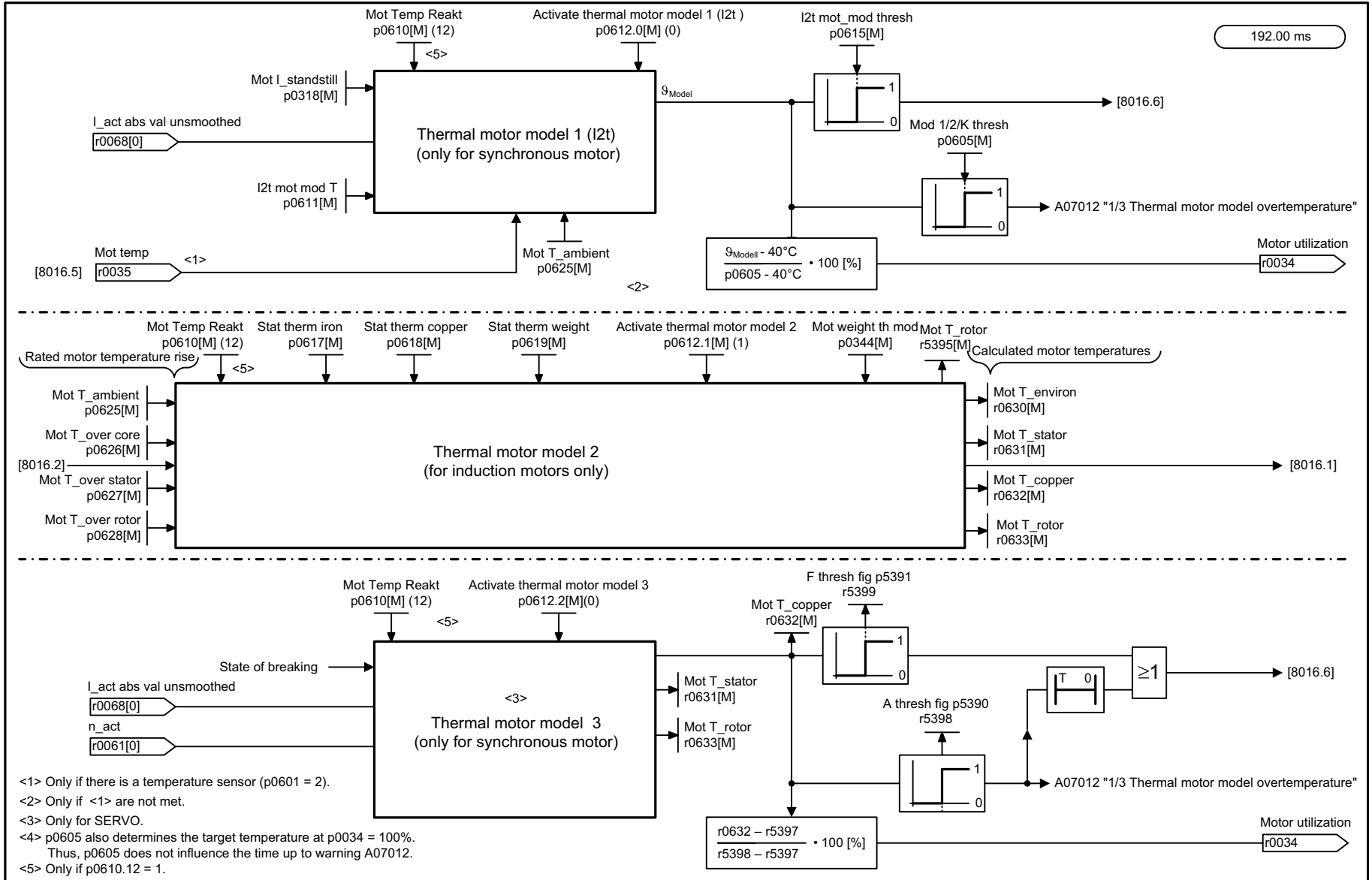
Fig. 2-163 8017 – Thermal motor models
