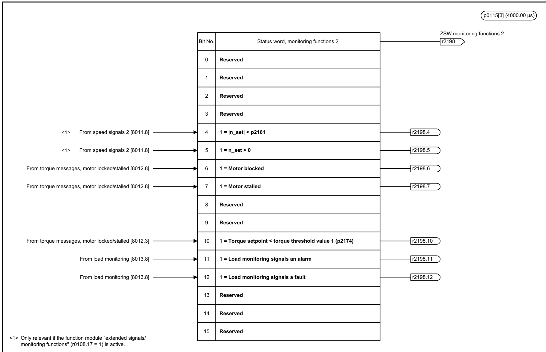
Fig. 2-76 2536 – Status word, monitoring functions 2
