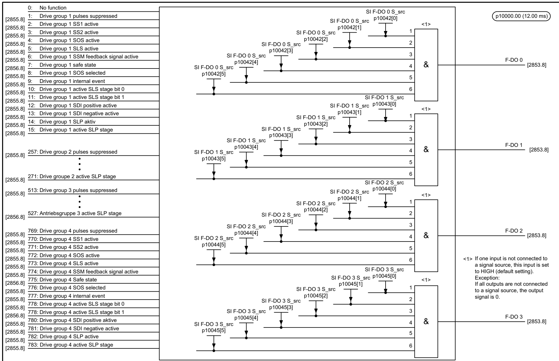
Fig. 2-111 2857 – TM54F assignment (F-DO 0 ... F-DO 3)
