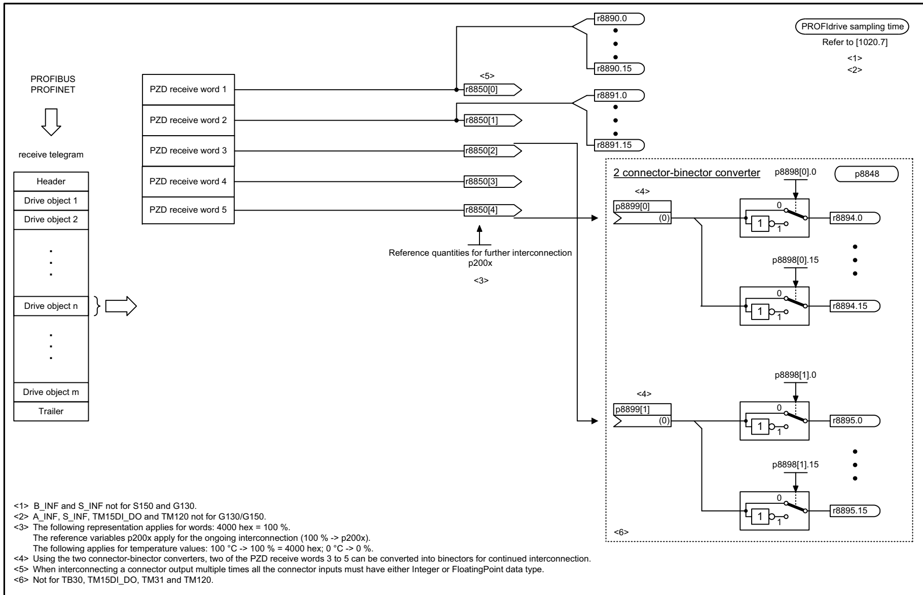
Fig. 2-60 2491 – IF2 receive telegram, free interconnection
