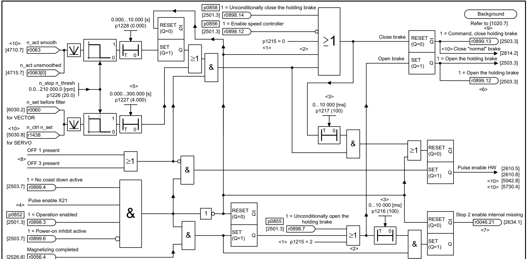
Fig. 2-82 2701 – Basic brake control (r0108.14 = 0)
