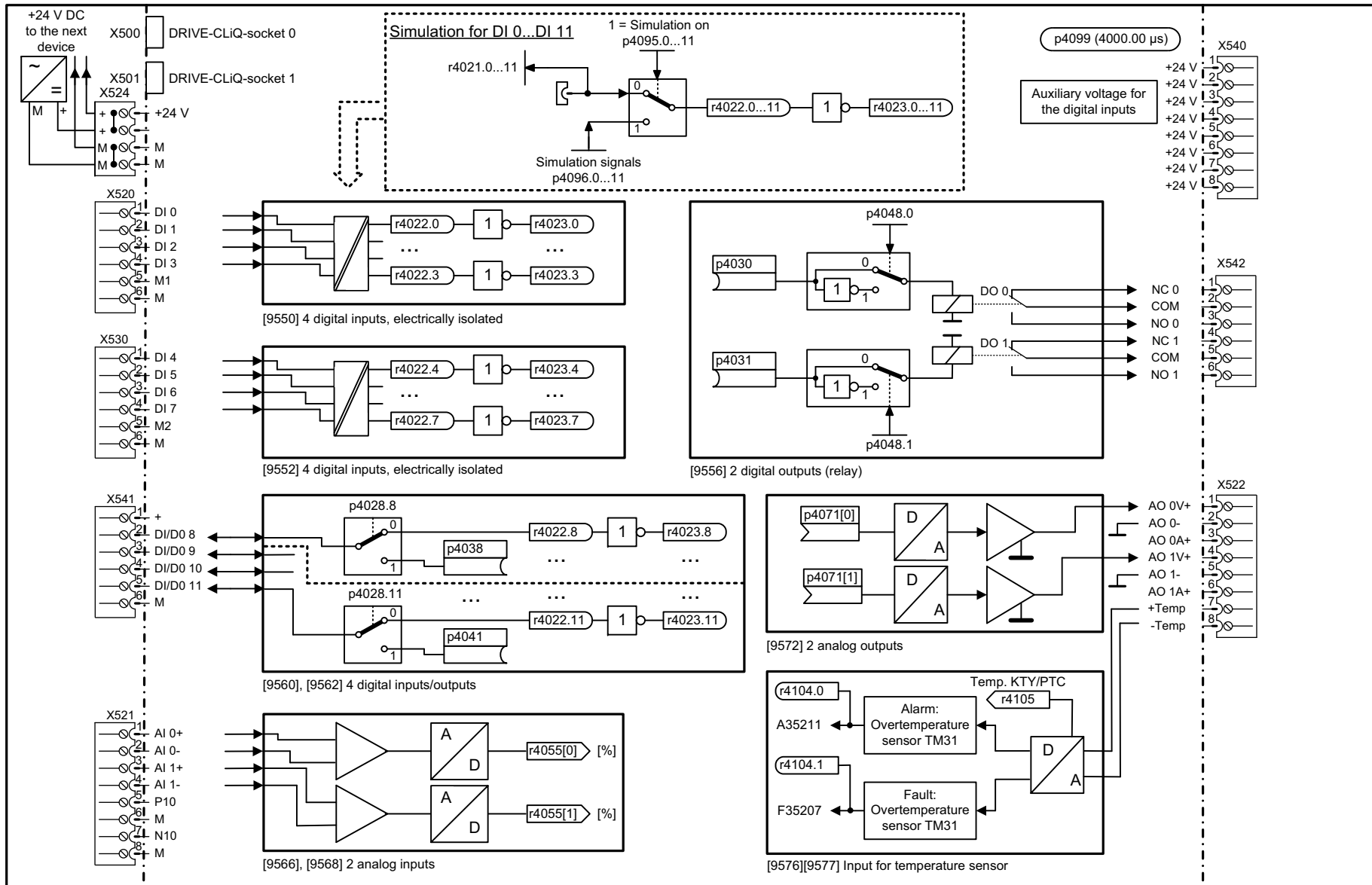
Fig. 2-16 1840 – Terminal Module 31 (TM31)
