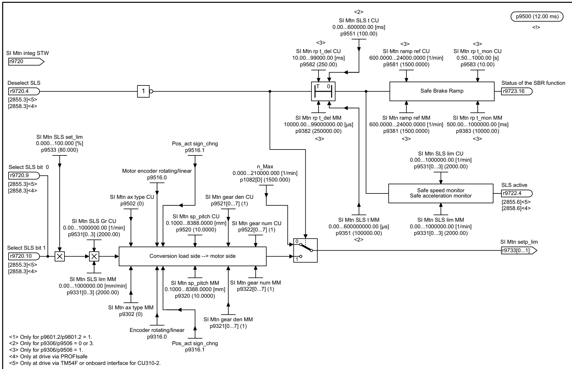
Fig. 2-95 2820 – SLS (Safely-Limited Speed)
