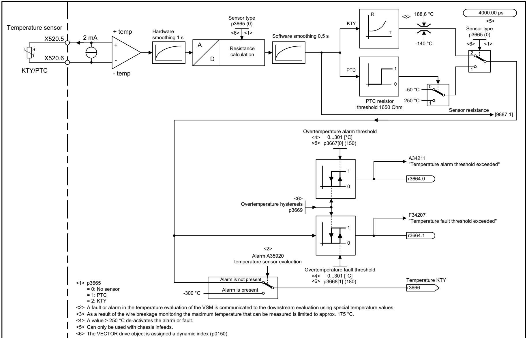
Fig. 2-203 9886 – Temperature evaluation
