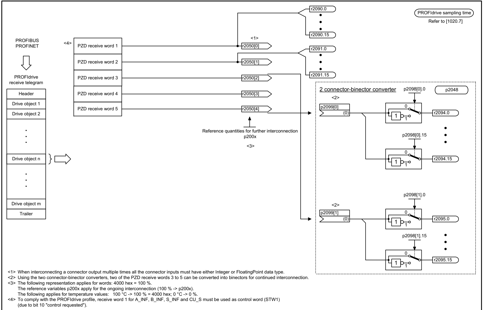
Fig. 2-55 2481 – IF1 receive telegram, free interconnection via BICO (p0922 = 999)
