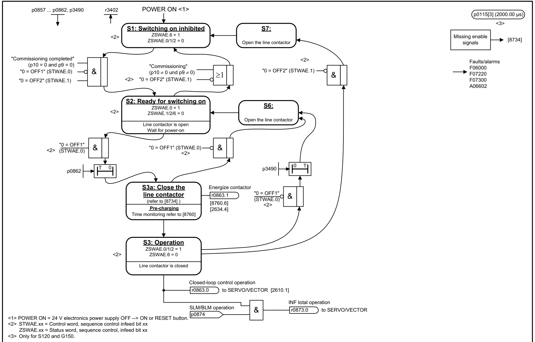
Fig. 2-176 8732 – Sequencer
