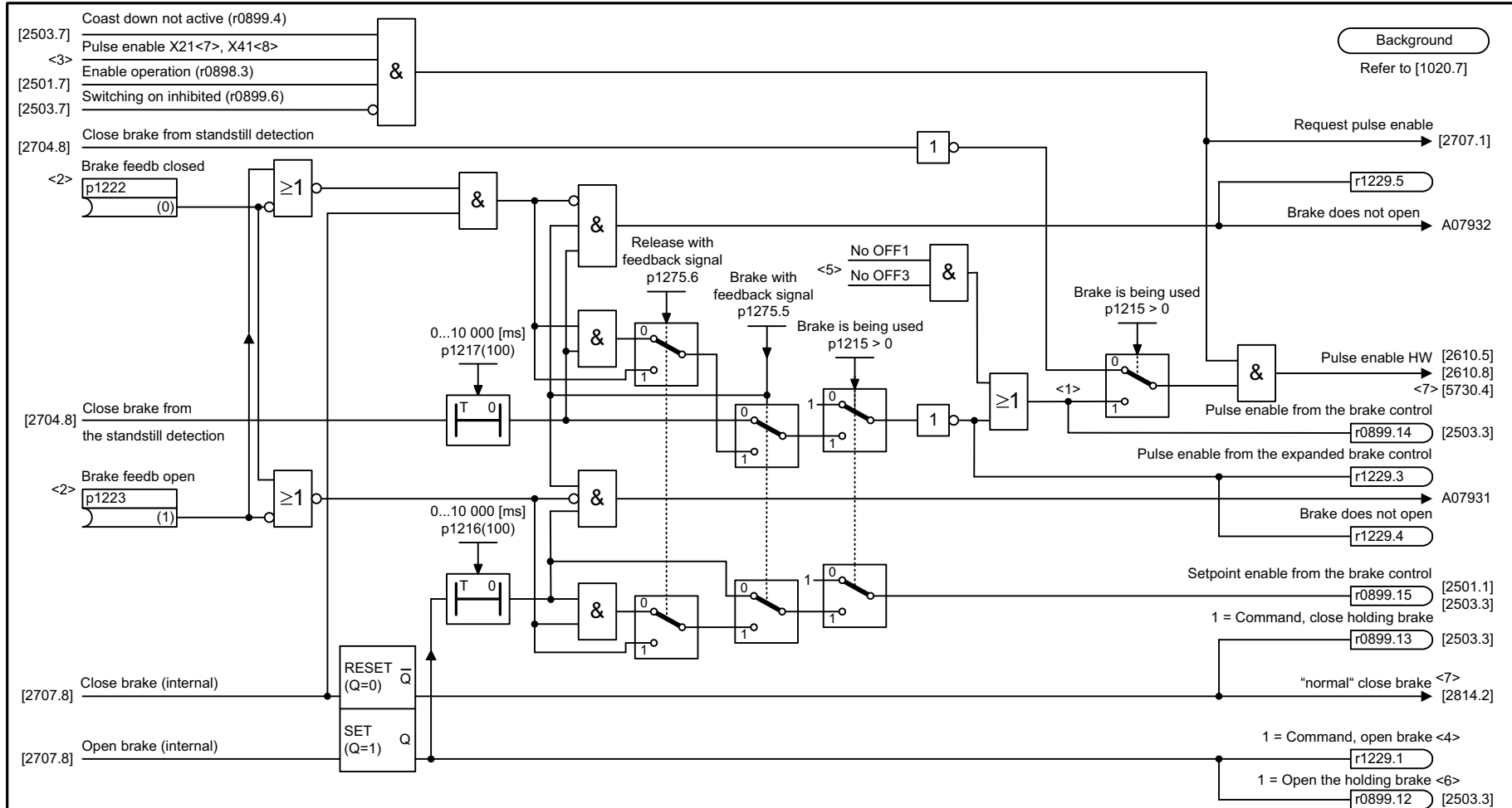
Fig. 2-85 2711 – Extended brake control, signal outputs (r0108.14 = 1)
