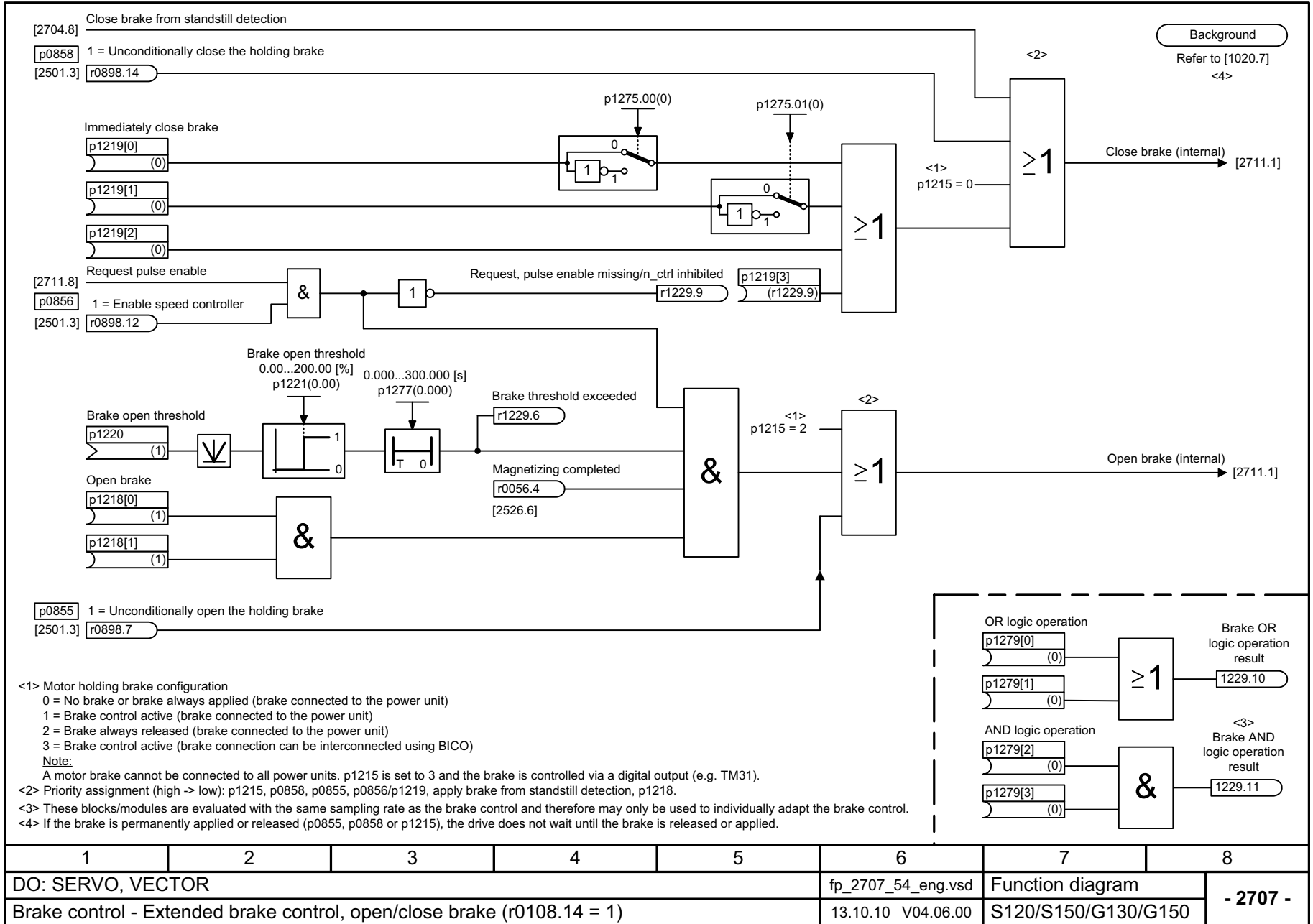
Fig. 2-84 2707 – Extended brake control, open/close brake (r0108.14 = 1)
