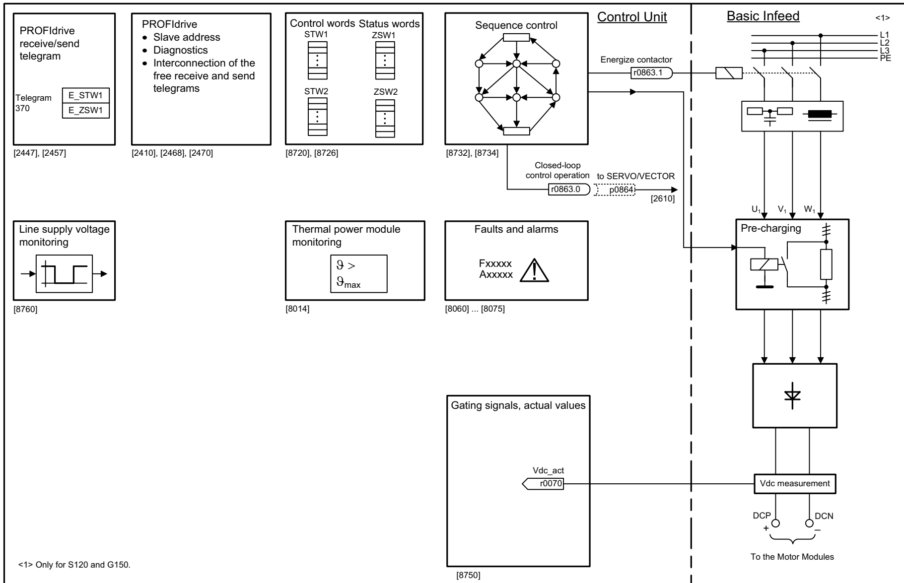
Fig. 2-14 1773 – Basic Infeed
