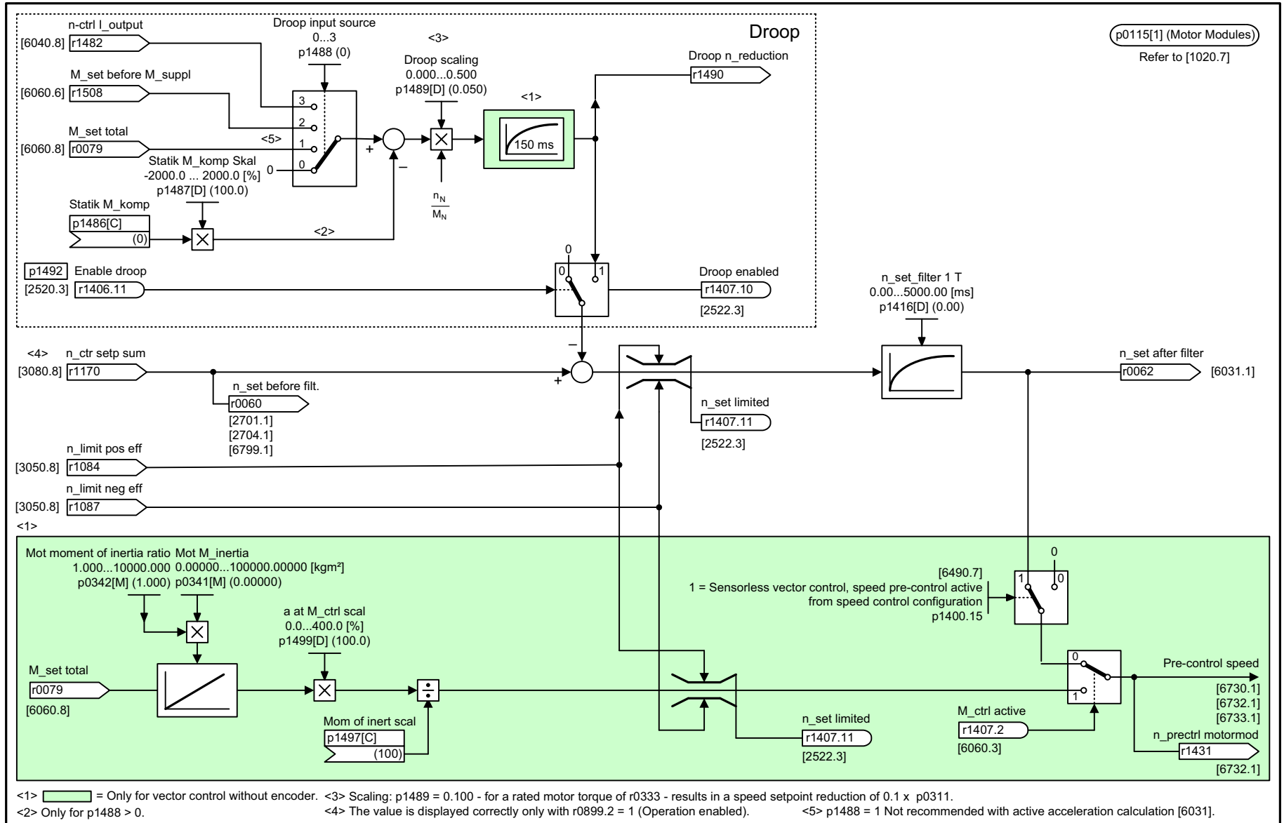
Fig. 2-124 6030 – Speed setpoint, droop
