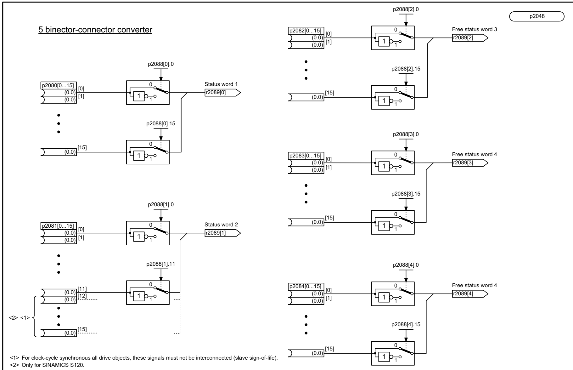
Fig. 2-54 2472 – IF1 status words, free interconnection
