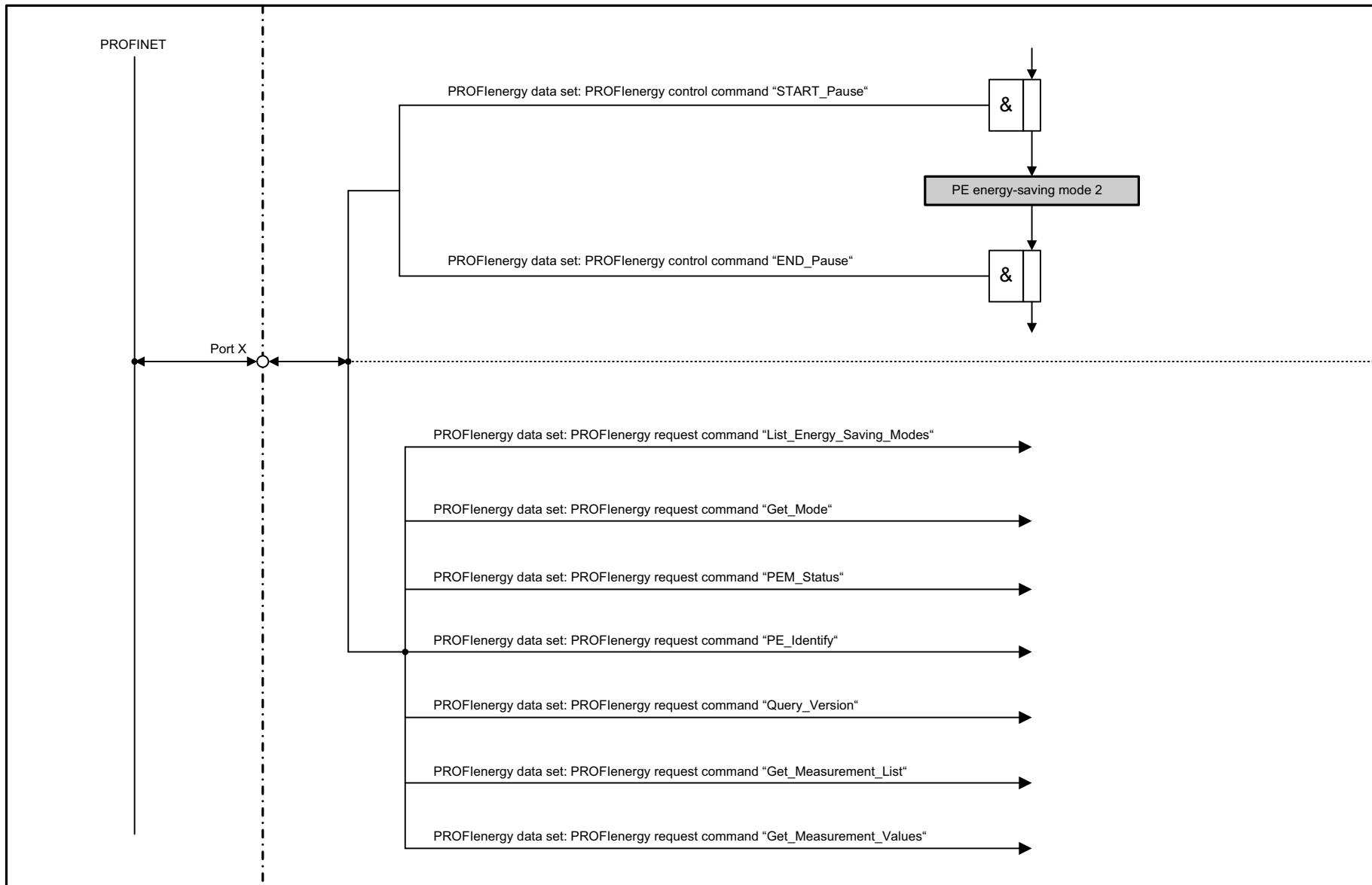
Fig. 2-24 2381 – Control commands / interrogation commands
