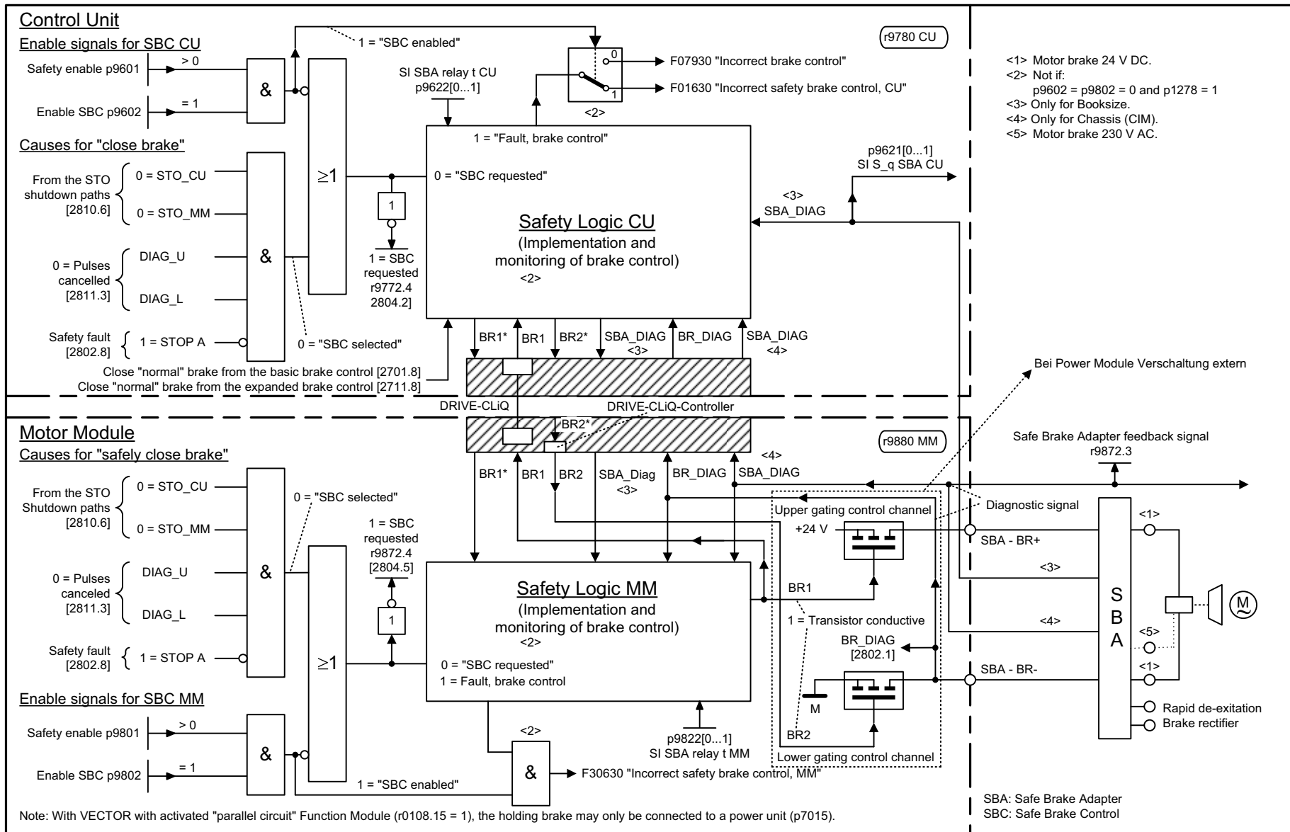
Fig. 2-92 2814 – SBC (Safe Brake Control), SBA (Safe Brake Adapter)
