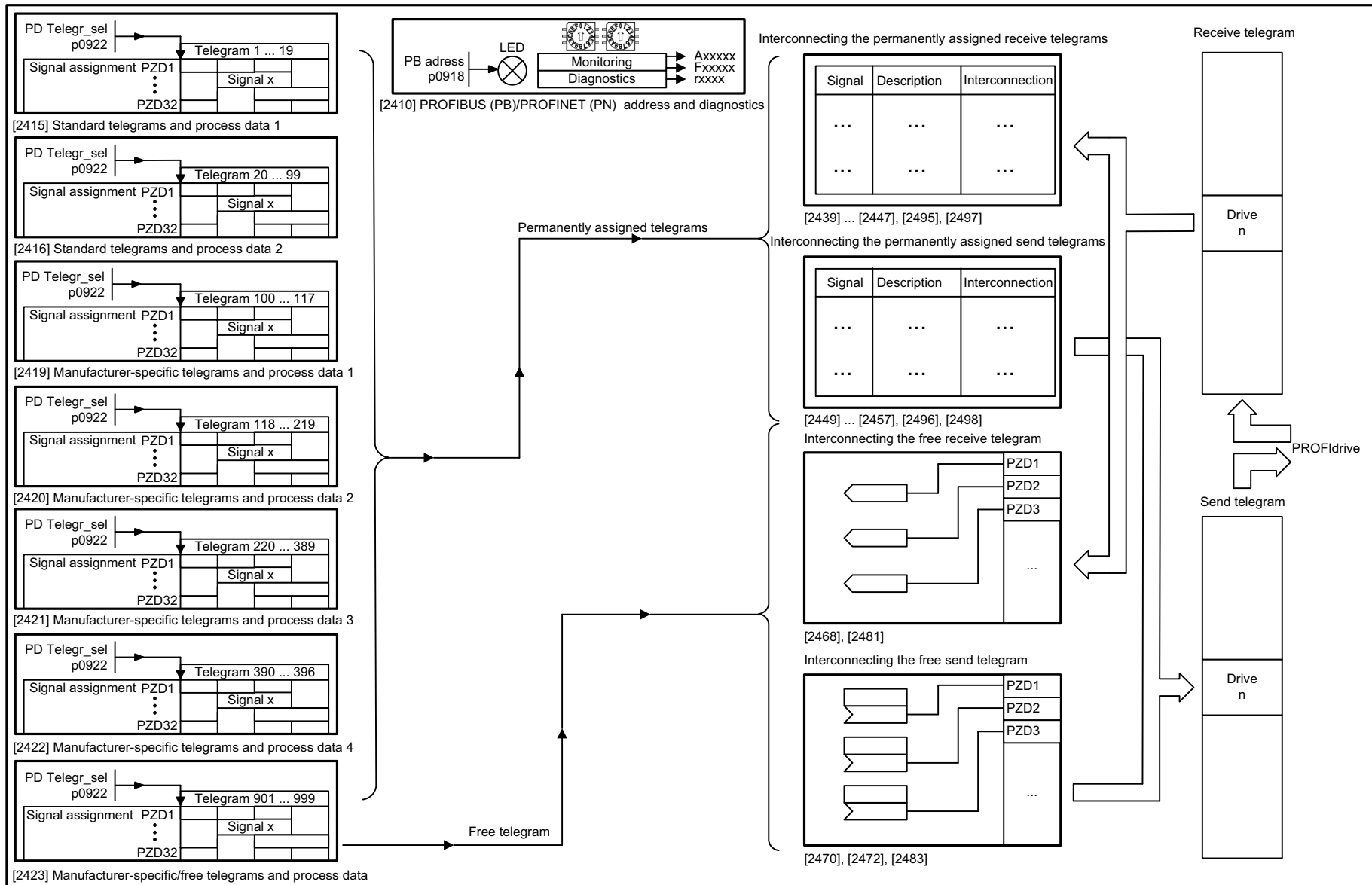
Fig. 2-6 1520 – PROFIdrive
