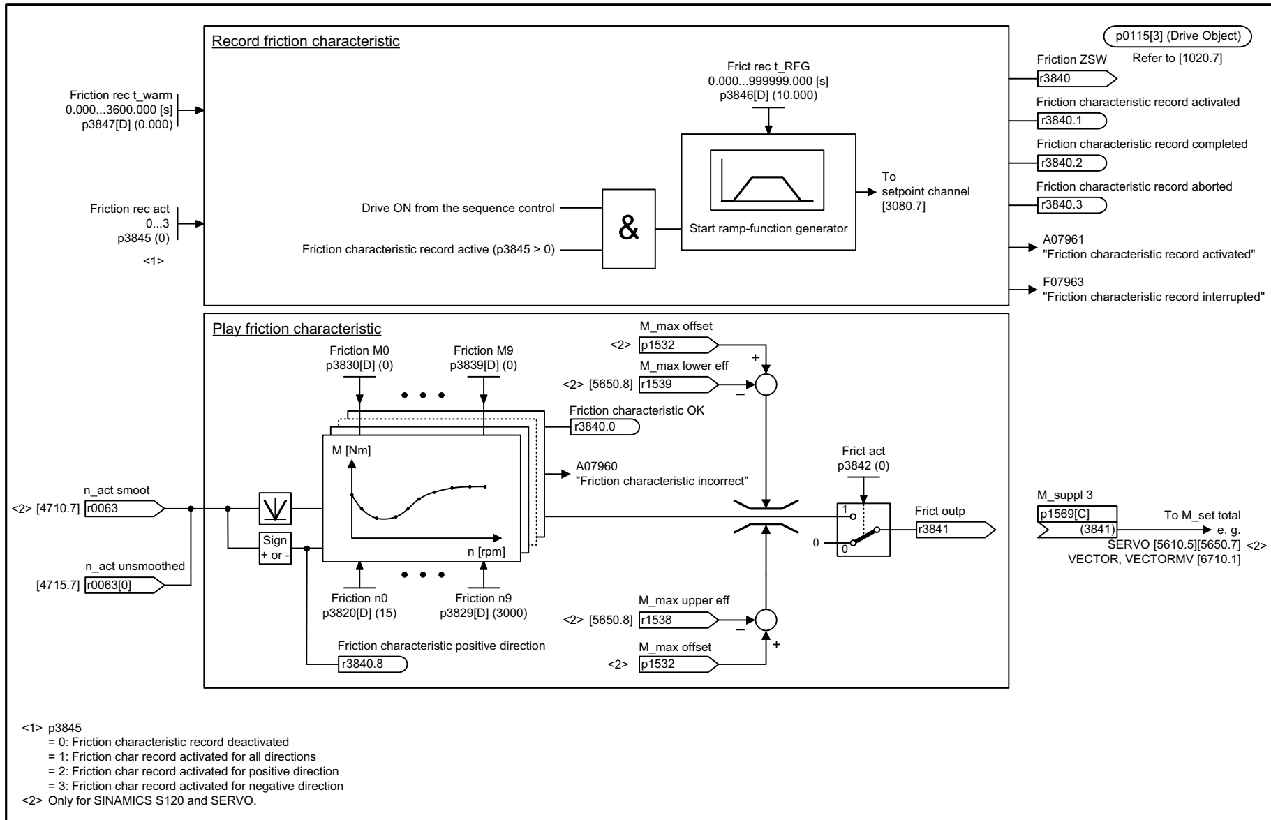
Fig. 2-146 7010 – Friction characteristic
