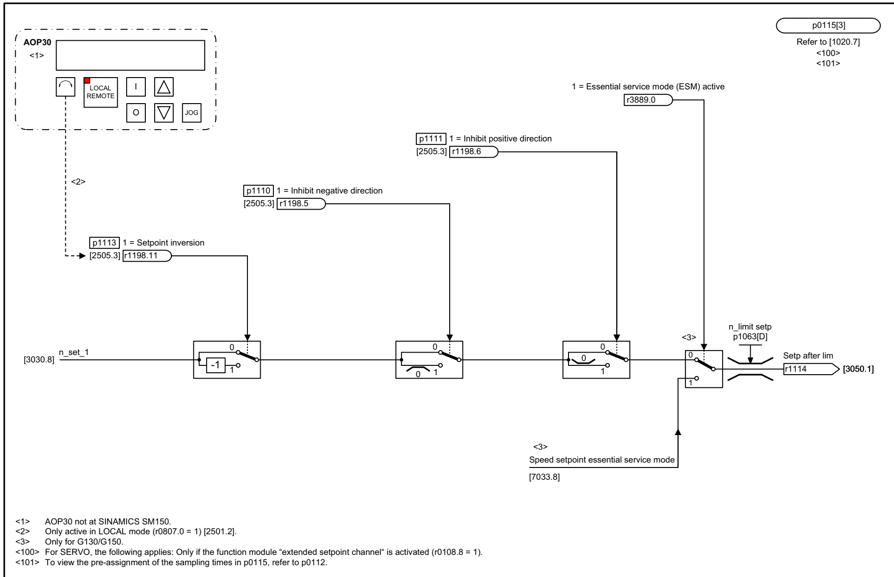
Fig. 2-117 3040 – Direction limitation and direction reversal
