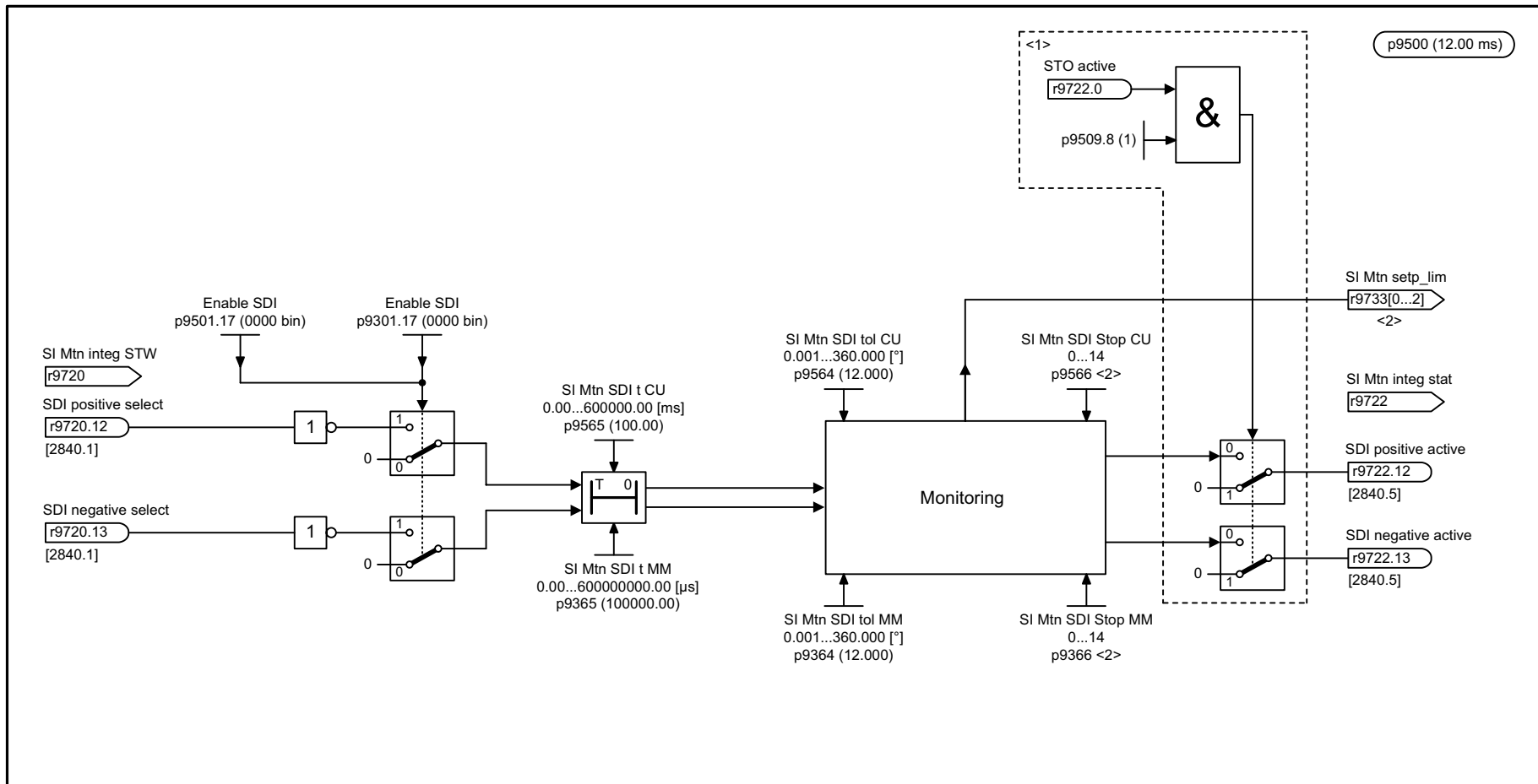
Fig. 2-98 2824 – SDI (Safe Direction)
