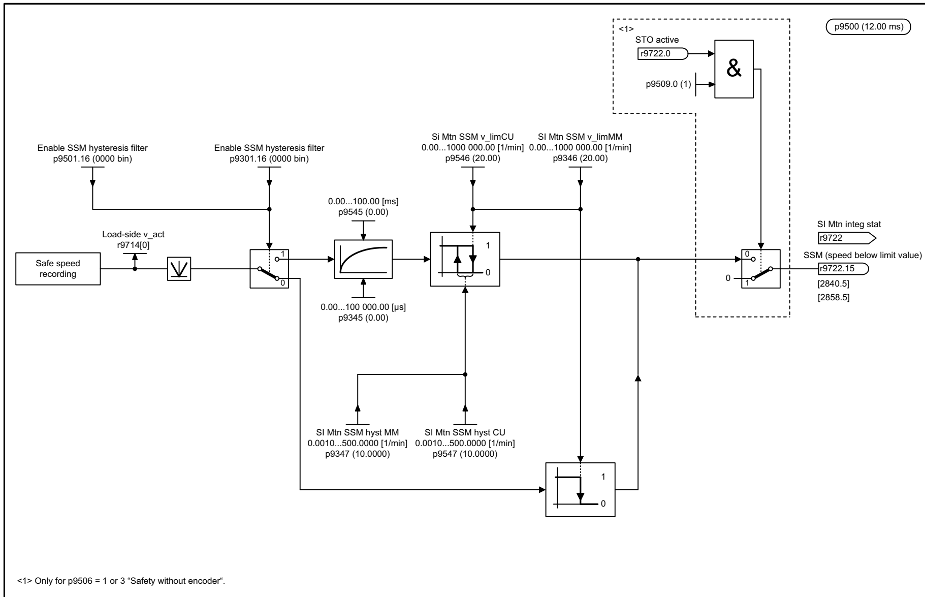
Fig. 2-97 2823 – SSM (Safe Speed Monitor)
