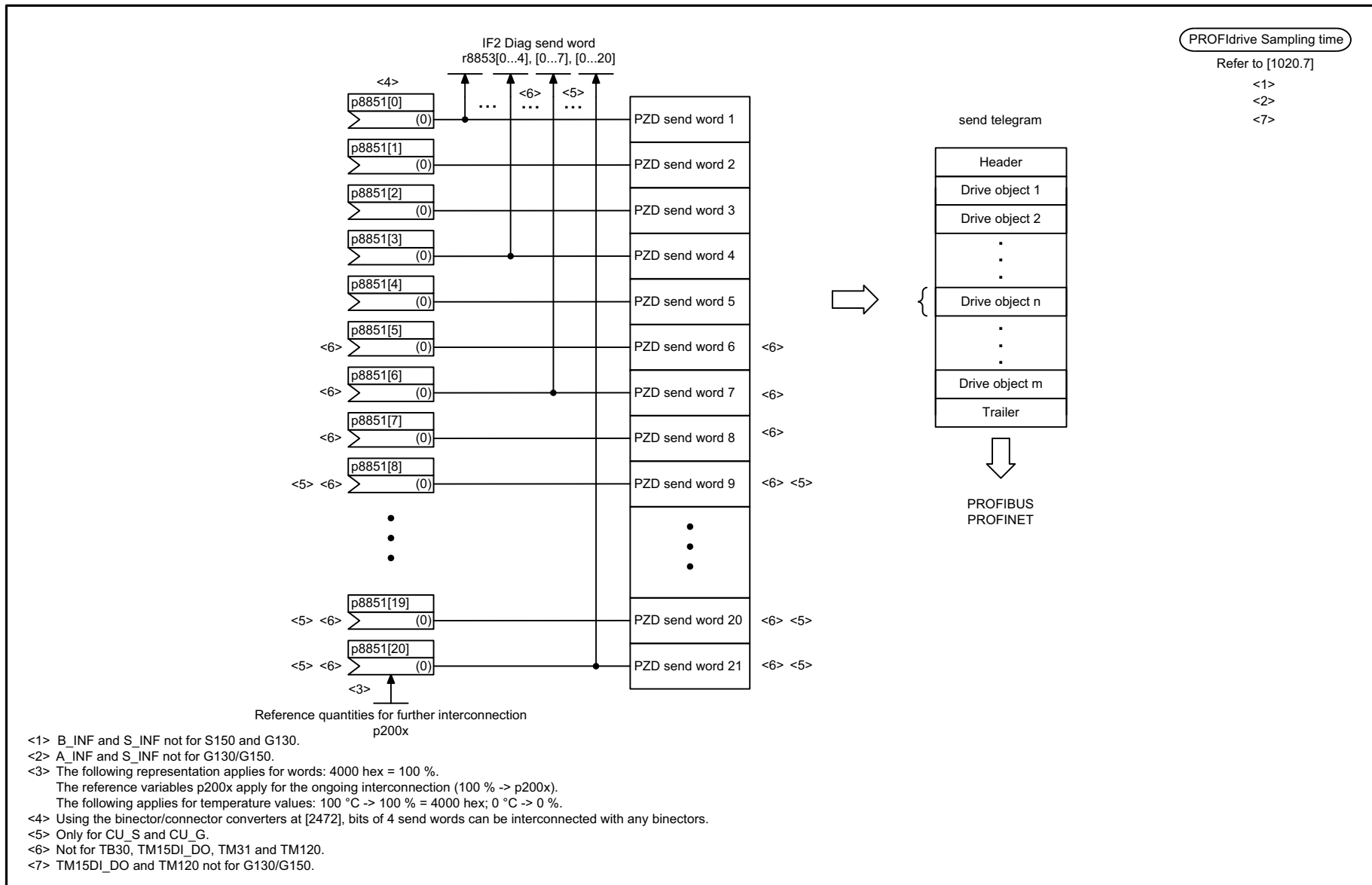
Fig. 2-61 2493 – IF2 send telegram, free interconnection
