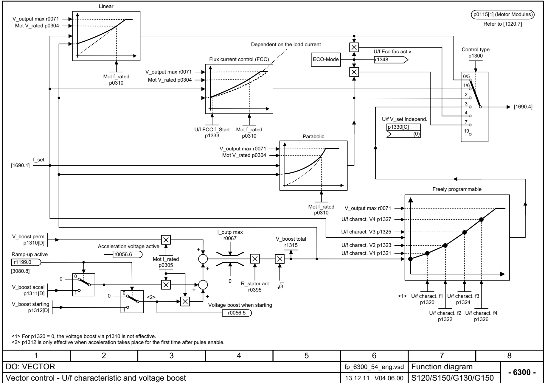
Fig. 2-130 6300 – V/f characteristic and voltage boost
