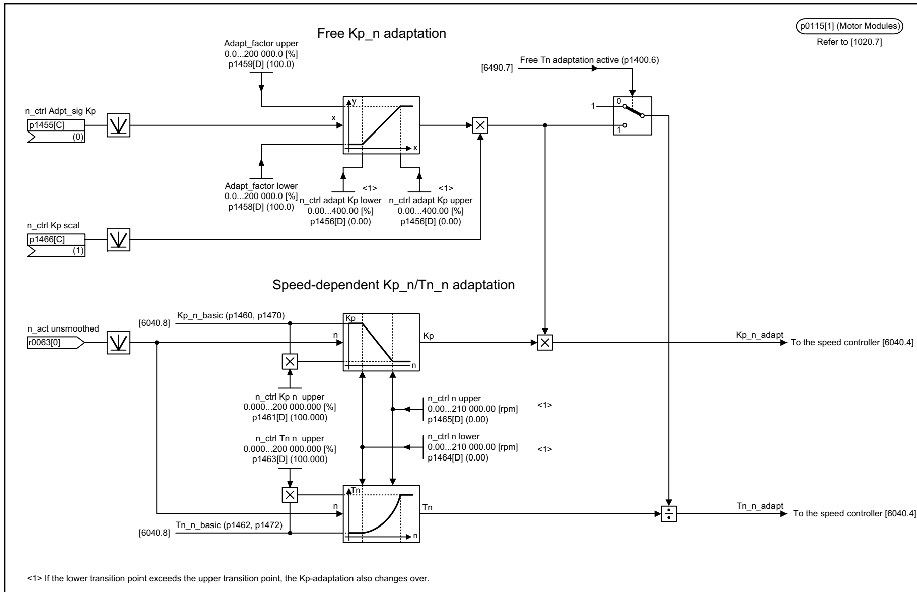
Fig. 2-127 6050 – Speed controller adaptation (Kp n /Tn n adaptation)
