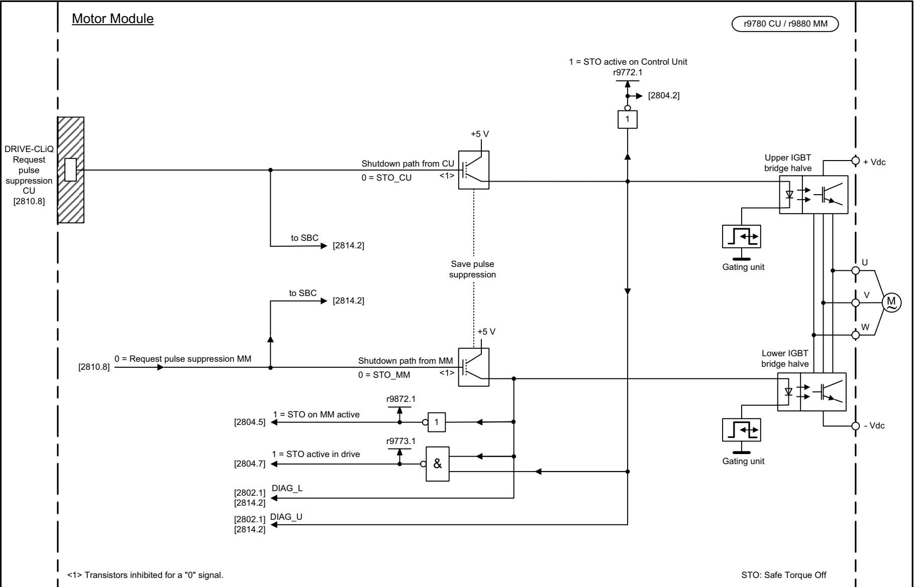
Fig. 2-91 2811 – STO (Safe Torque Off), safe pulse suppression
