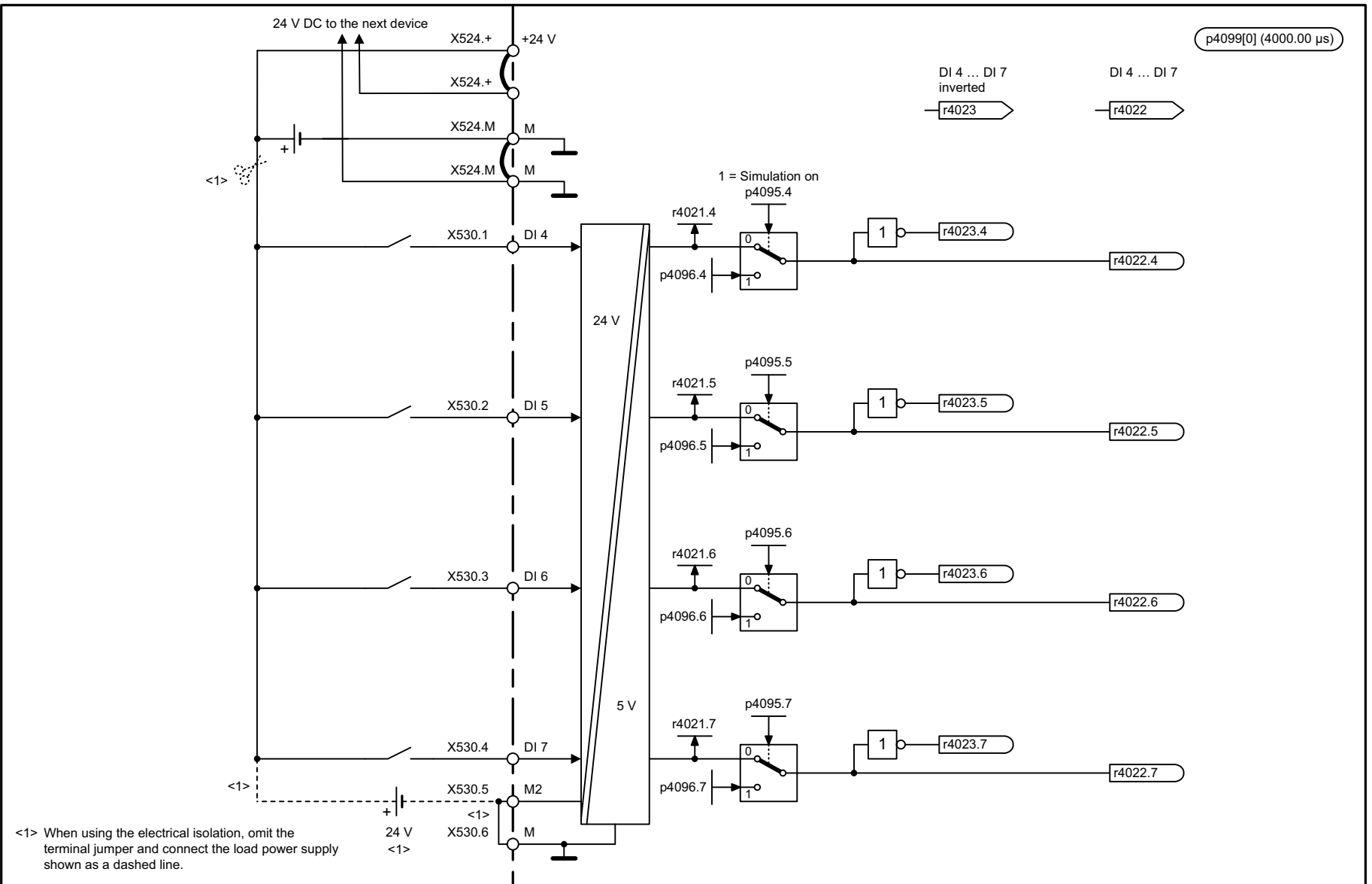
Fig. 2-191 9552 – Digital inputs, electrically isolated (DI 4 ... DI 7)
