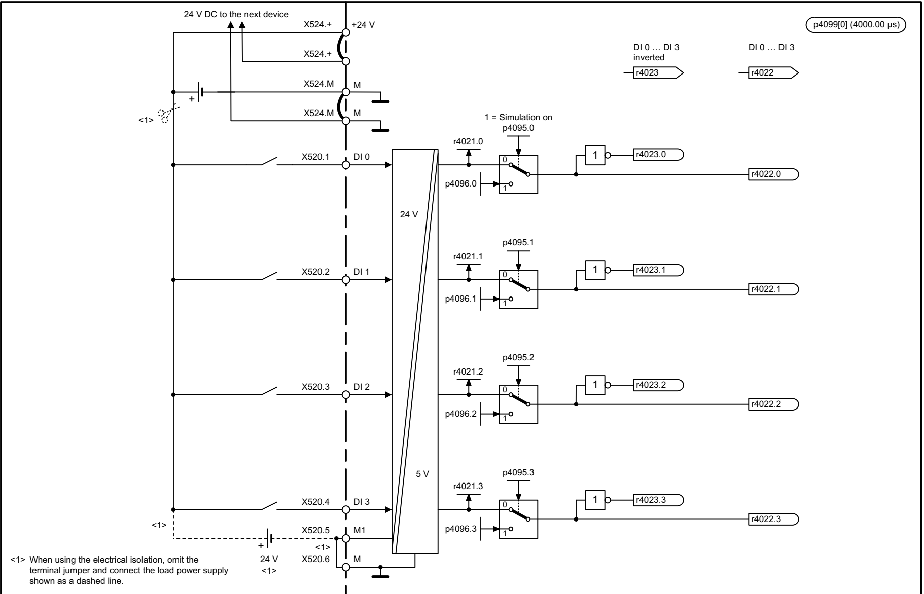
Fig. 2-190 9550 – Digital inputs, electrically isolated (DI 0 ... DI 3)
