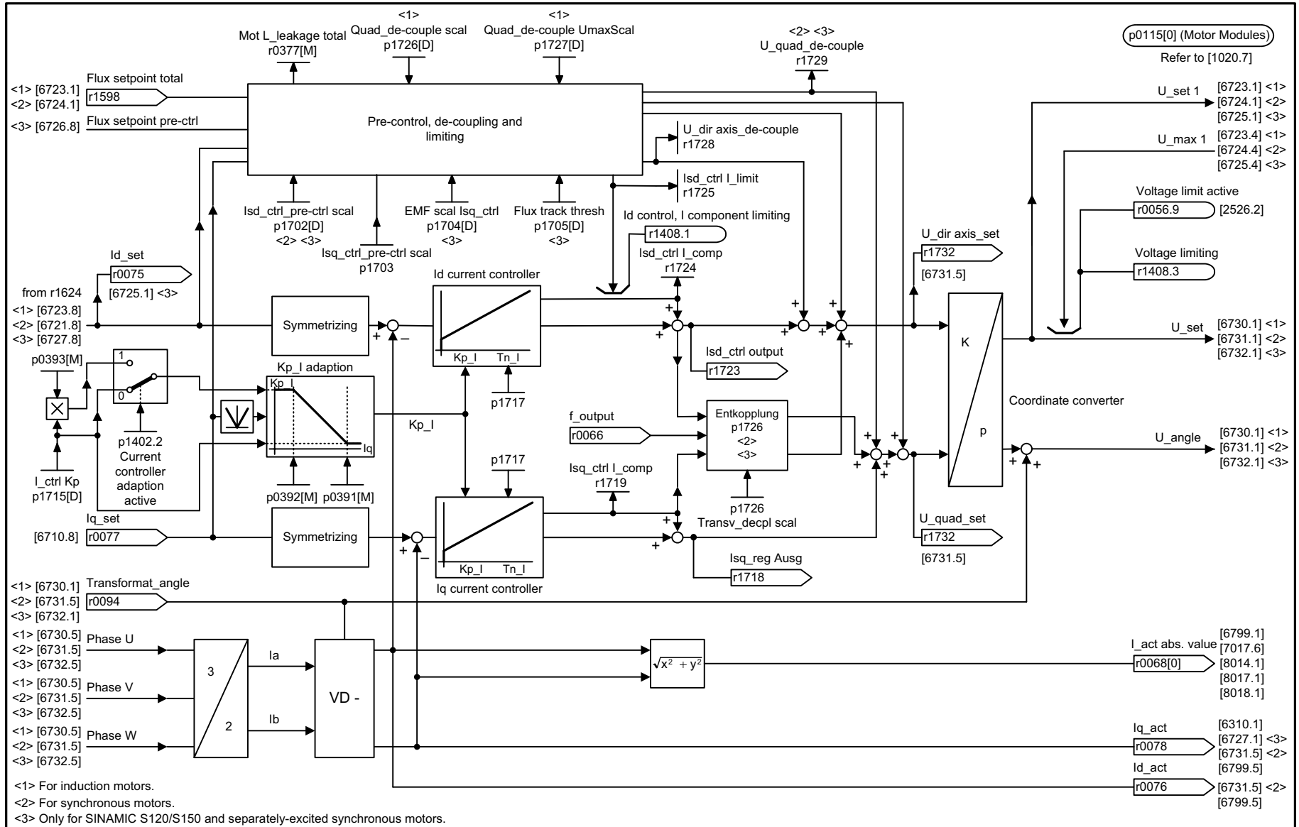
Fig. 2-138 6714 - Iq and Id controllers
