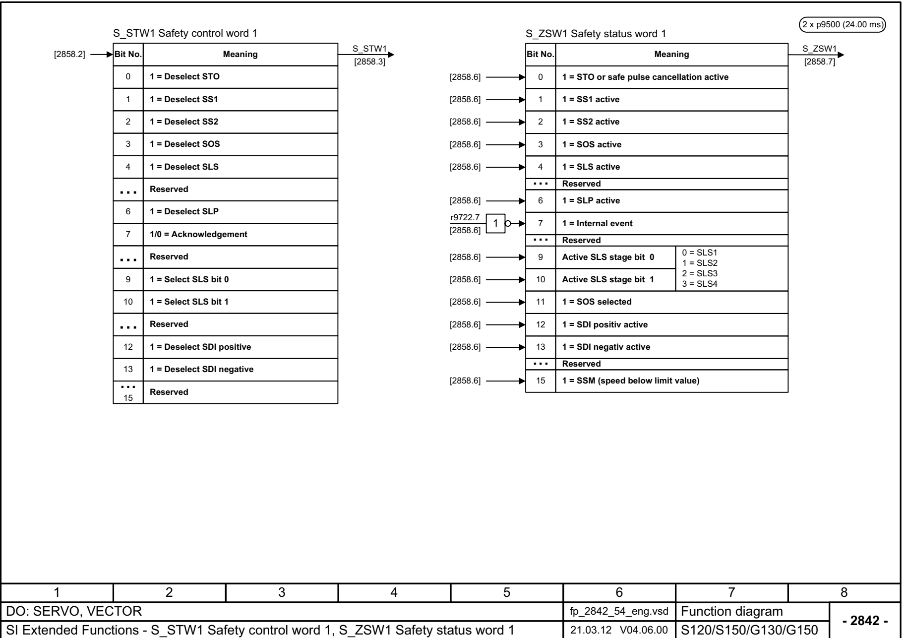
Fig. 2-102 2842 – S_STW1 Safety control word 1, S_ZSW1 Safety status word 1
