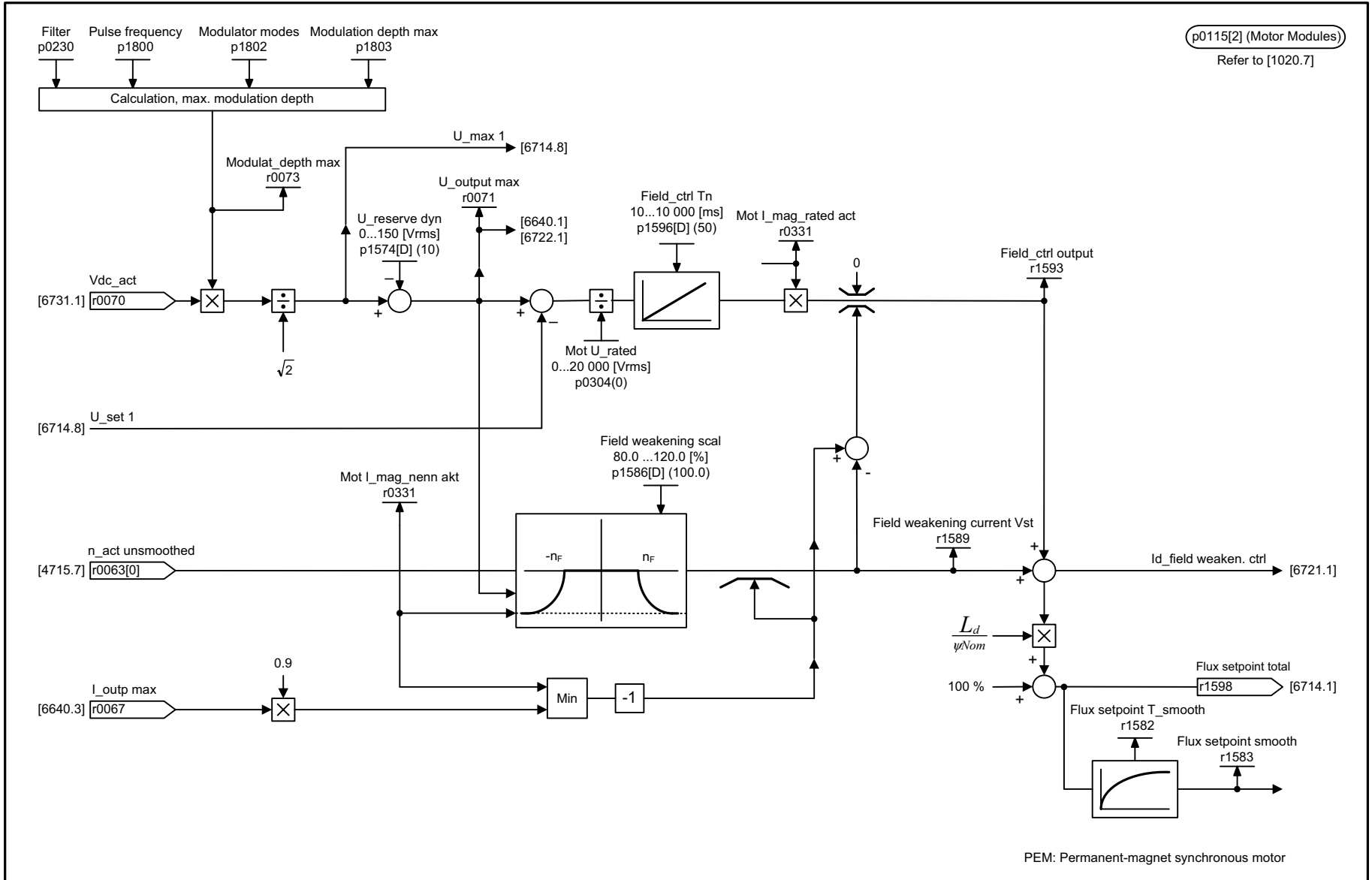
Fig. 2-142 6724 – Field weakening controller (PEM, p0300 = 2)
