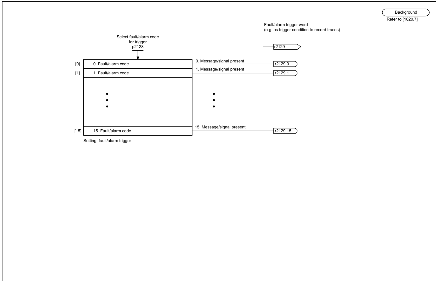
Fig. 2-166 8070 – Fault/alarm trigger word (r2129)
