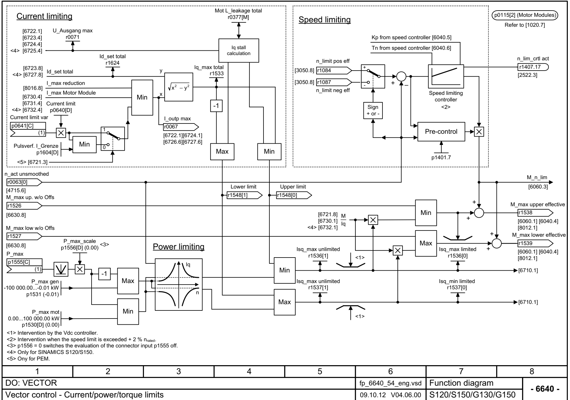
Fig. 2-136 6640 – Current/power/torque limits
