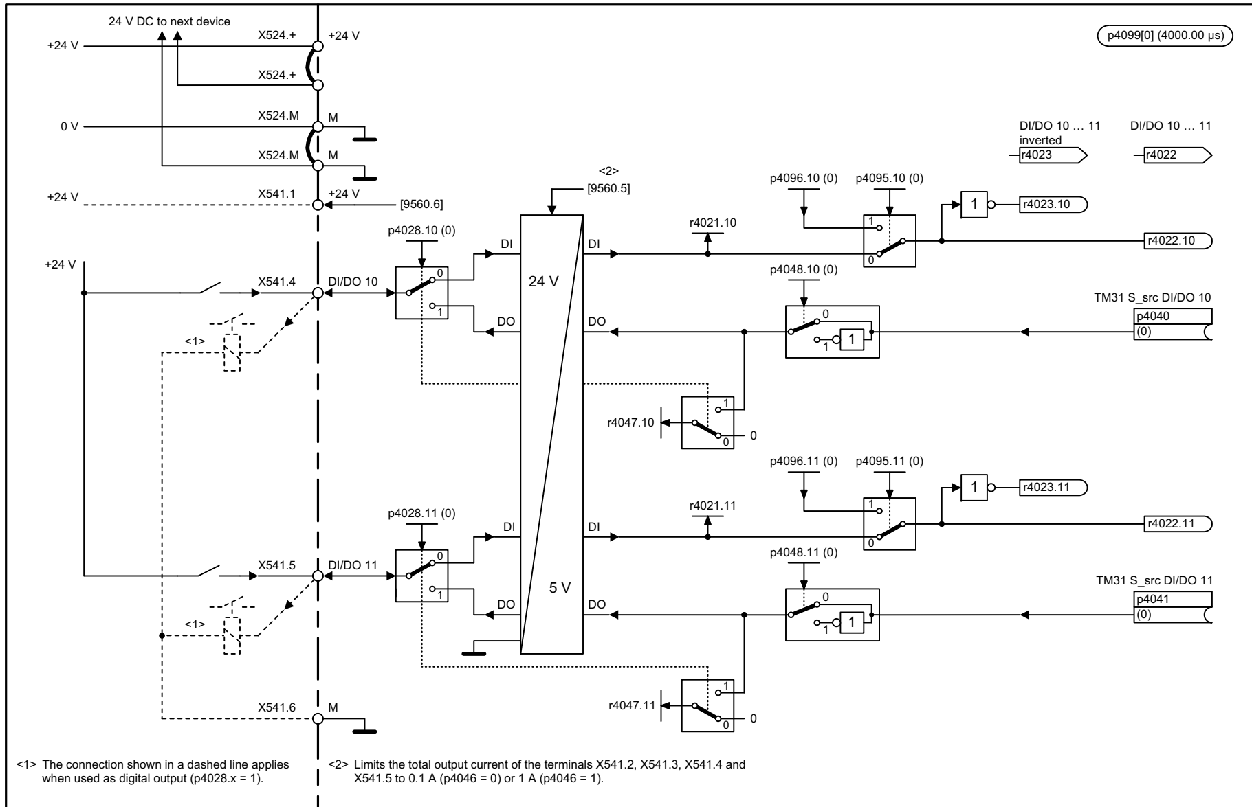
Fig. 2-194 9562 – Digital inputs/outputs, bidirectional (DI/DO 10 to DI/DO 11)
