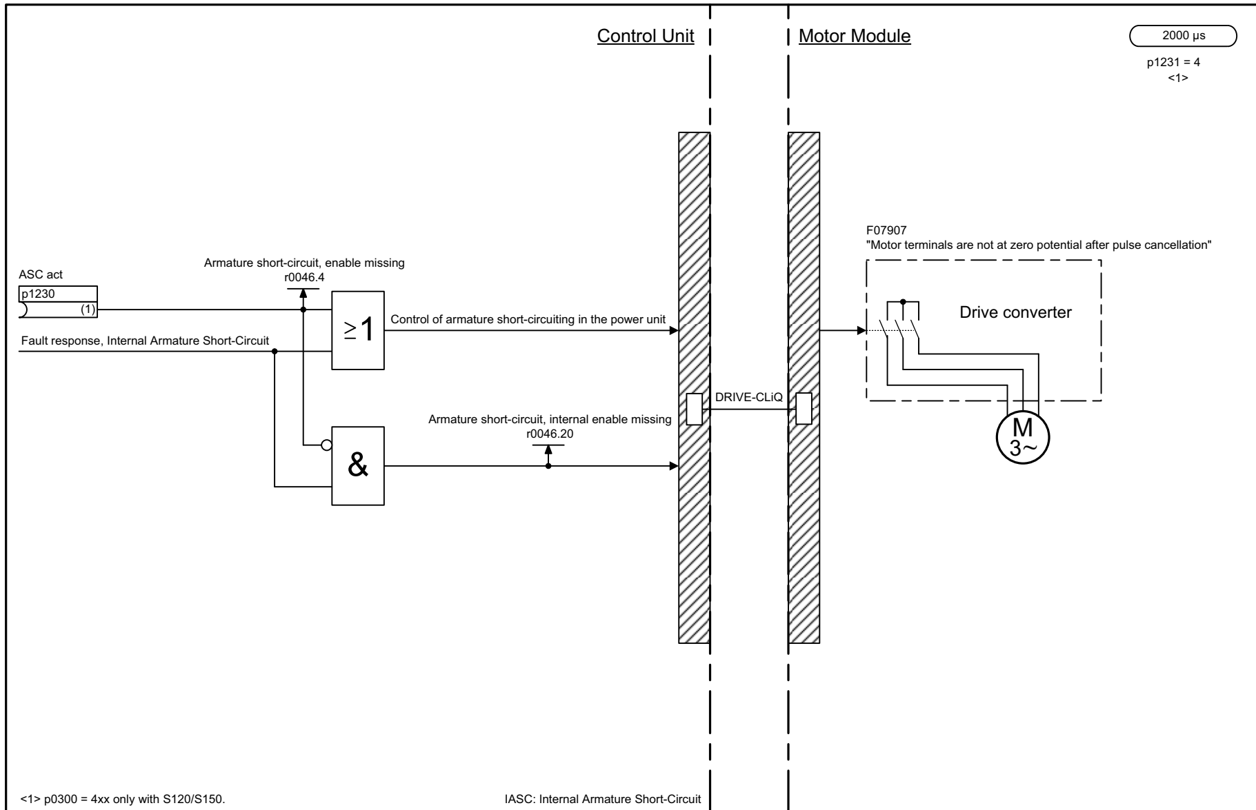
Fig. 2-148 7016 – Internal Armature Short-Circuit (IASC, p0300 = 2xx or 4xx)
