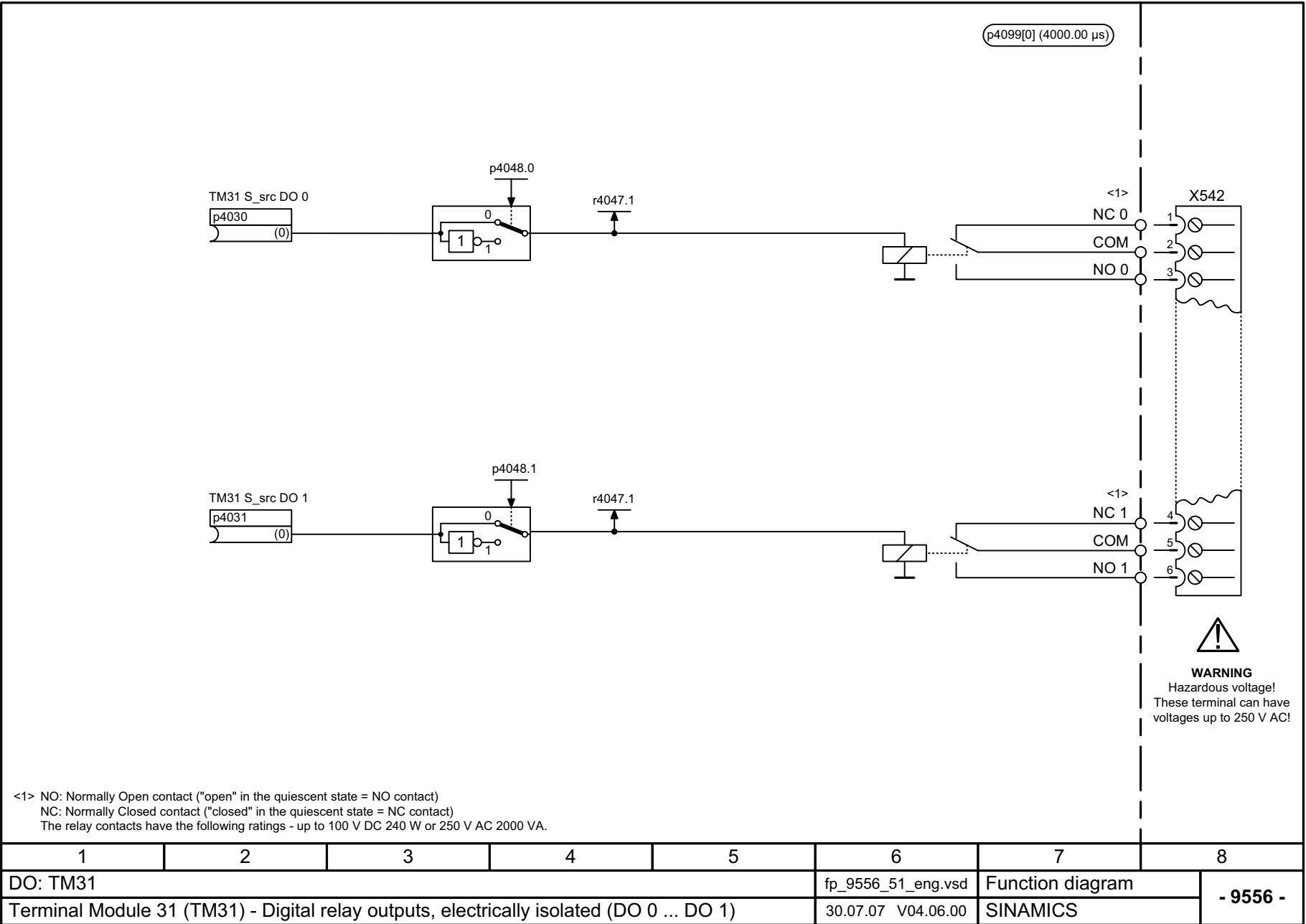
Fig. 2-192 9556 – Digital relay outputs, electrically isolated (DO 0 ... DO 1)
