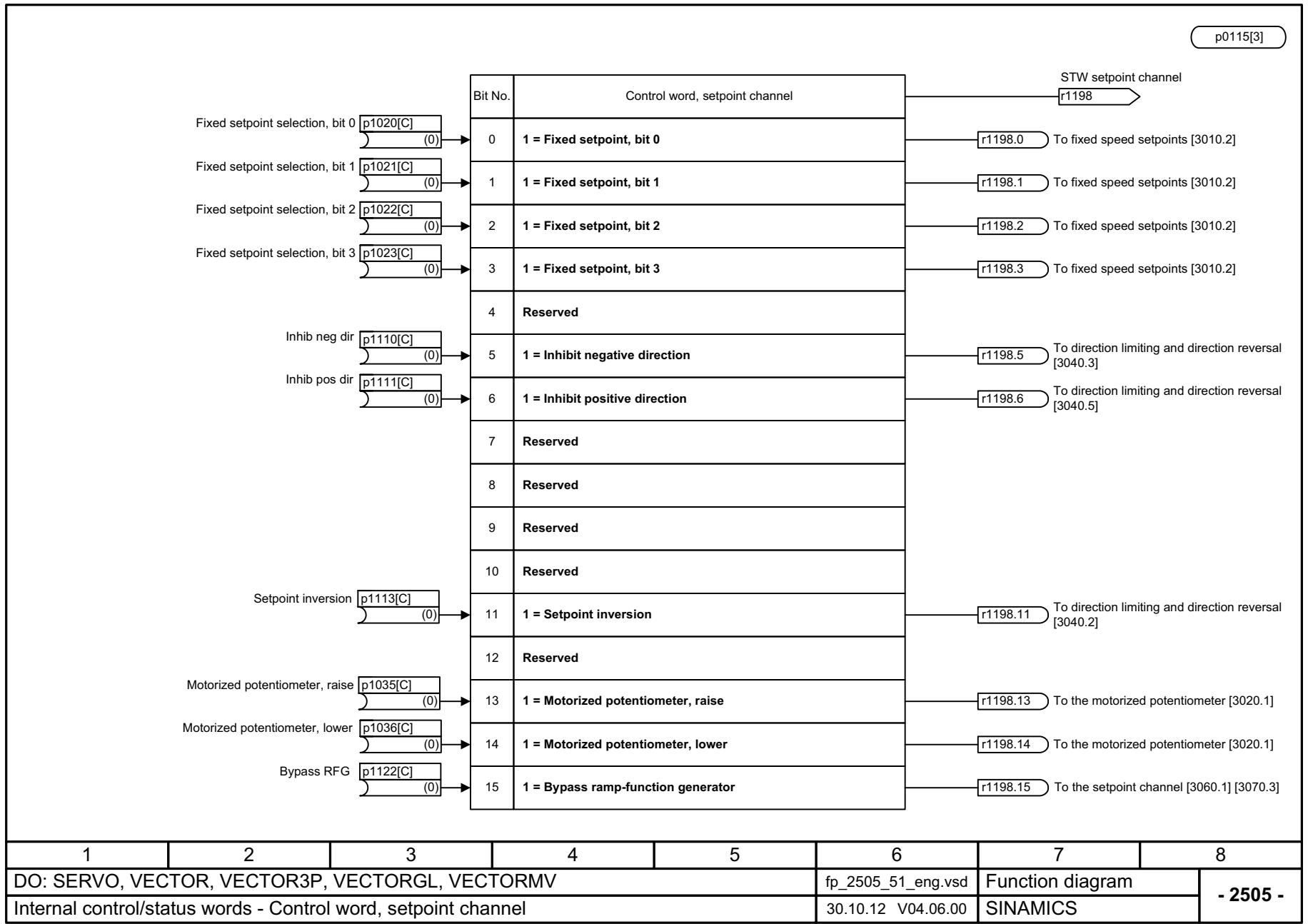
Fig. 2-70 2505 – Control word, setpoint channel
