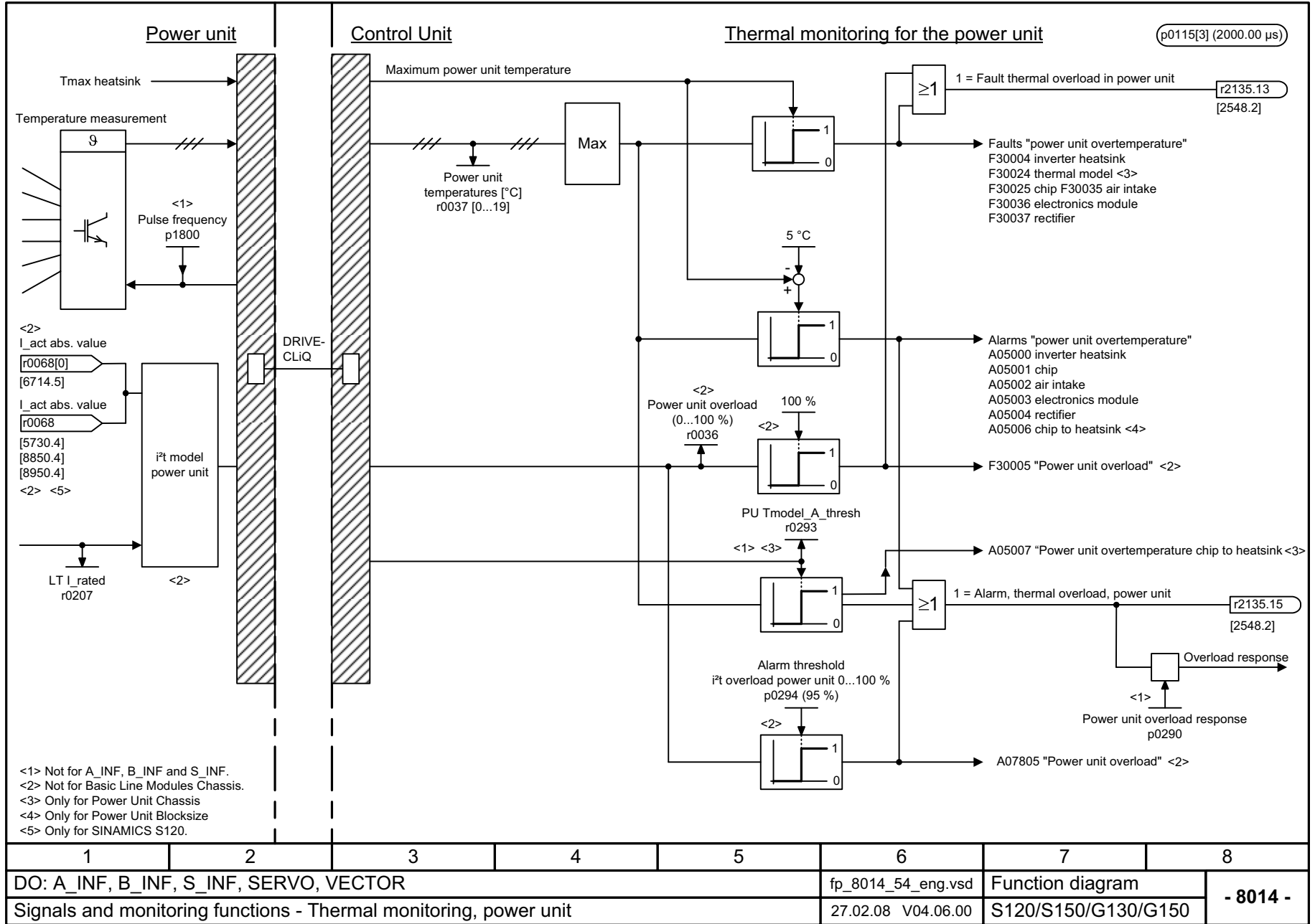
Fig. 2-161 8014 – Thermal monitoring, power unit
