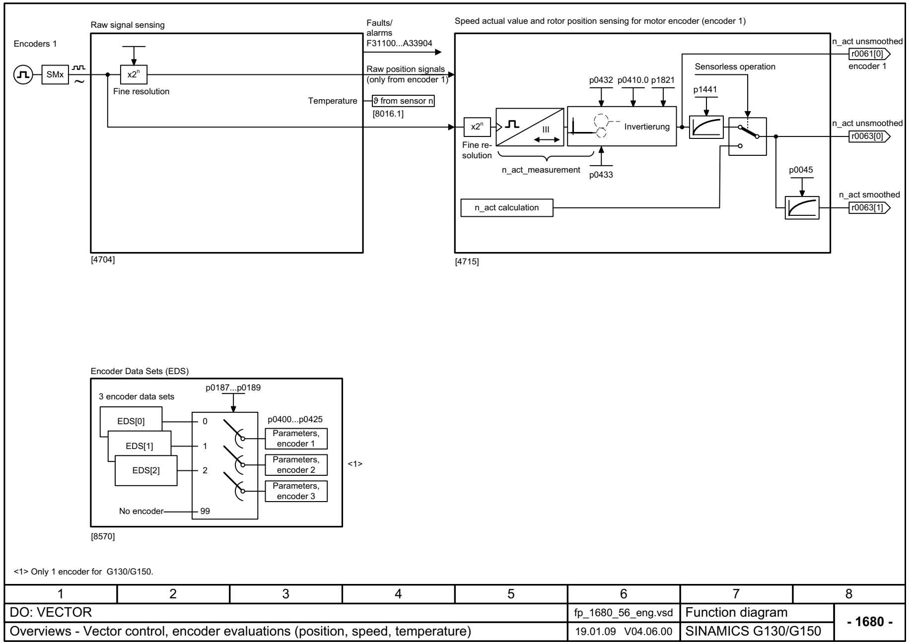
Fig. 2-9 1680 – Vector control, encoder evaluations (position, speed, temperature)
