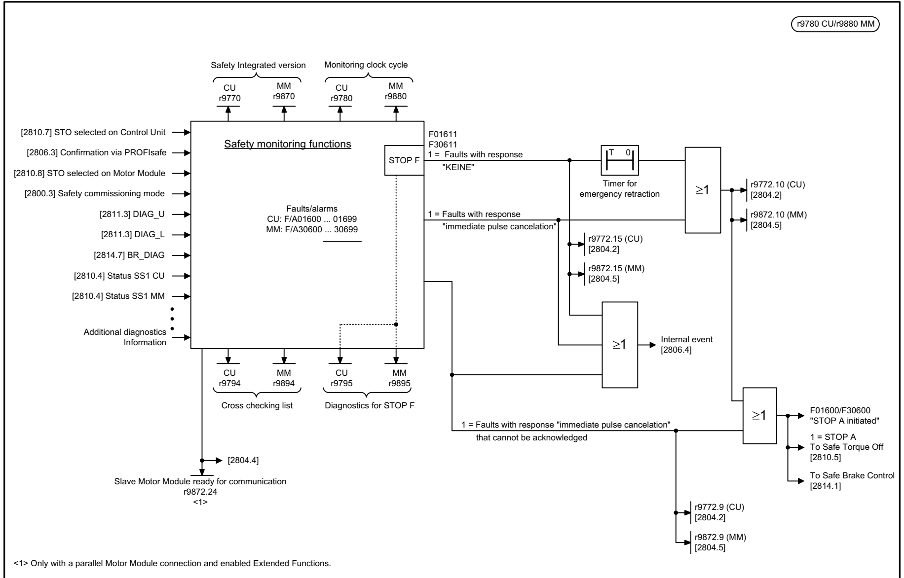
Fig. 2-87 2802 – Monitoring functions and faults/alarms
