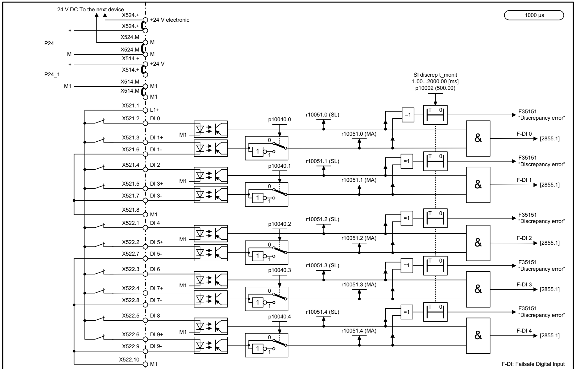
Fig. 2-106 2850 – TM54F (F-DI 0 ... F-DI 4)
