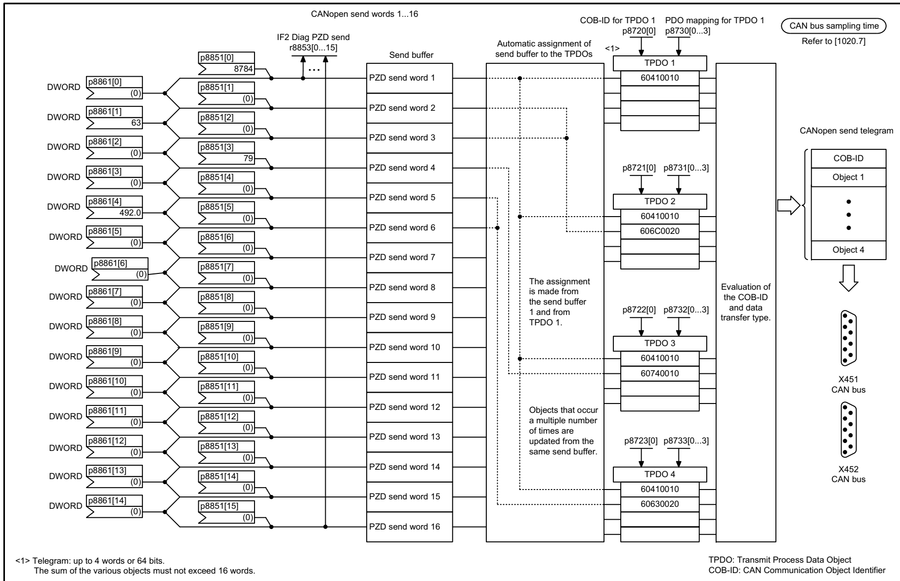
Fig. 2-187 9210 – Send telegram, Predefined Connection Set (p8744 = 1)
