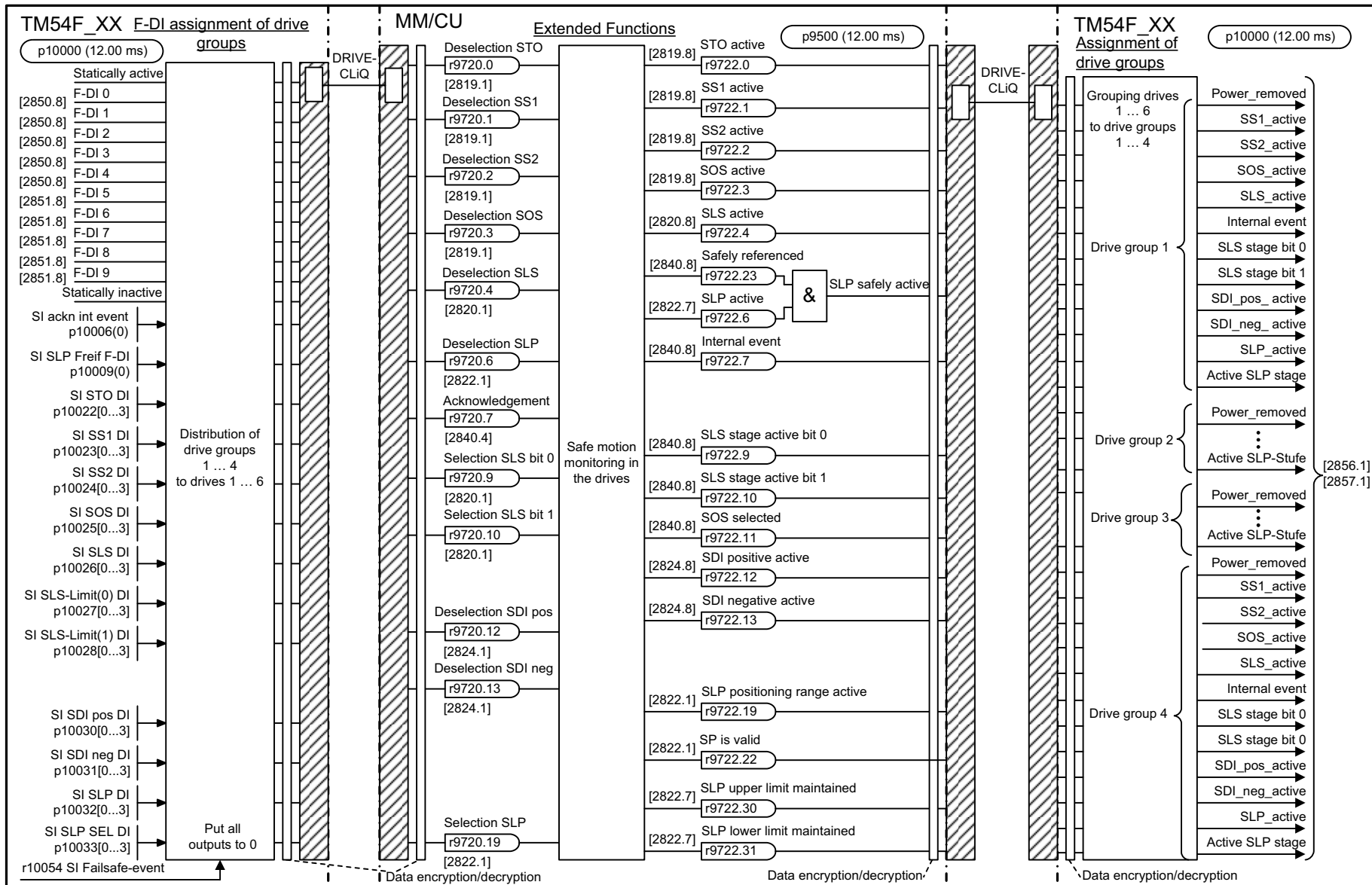
Fig. 2-109 2855 – TM54F control interface (p9601.2 = 1 & p9601.3 = 0)
