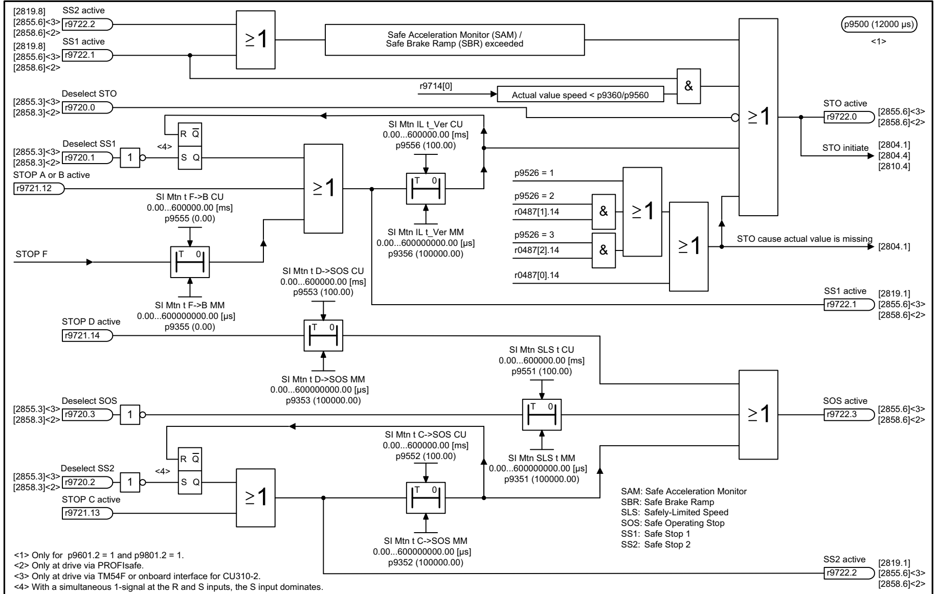
Fig. 2-94 2819 – SS1, SS2, SOS, Internal STOP B, C, D, F
