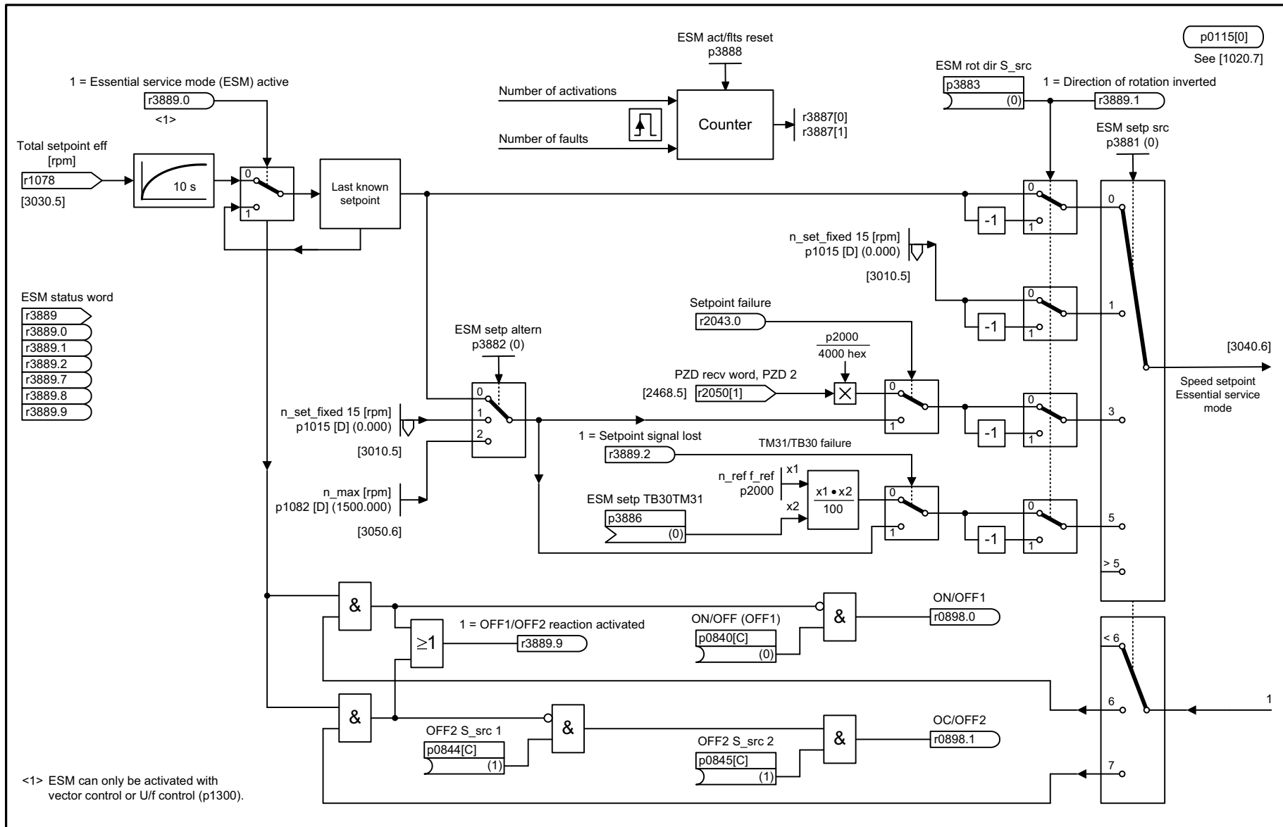
Fig. 2-151 7033 – Essential service mode (ESM)
