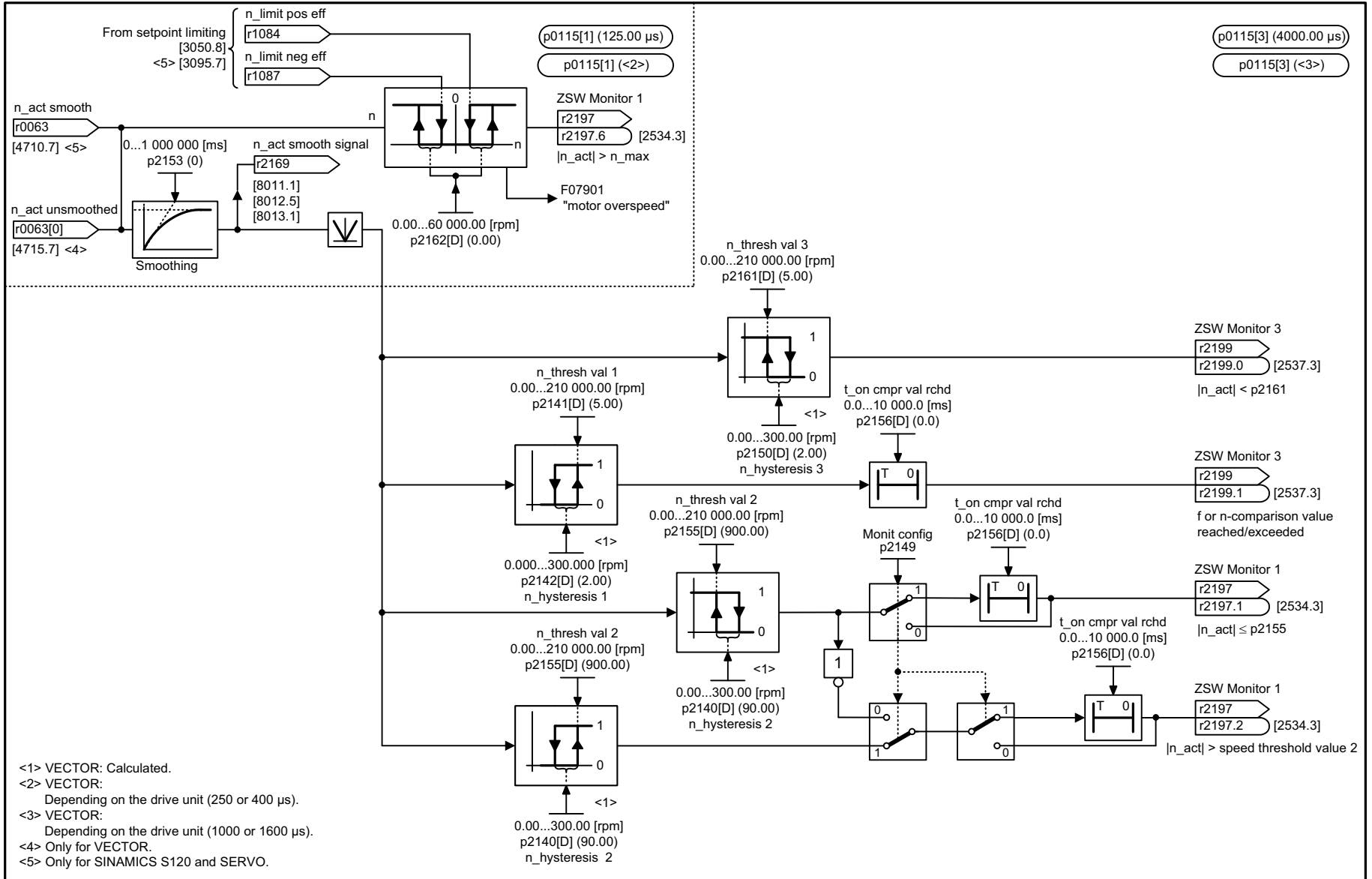
Fig. 2-157 8010 – Speed signals 1
