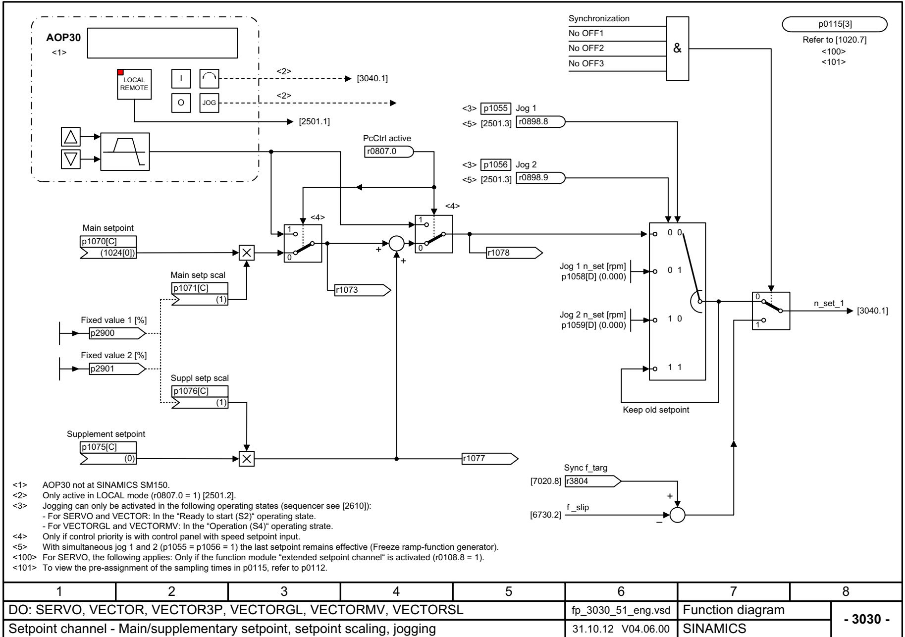
Fig. 2-116 3030 – Main/supplementary setpoint, setpoint scaling, jogging
