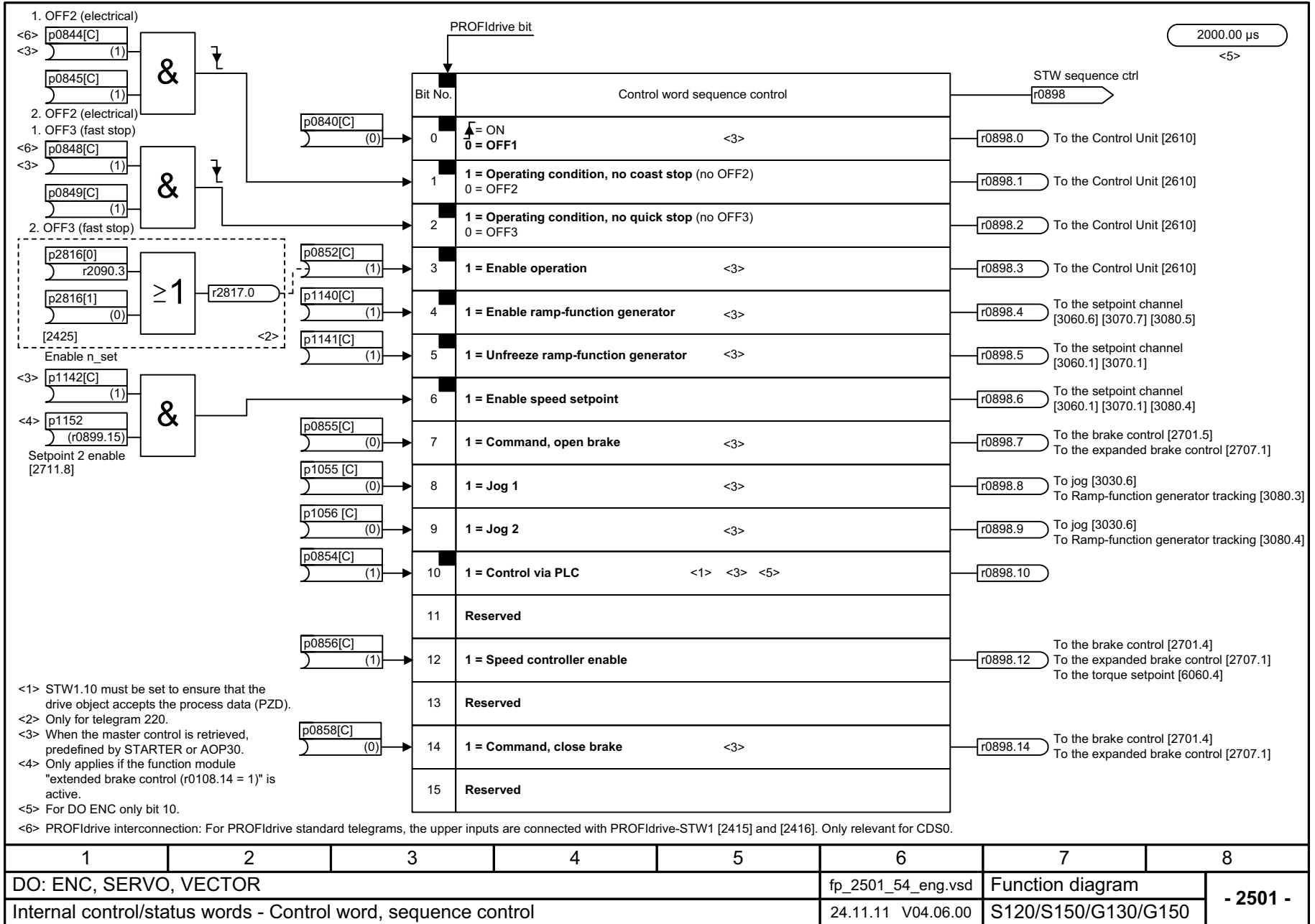
Fig. 2-68 2501 – Control word, sequence control
