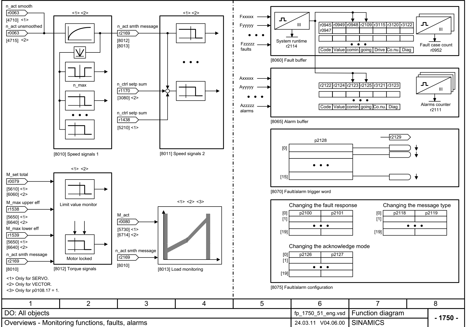
Fig. 2-13 1750 – Monitoring functions, faults, alarms
