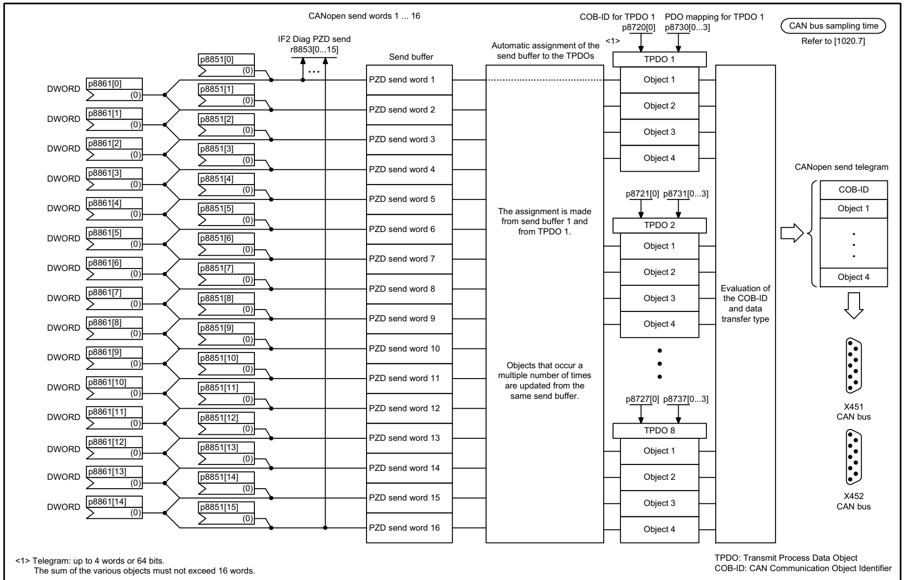
Fig. 2-186 9208 – Send telegram, free PDO mapping (p8744 = 2)
