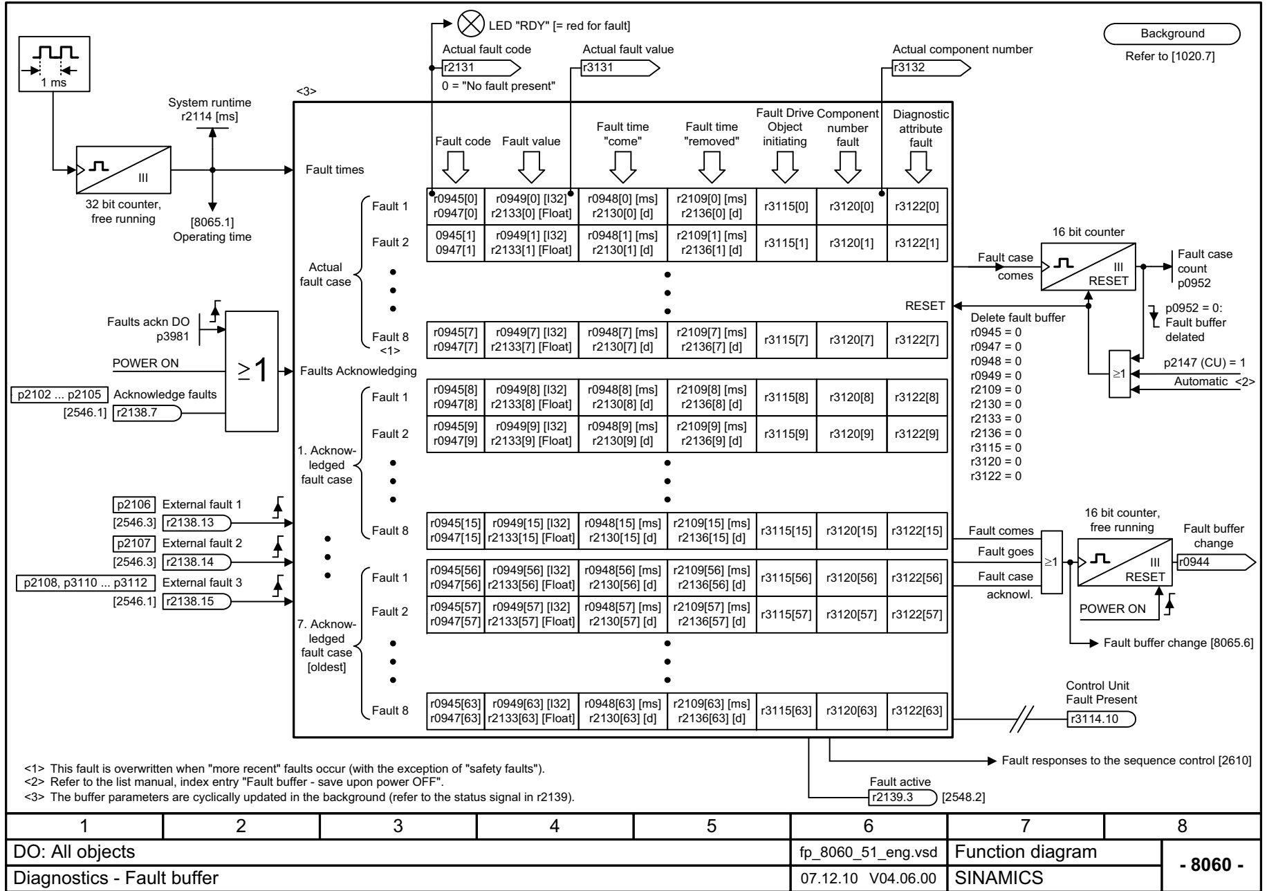
Fig. 2-164 8060 – Fault buffer
