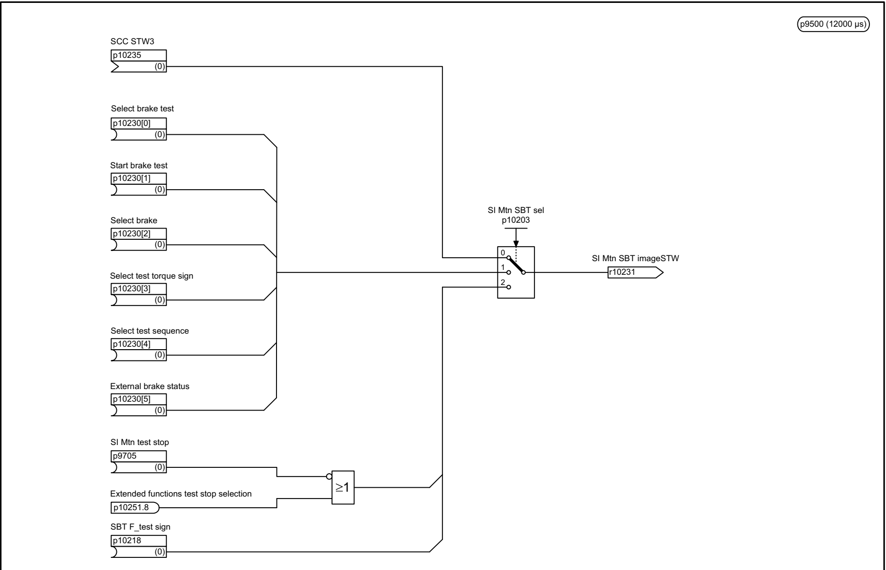
Fig. 2-100 2837 – Selection of active control word
