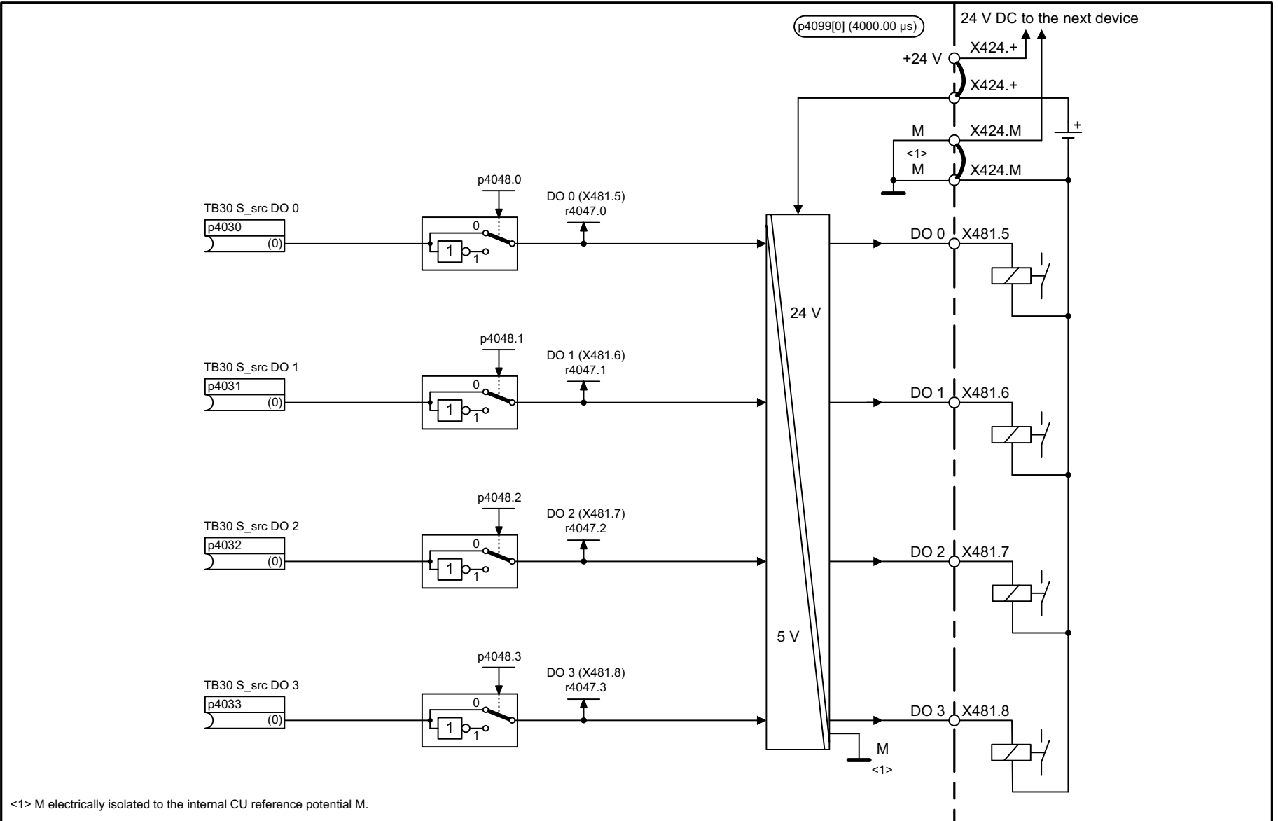
Fig. 2-181 9102 – Digital outputs, electrically isolated (DO 0 ... DO 3)
