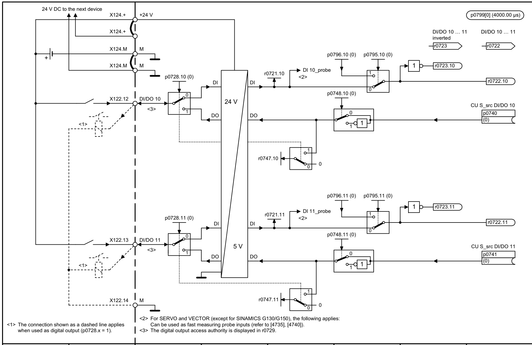
Fig. 2-21 2131 – Digital inputs/outputs, bidirectional (DI/DO 10 ... DI/DO 11)
