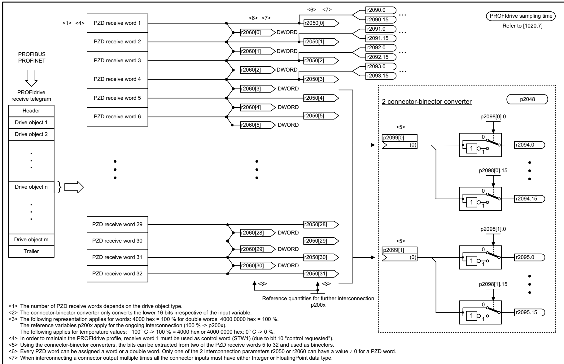
Fig. 2-52 2468 – IF1 receive telegram, free interconnection via BICO (p0922 = 999)
