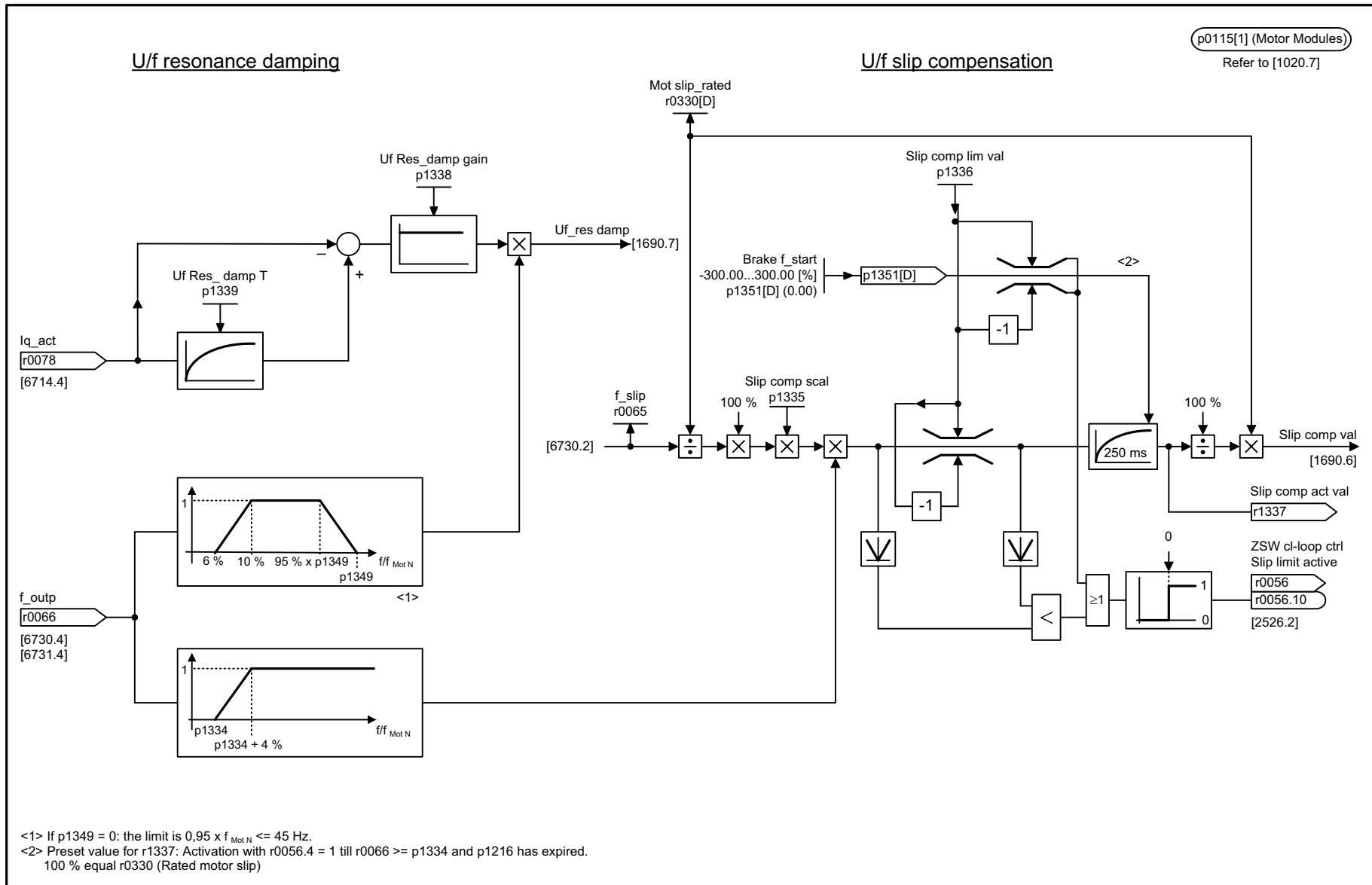
Fig. 2-131 6310 – Resonance damping and slip compensation
