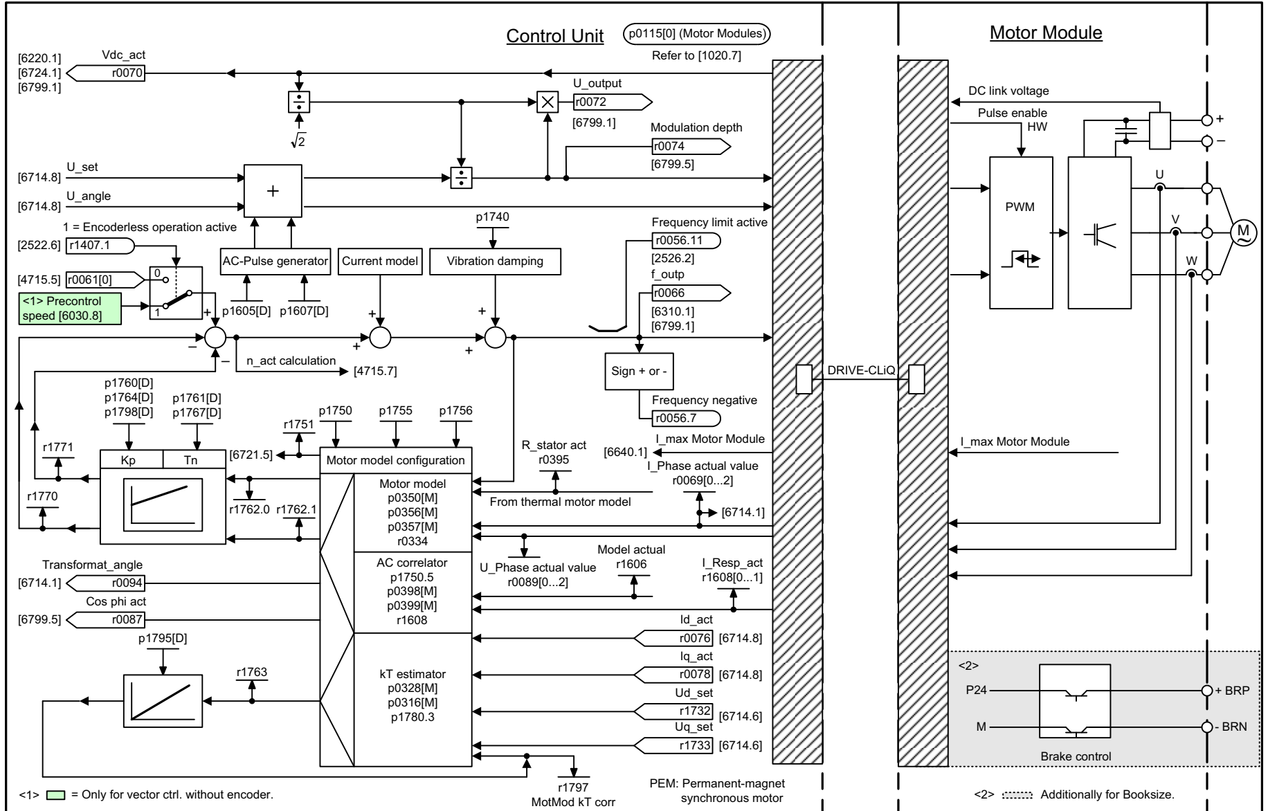
Fig. 2-144 6731 – Interface to the Motor Module (PEM, p0300 = 2)
