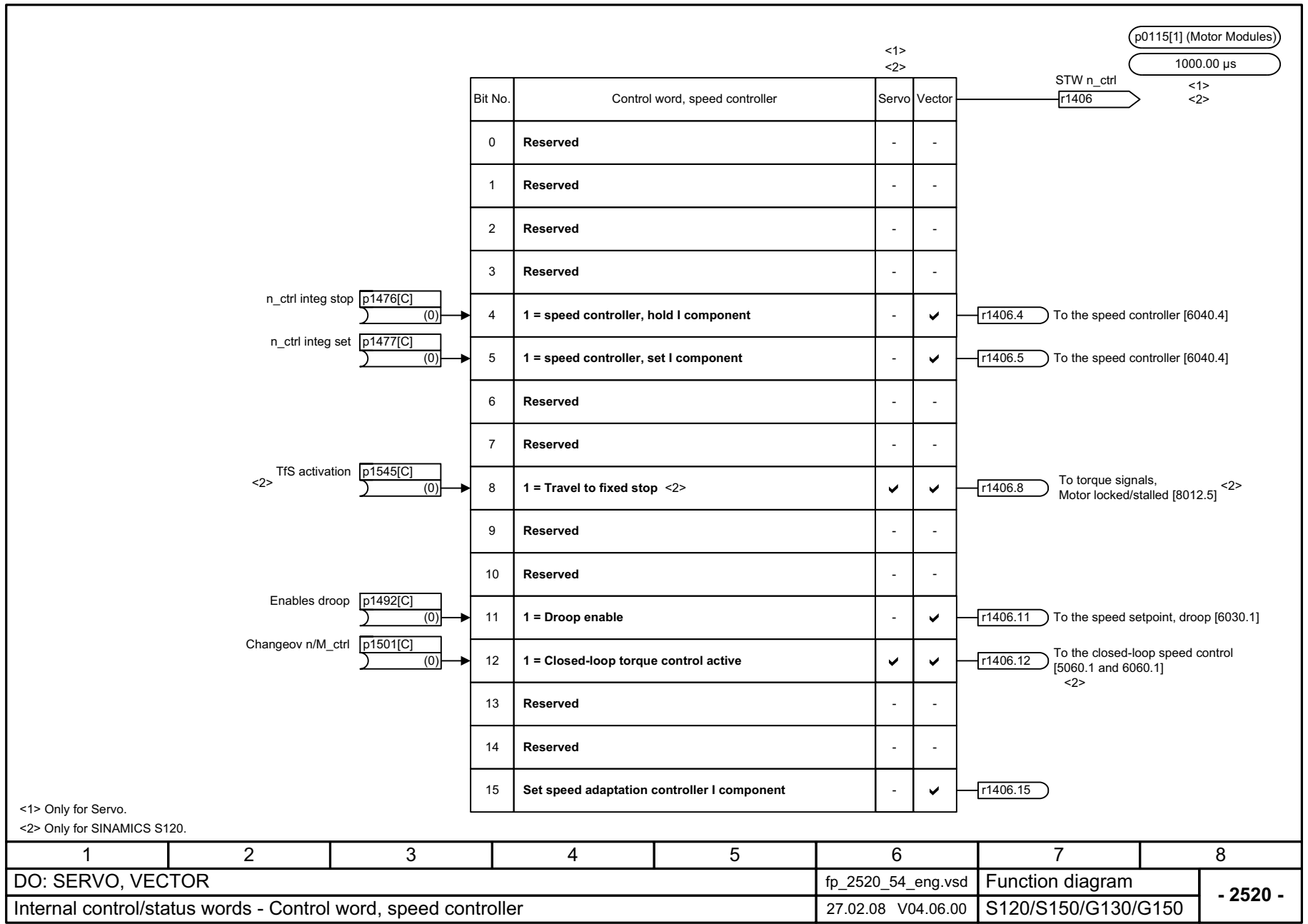
Fig. 2-71 2520 – Control word, speed controller
