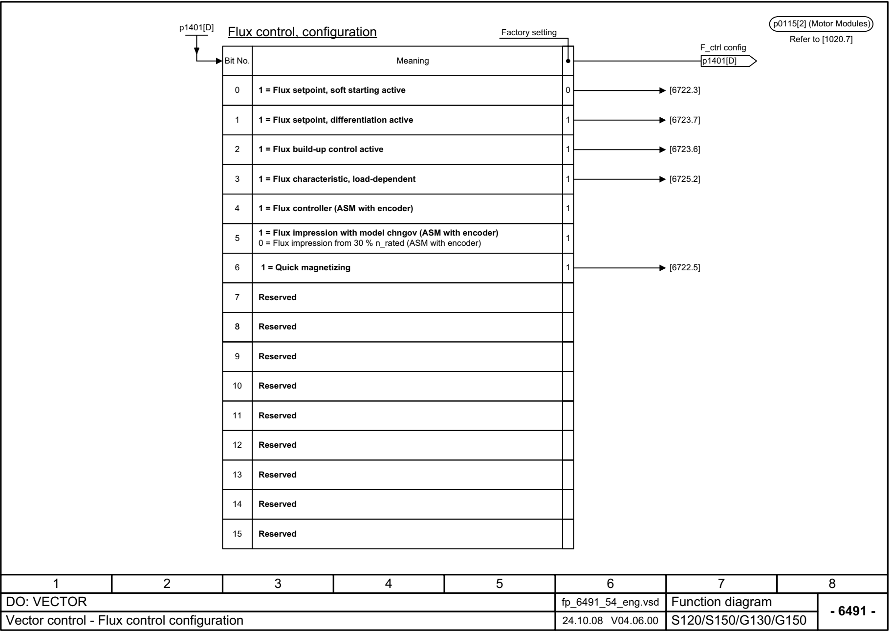
Fig. 2-134 6491 – Flux control configuration
