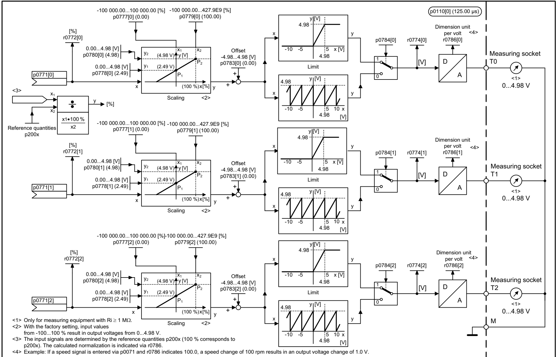
Fig. 2-168 8134 – Measuring sockets (T0, T1, T2)
