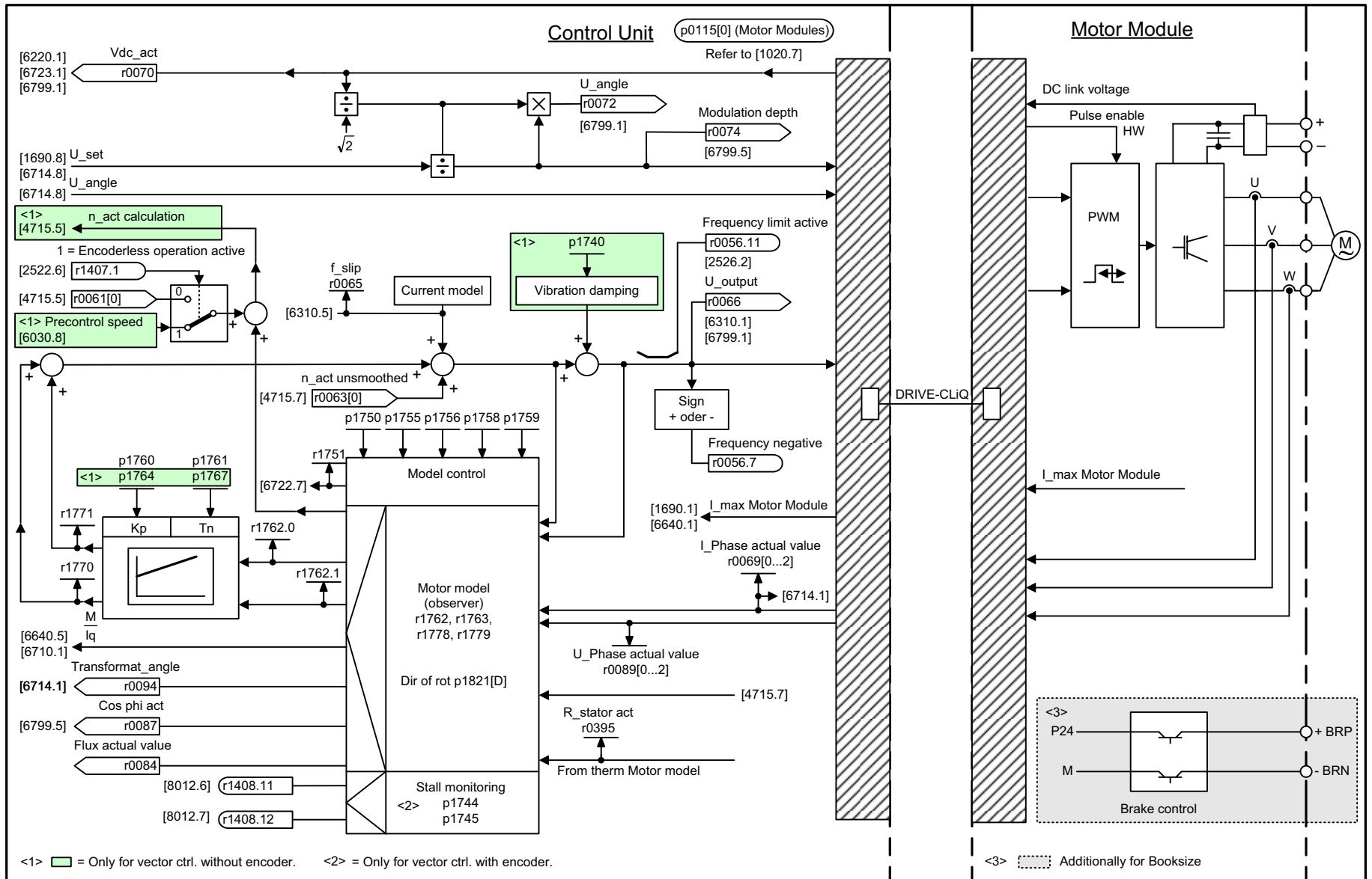
Fig. 2-143 6730 – Interface to the Motor Module (ASM, p0300 = 1)
