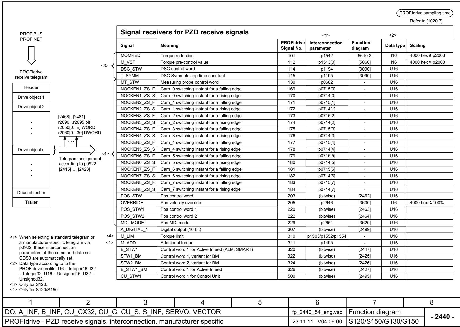
Fig. 2-41 2440 – PZD receive signals, interconnection, manufacturer-specific
