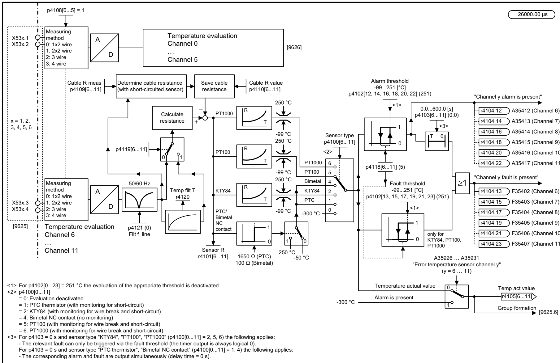
Fig. 2-201 9627 – Temperature evaluation 2x2-wire (channel 0 ... 11)
