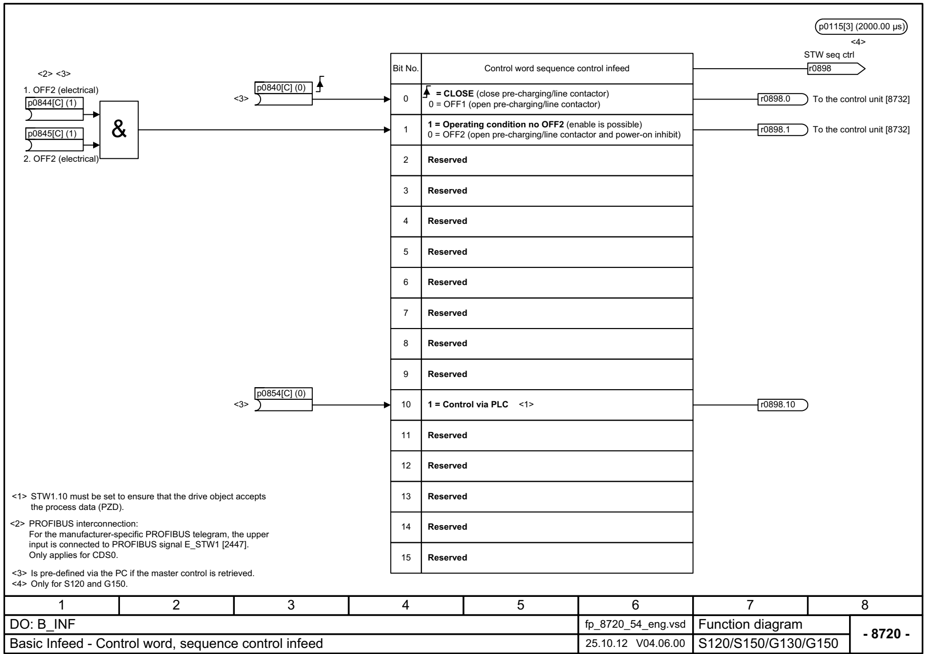
Fig. 2-174 8720 – Control word, sequence control infeed
