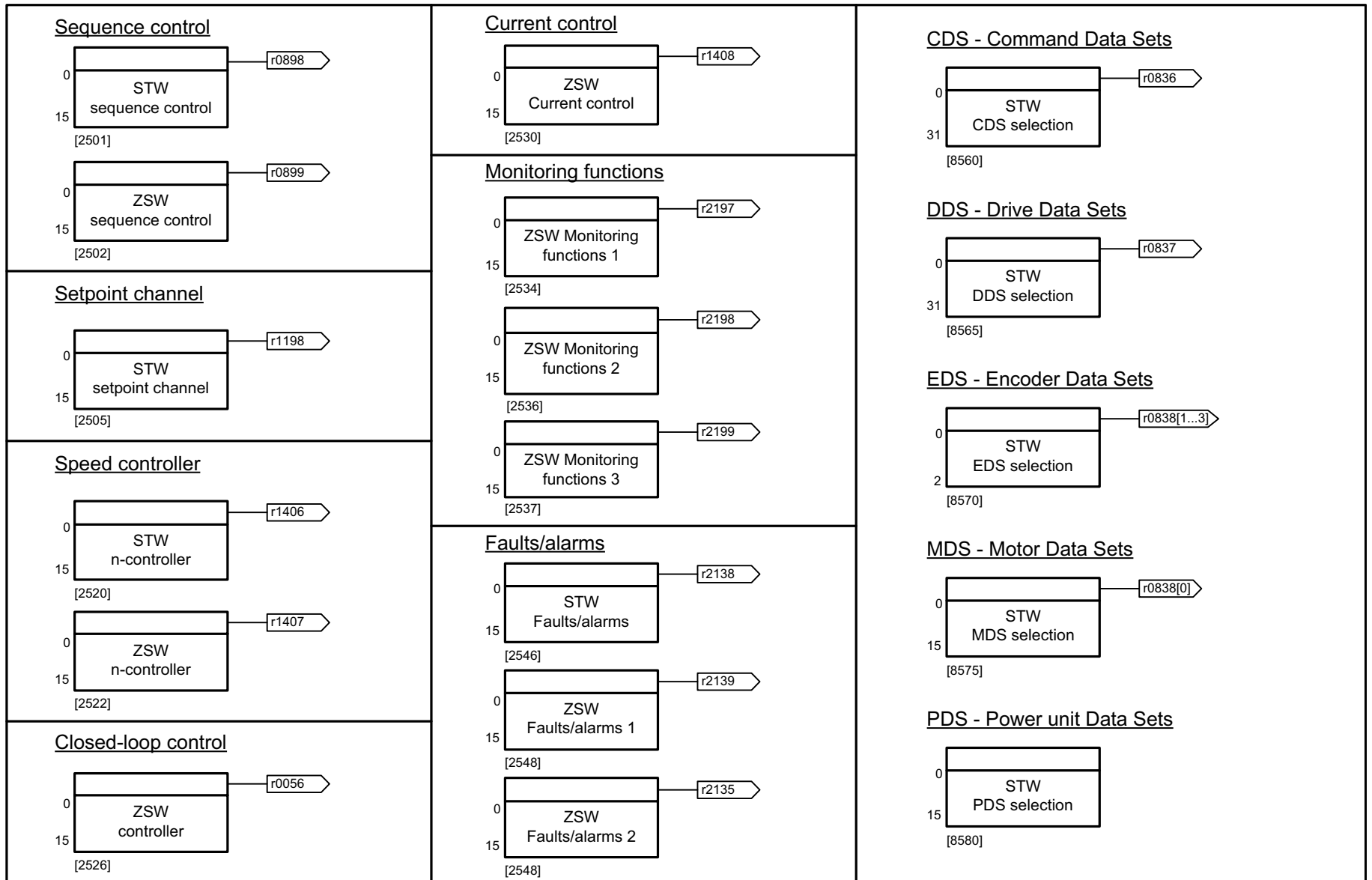
Fig. 2-7 1530 – Internal control/status words, data sets
