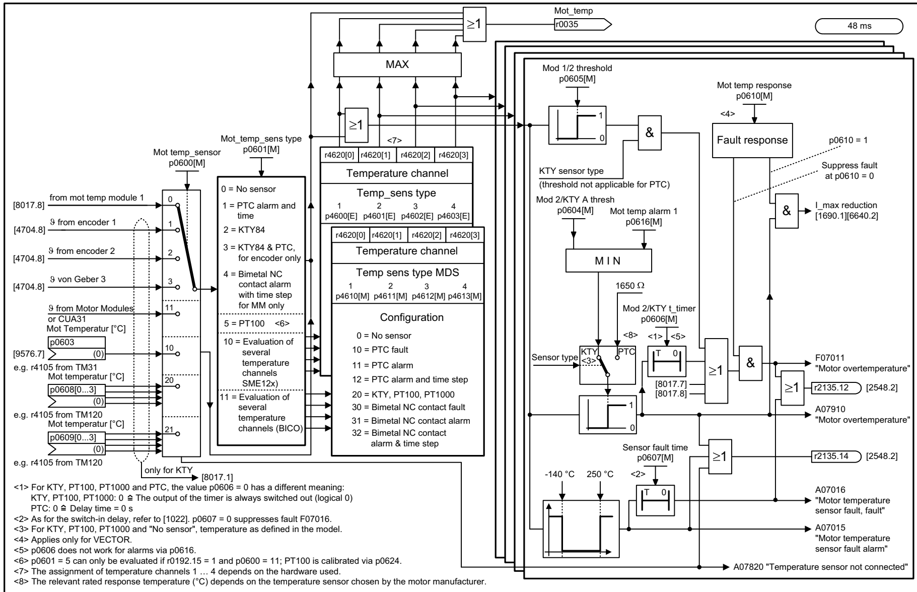
Fig. 2-162 8016 – Thermal monitoring, motor
