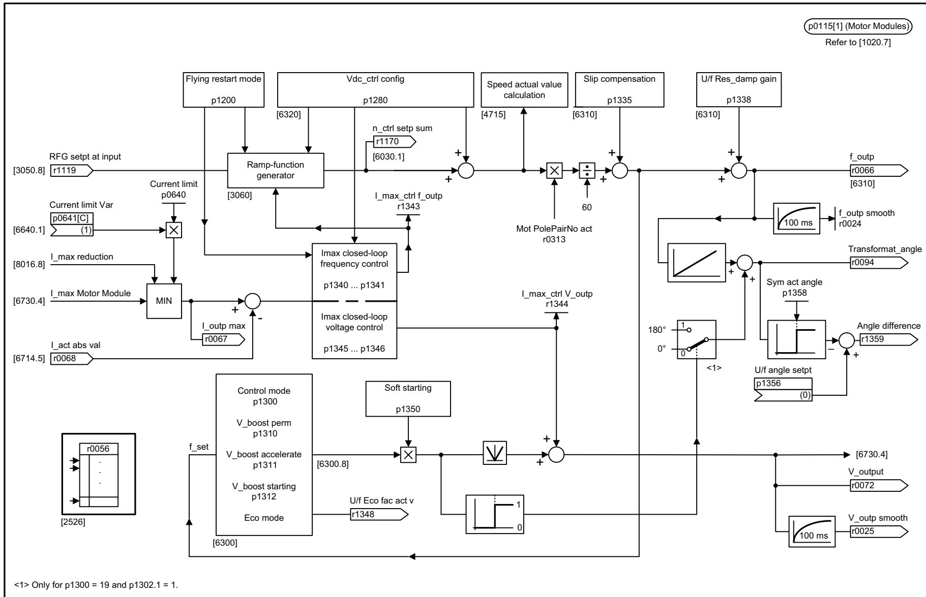
Fig. 2-10 1690 – Vector control, U/f control
