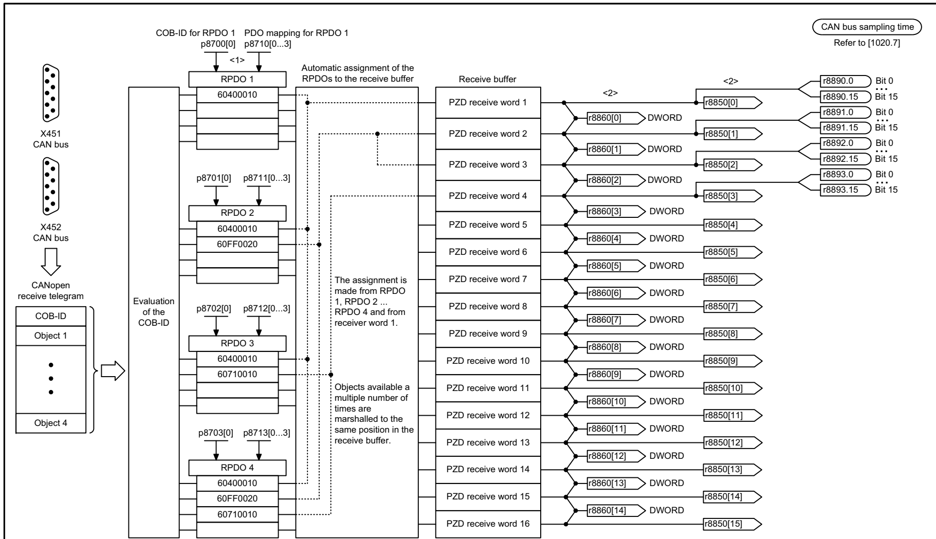
Fig. 2-185 9206 – Receive telegram, Predefined Connection Set (p8744 = 1)
