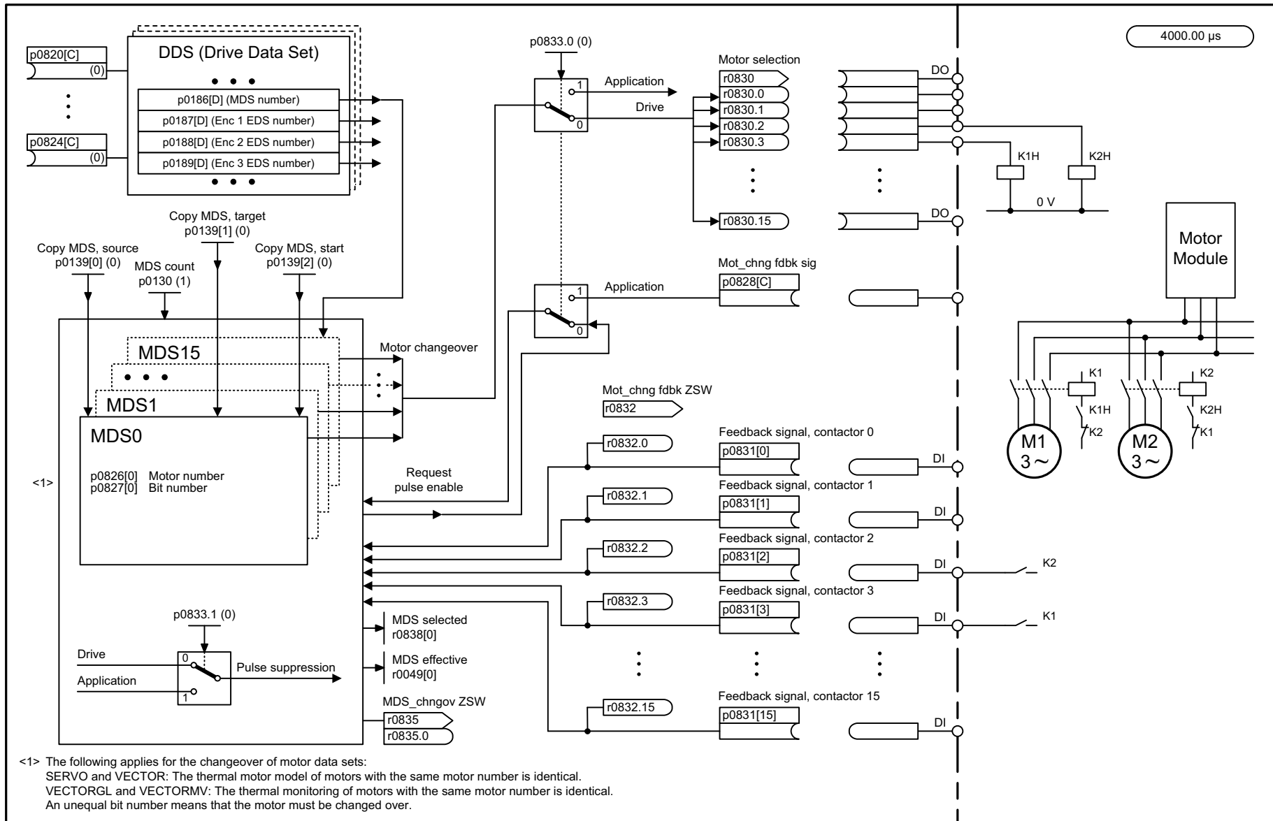
Fig. 2-172 8575 – Motor Data Sets (MDS)
