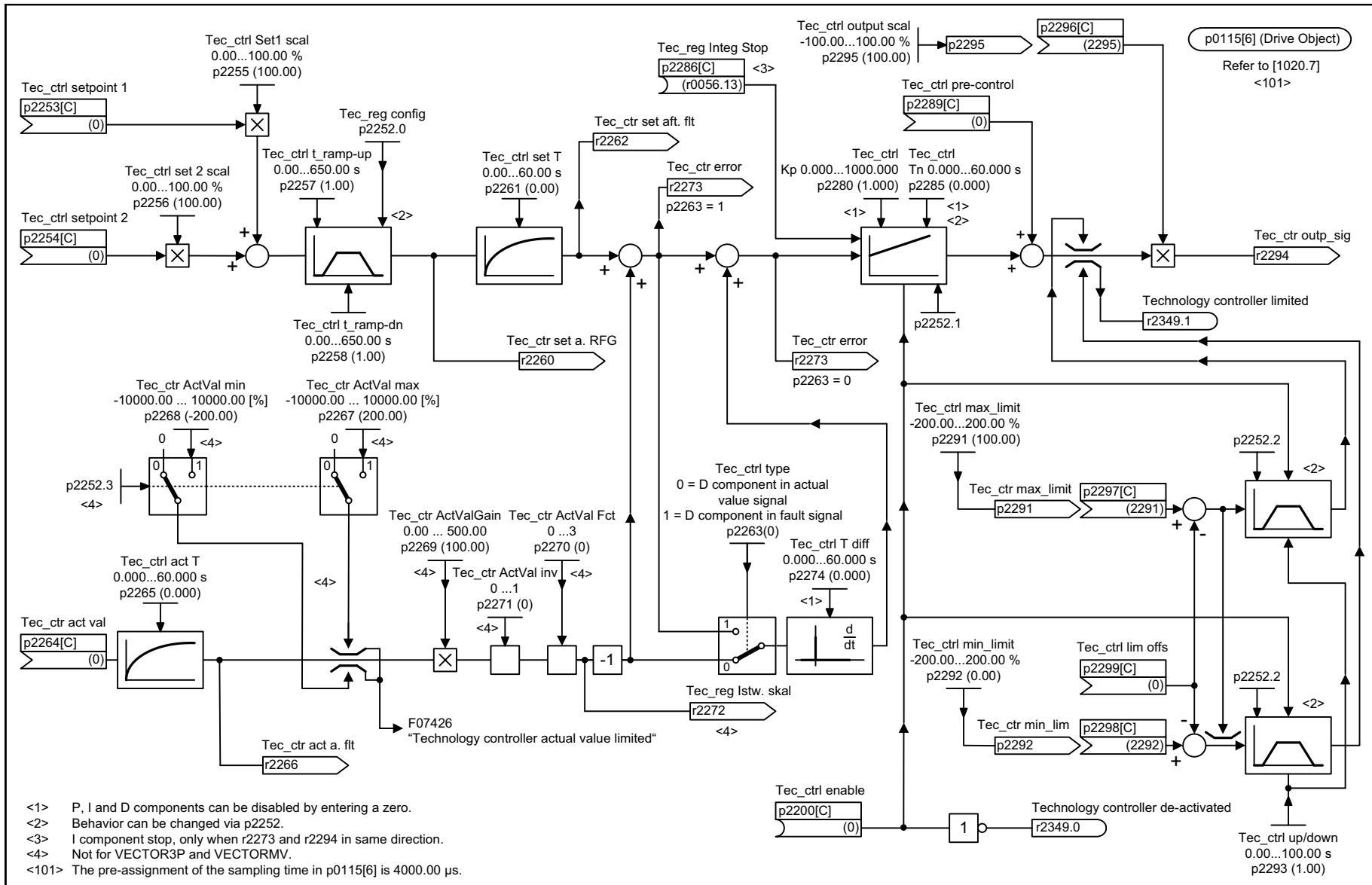
Fig. 2-155 7958 – Closed-loop control (r0108.16 = 1)
