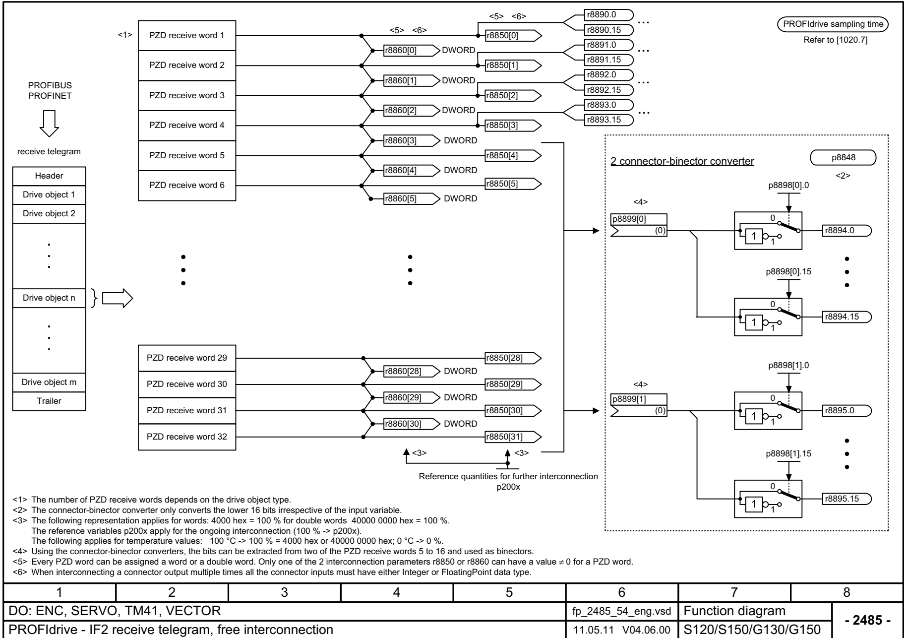
Fig. 2-57 2485 – IF2 receive telegram, free interconnection
