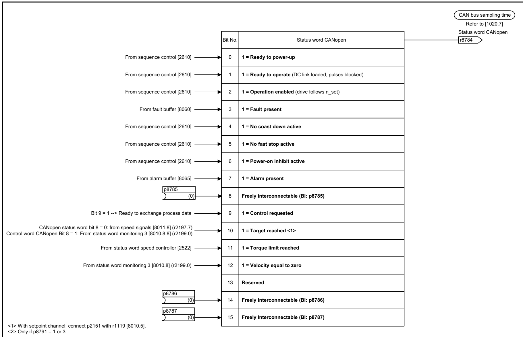
Fig. 2-189 9226 – Status word, CANopen
