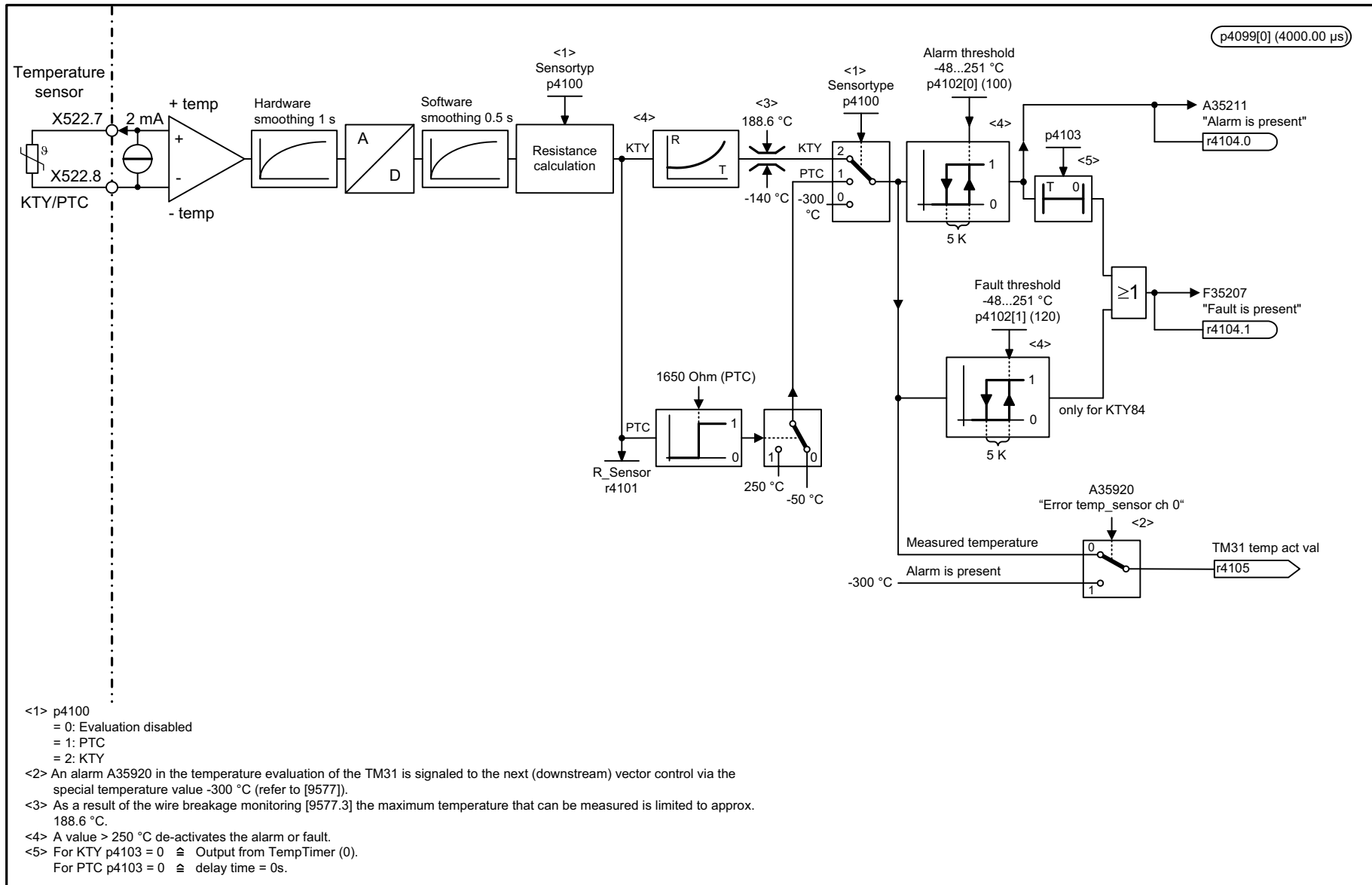
Fig. 2-198 9576 – Temperature evaluation (KTY/PTC)
