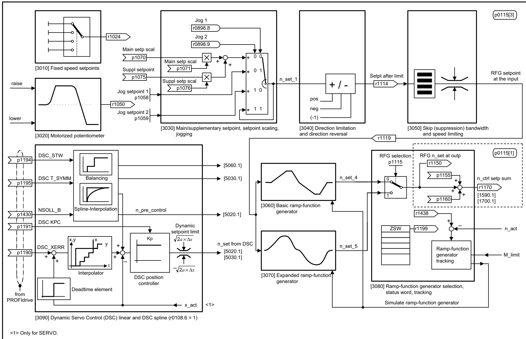
Fig. 2-8 1550 – Setpoint channel
