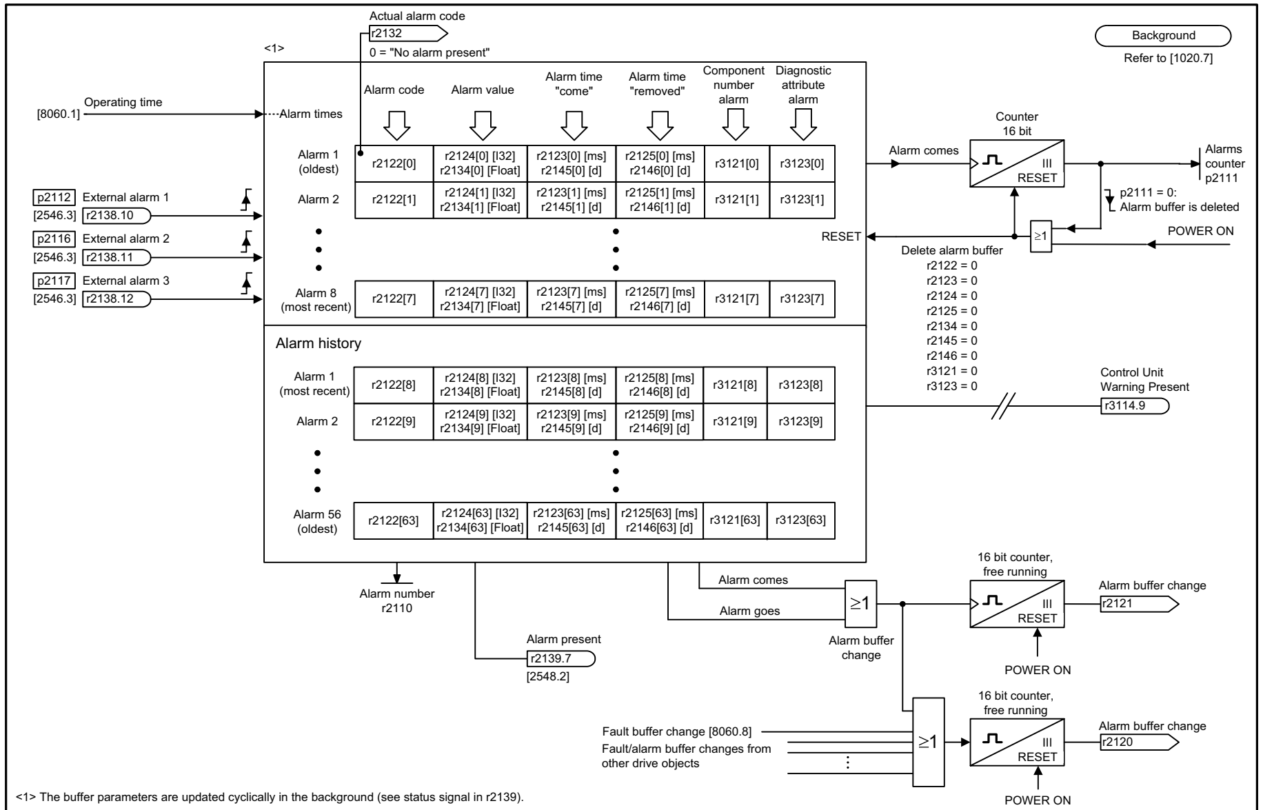
Fig. 2-165 8065 – Alarm buffer
