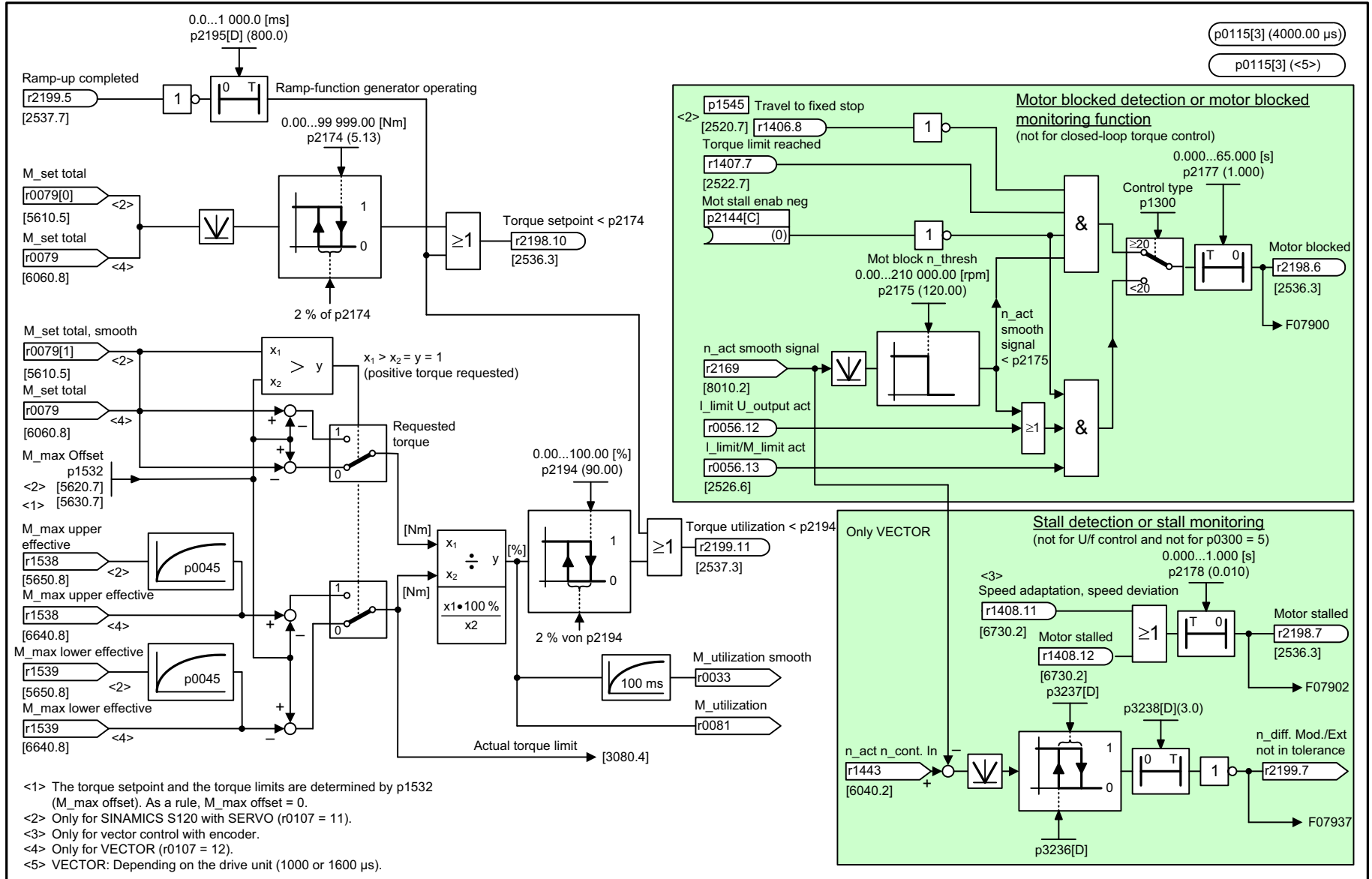
Fig. 2-159 8012 – Torque signals, motor locked/stalled
