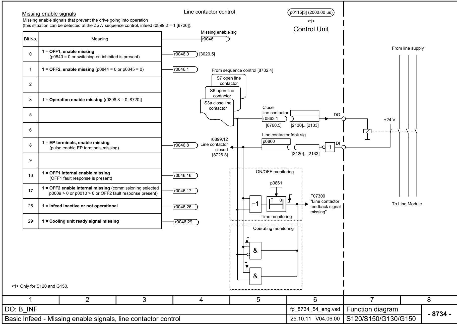
Fig. 2-177 8734 – Missing enable signals, line contactor control
