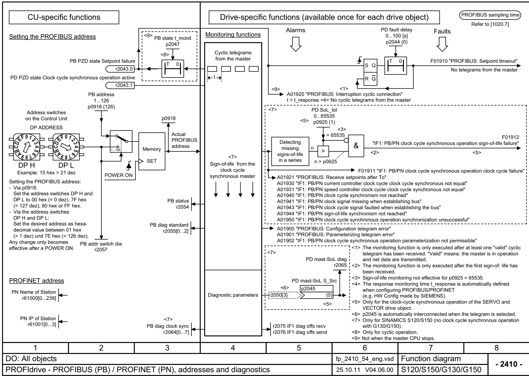
Fig. 2-26 2410 – PROFIBUS (PB) / PROFINET (PN), addresses and diagnostics
