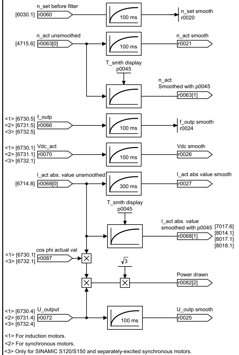
Fig. 2-145 6799 – Display signals
