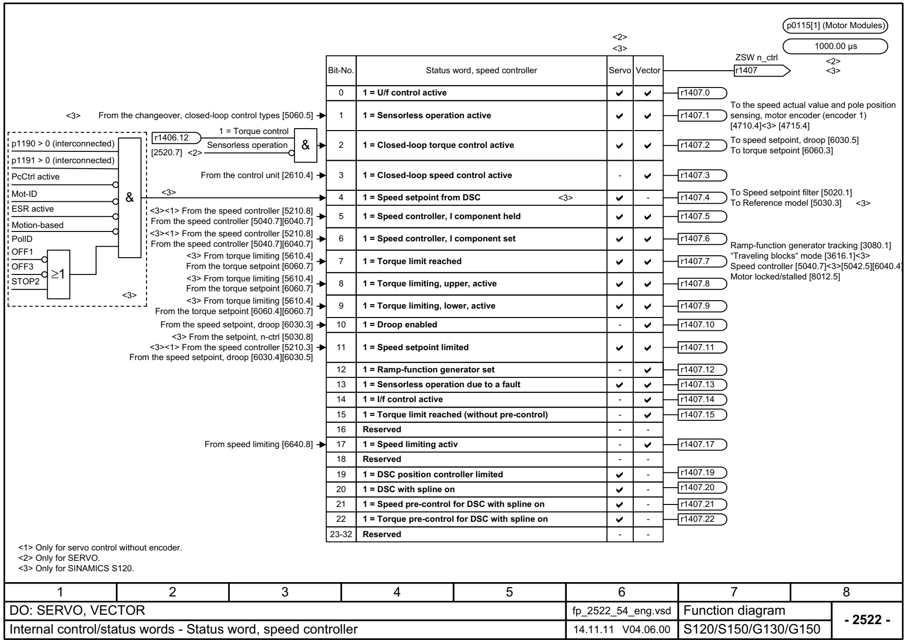
Fig. 2-72 2522 – Status word, speed controller
