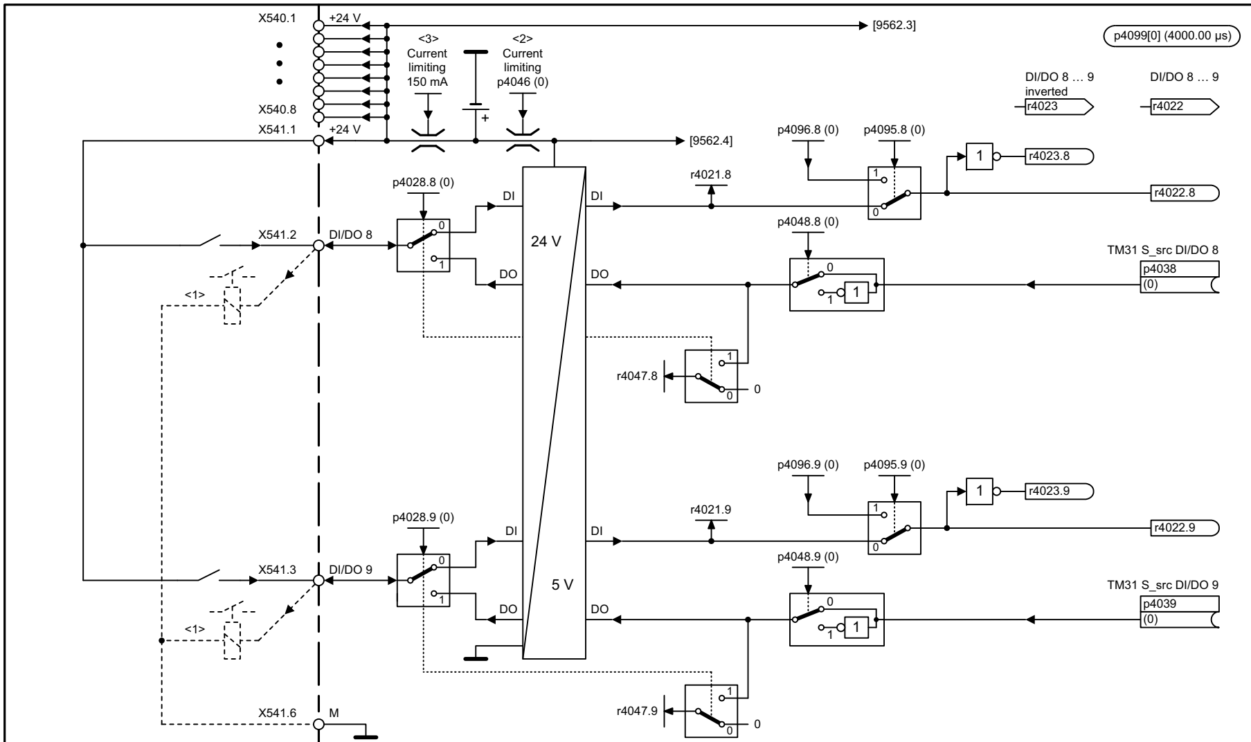
Fig. 2-193 9560 – Digital inputs/outputs, bidirectional (DI/DO 8 to DI/DO 9)
