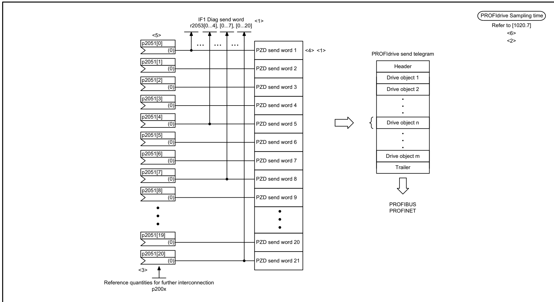
Fig. 2-56 2483 – IF1 send telegram, free interconnection via BICO (p0922 = 999)
