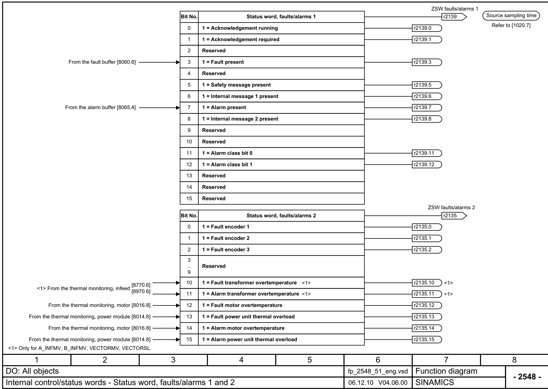
Fig. 2-79 2548 – Status word, faults/alarms 1 and 2
