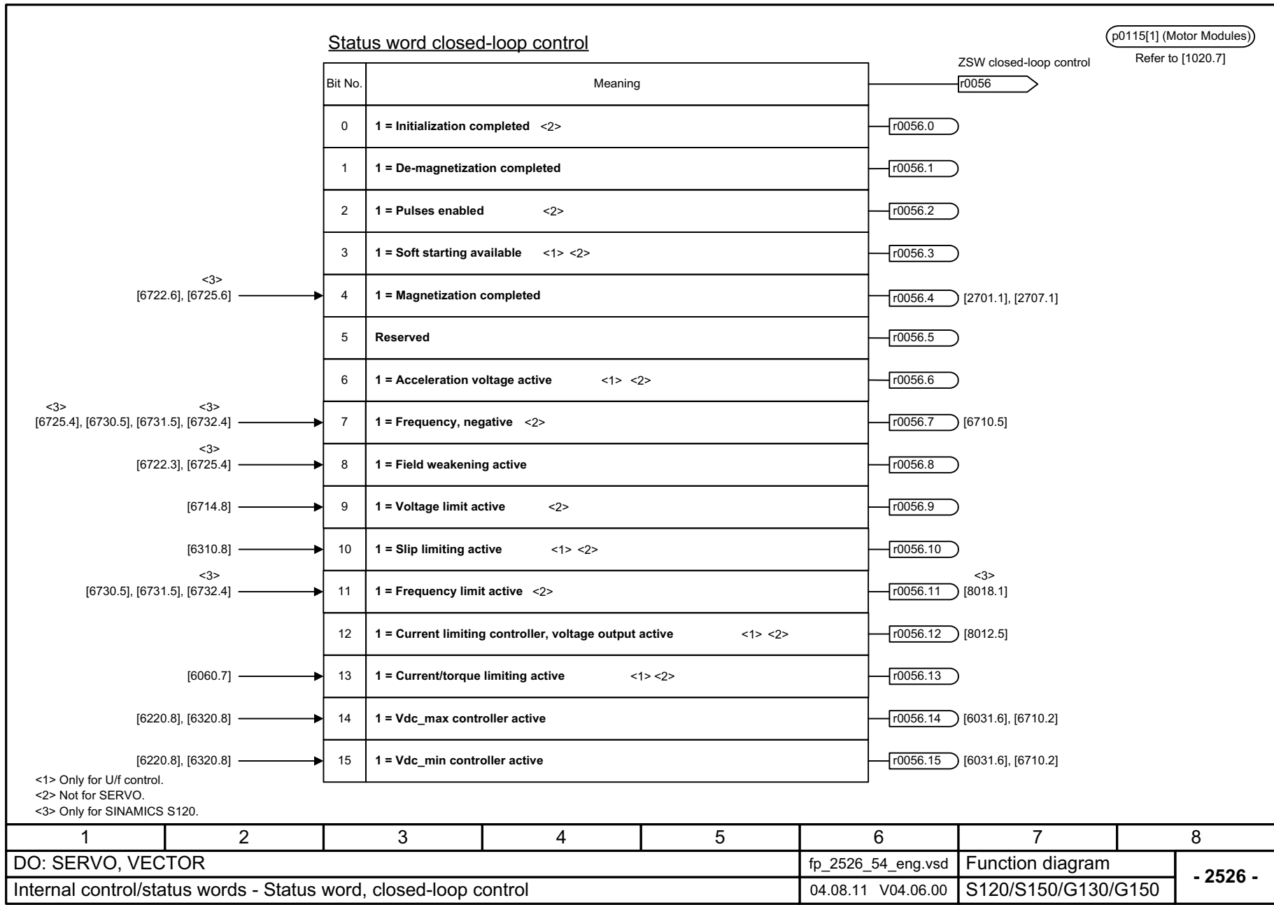
Fig. 2-73 2526 – Status word, closed-loop control
