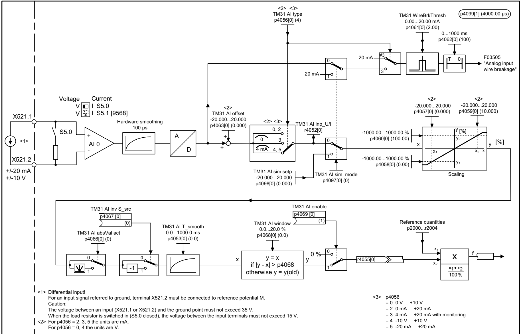
Fig. 2-195 9566 – Analog input 0 (AI 0)
