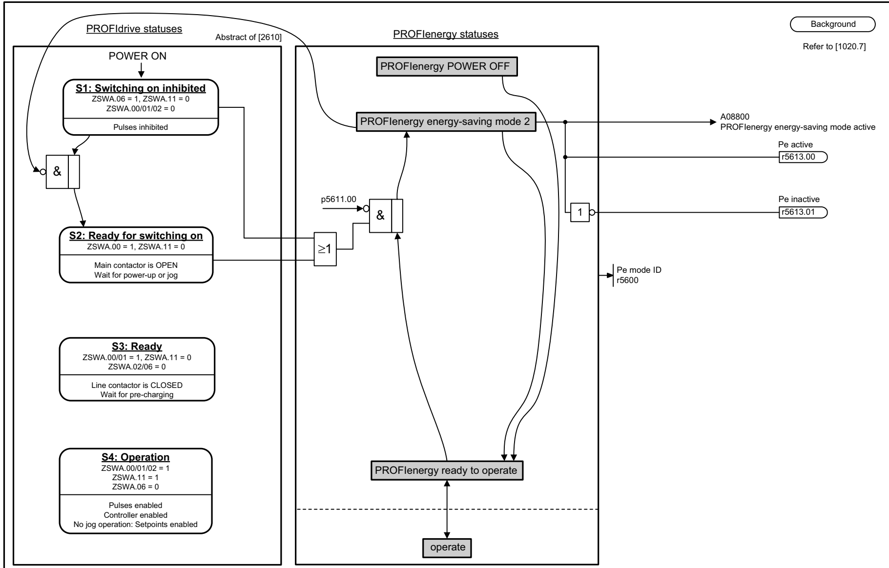
Fig. 2-25 2382 – States
