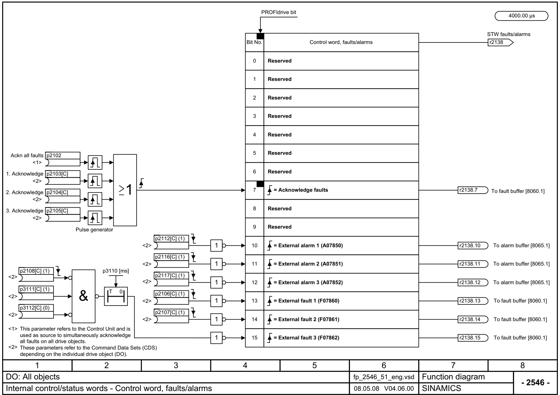
Fig. 2-78 2546 – Control word, faults/alarms
