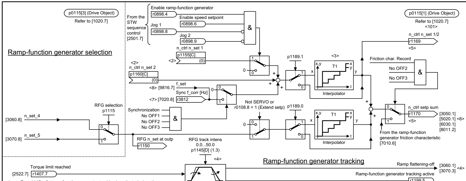
Fig. 2-121 3080 – Ramp-function generator selection, status word, tracking
