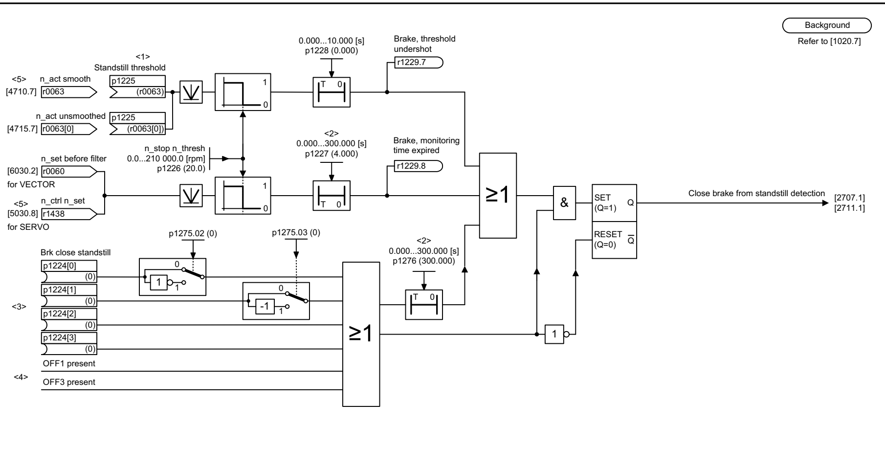
Fig. 2-83 2704 – Extended brake control, zero-speed detection (r0108.14 = 1)
