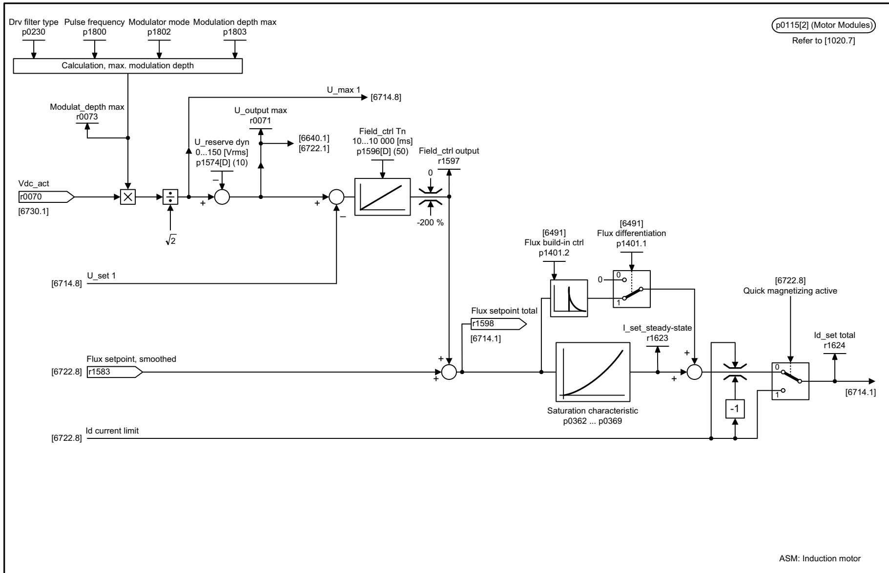
Fig. 2-141 6723 – Field weakening controller, flux controller (ASM, p0300 = 1)
