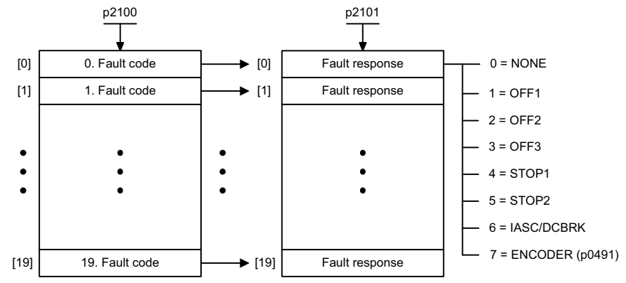
Fig. 2-167 8075 – Fault/alarm configuration
