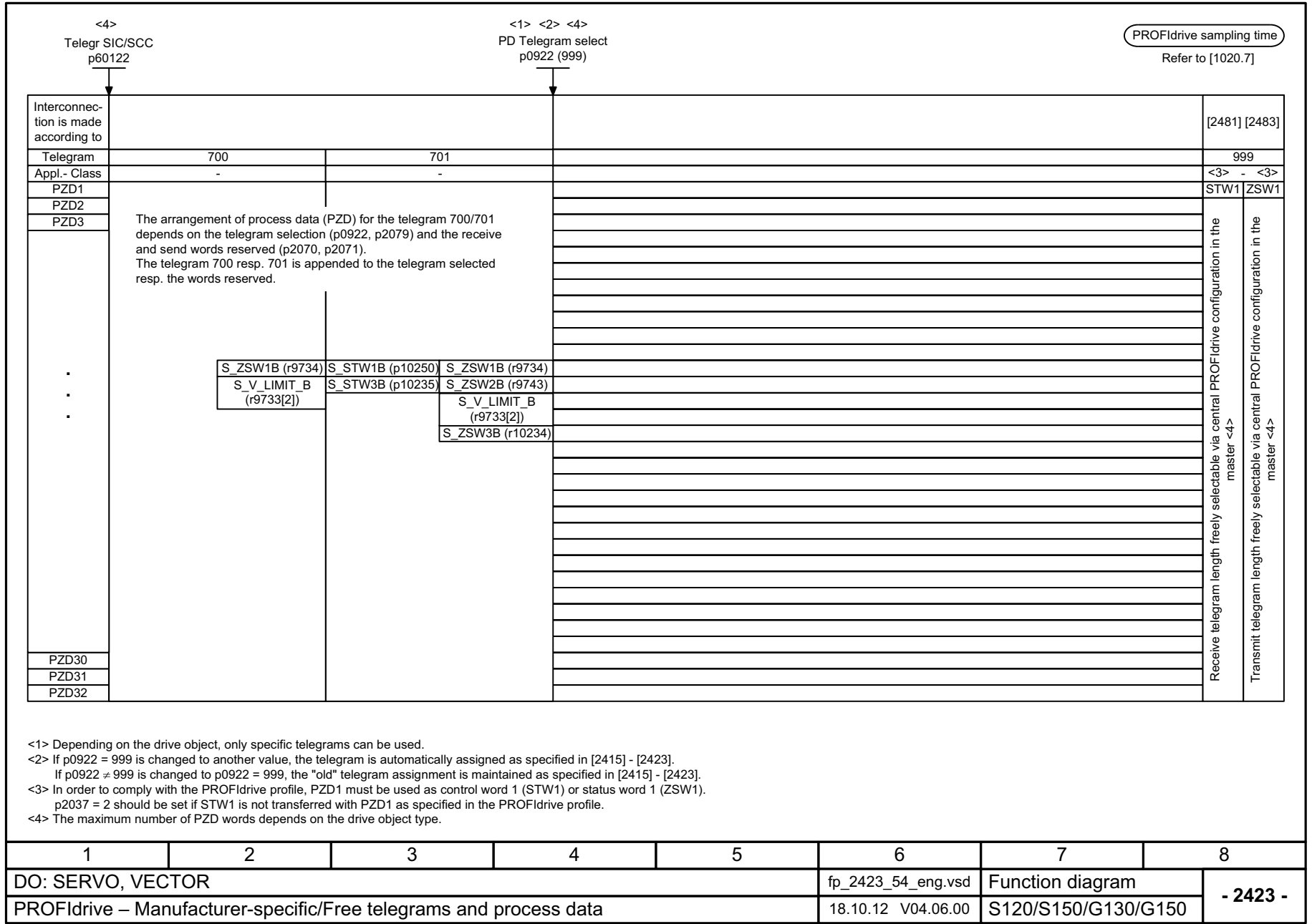
Fig. 2-33 2423 – Manufacturer-specific/free telegrams and process data
