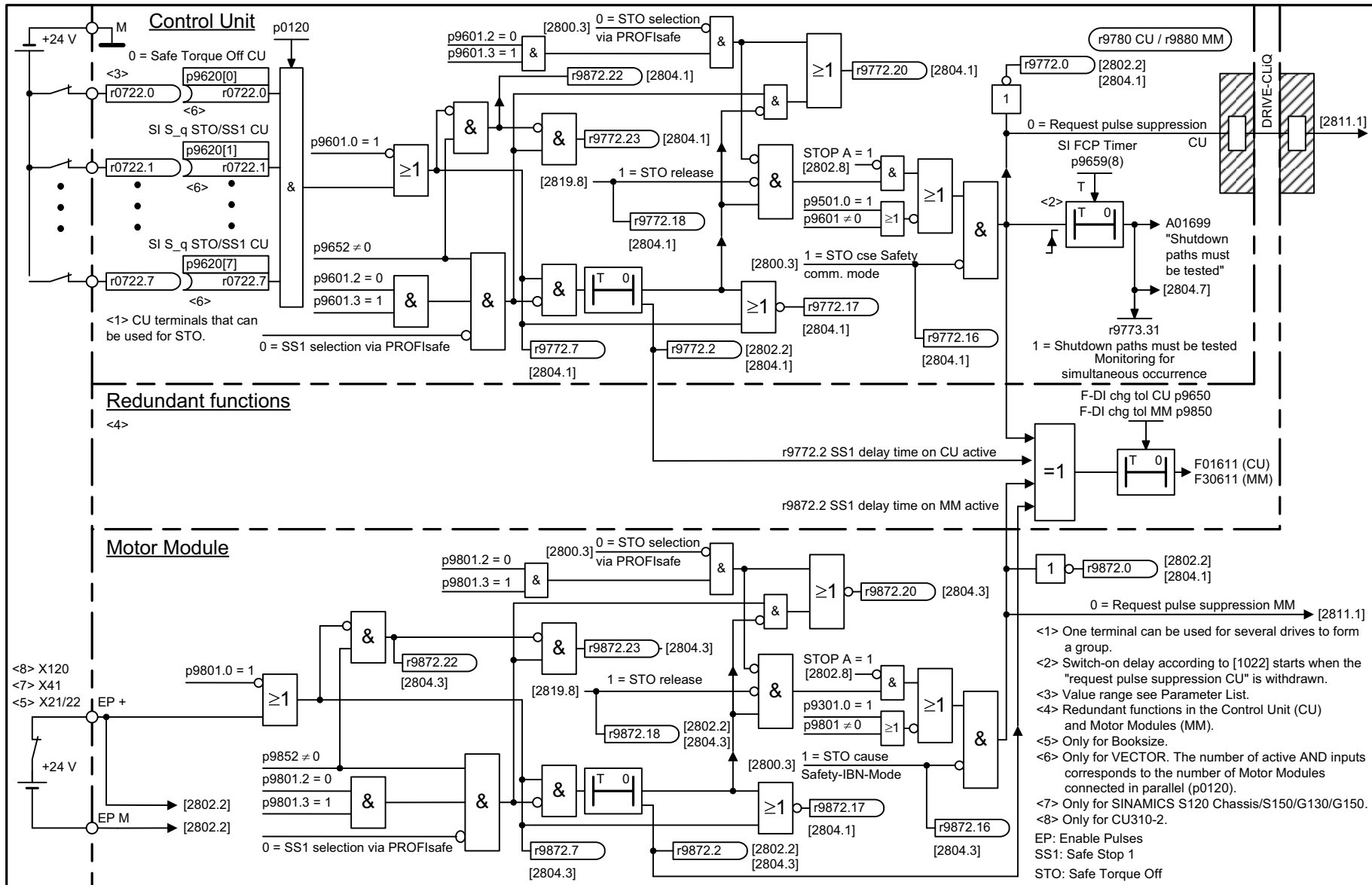
Fig. 2-90 2810 – STO (Safe Torque Off), SS1 (Safe Stop 1)
