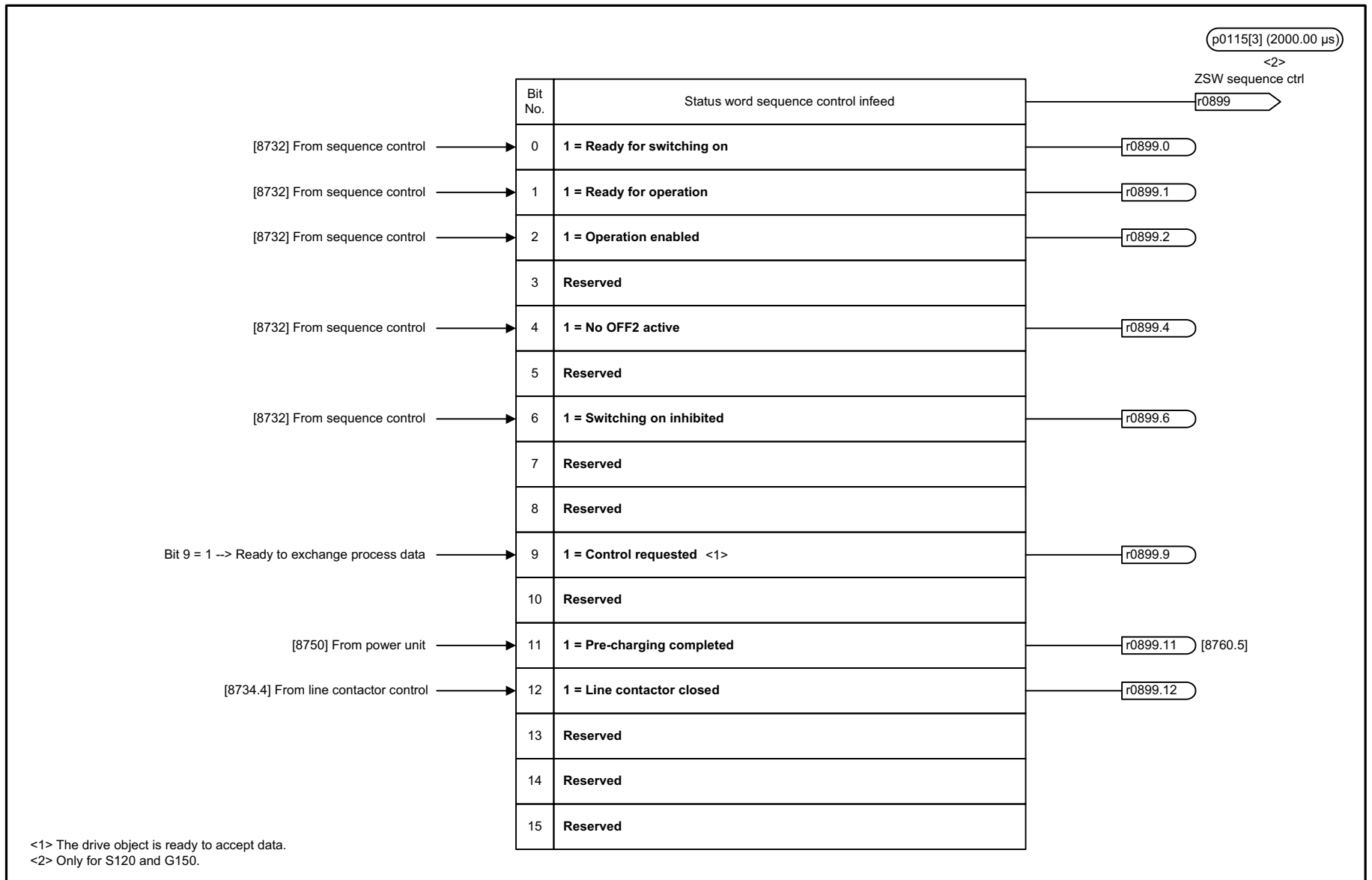
Fig. 2-175 8726 – Status word, sequence control infeed
