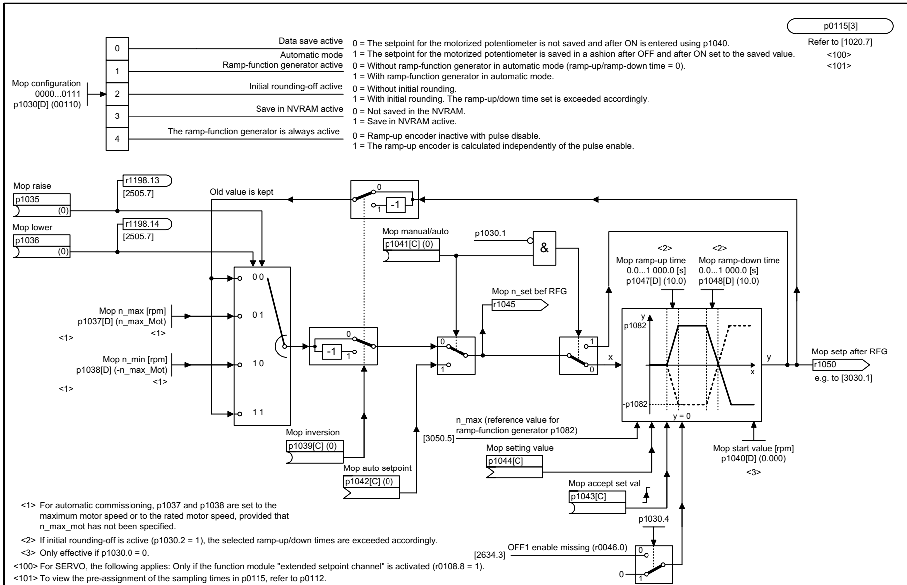
Fig. 2-115 3020 – Motorized potentiometer
