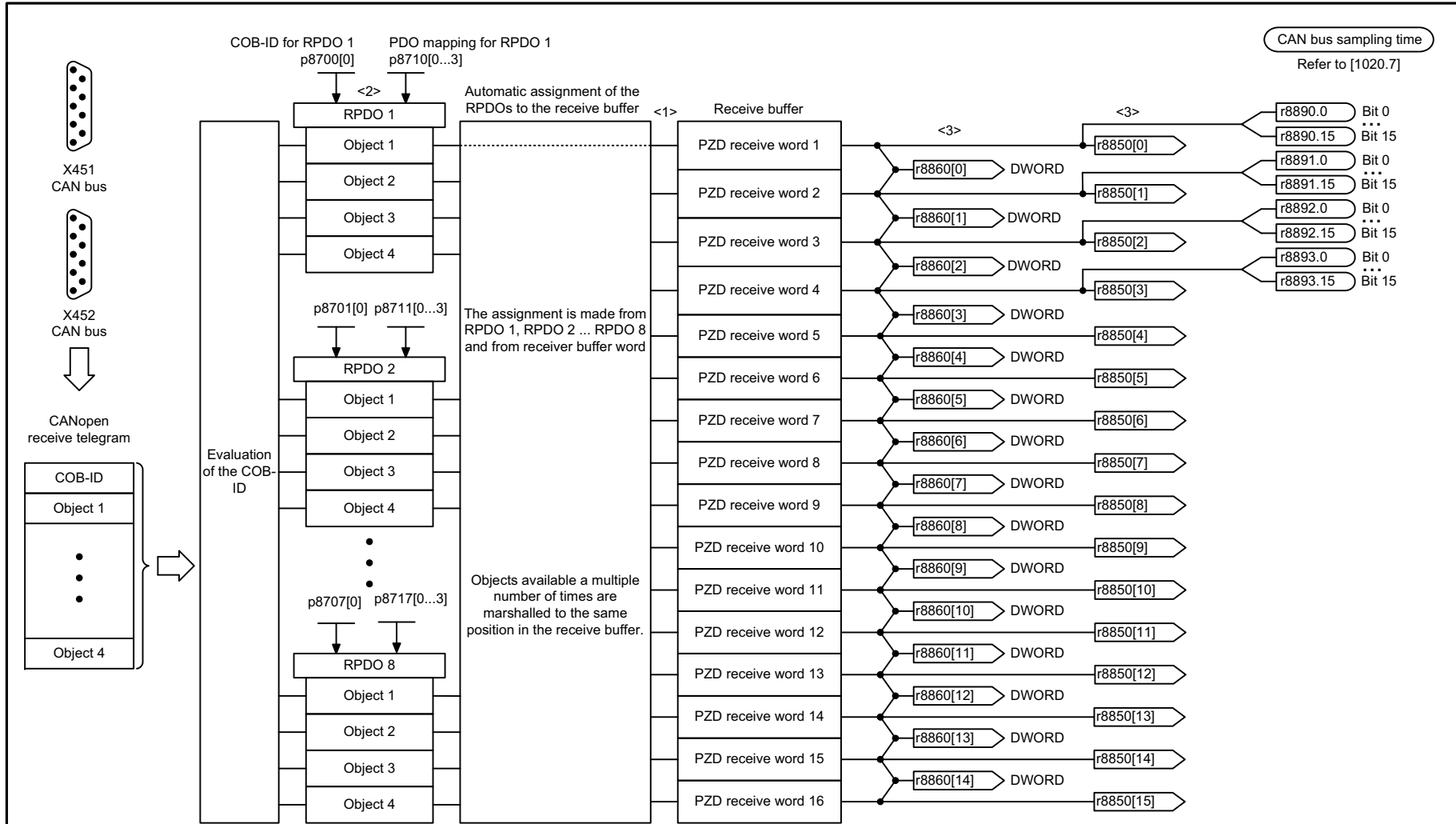
Fig. 2-184 9204 – Receive telegram, free PDO mapping (p8744 = 2)
