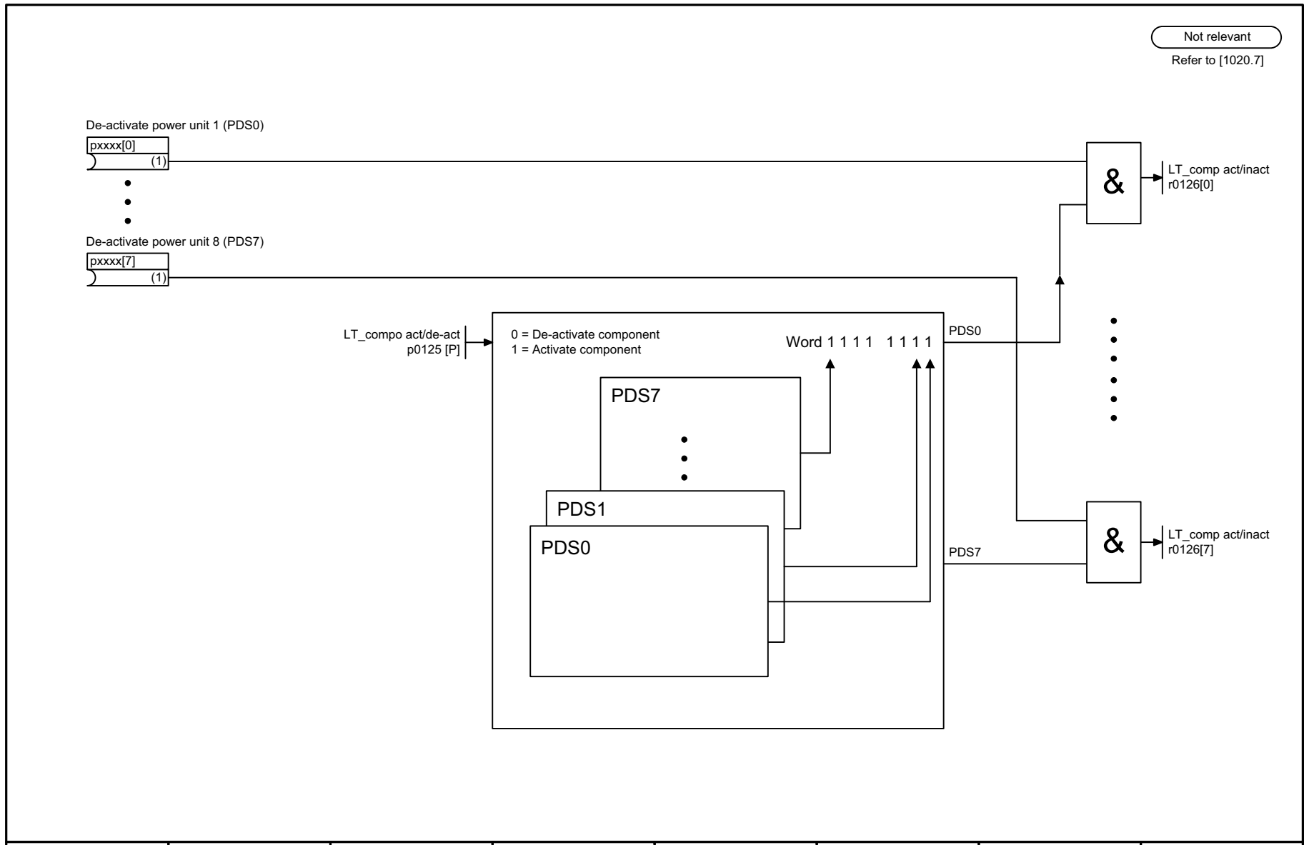
Fig. 2-173 8580 – Power unit data sets (PDS)
