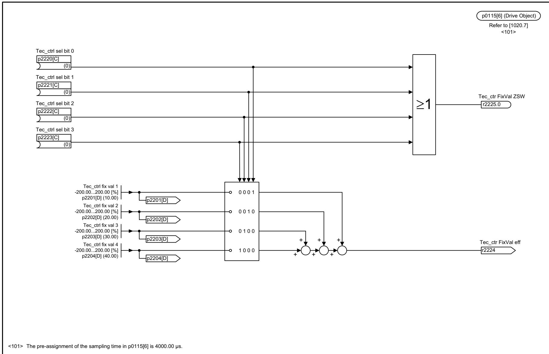
Fig. 2-153 7951 – Fixed value selection direct (r0108.16 = 1 and p2216 = 1)
