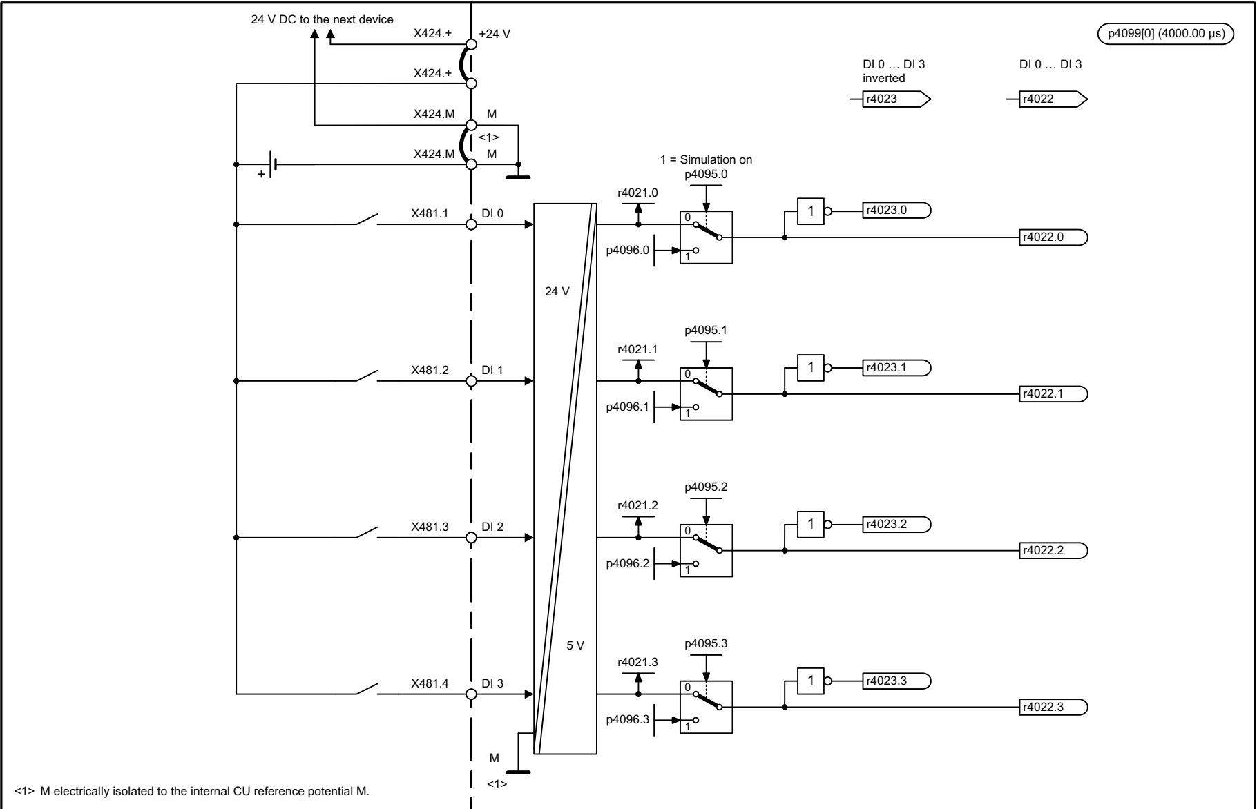
Fig. 2-180 9100 – Digital inputs, electrically isolated (DI 0 ... DI 3)
