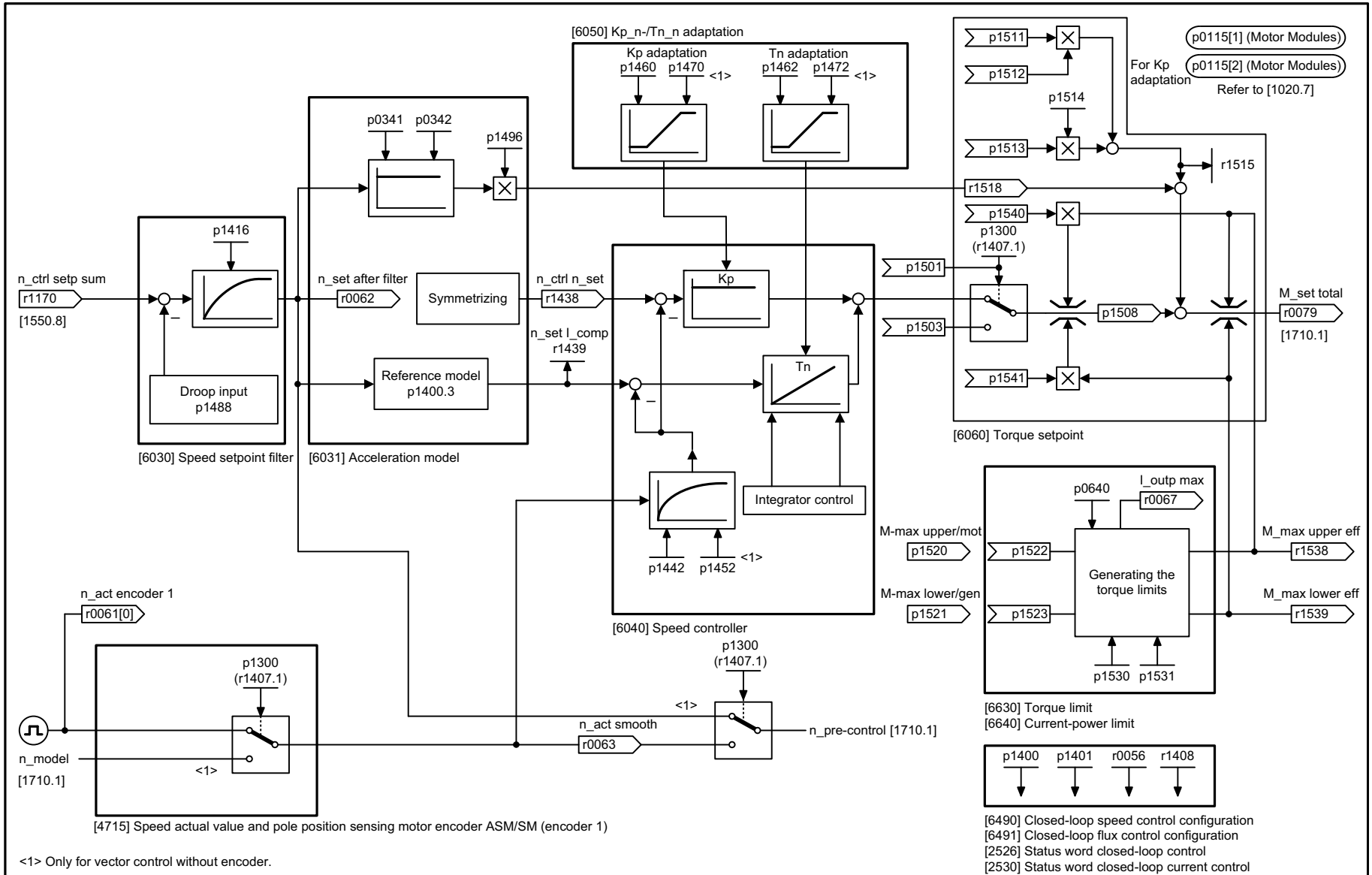
Fig. 2-11 1700 – Vector control, speed control and generation of the torque limits
