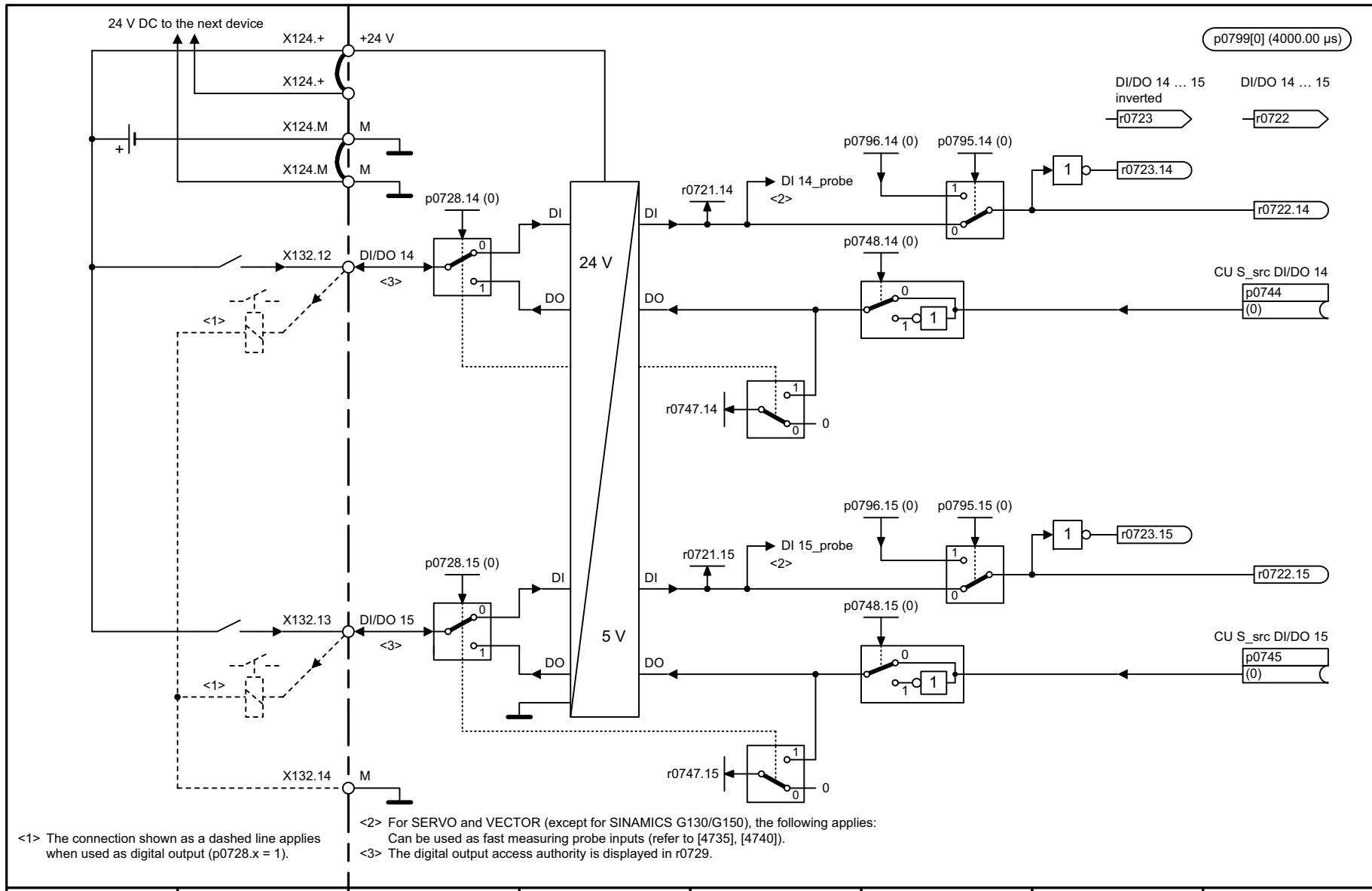
Fig. 2-23 2133 – Digital inputs/outputs, bidirectional (DI/DO 14 ... DI/DO 15)
