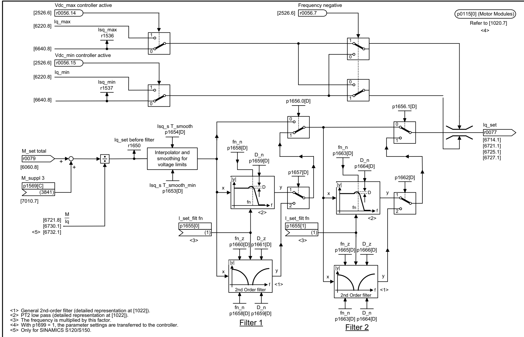
Fig. 2-137 6710 – Current setpoint filter
