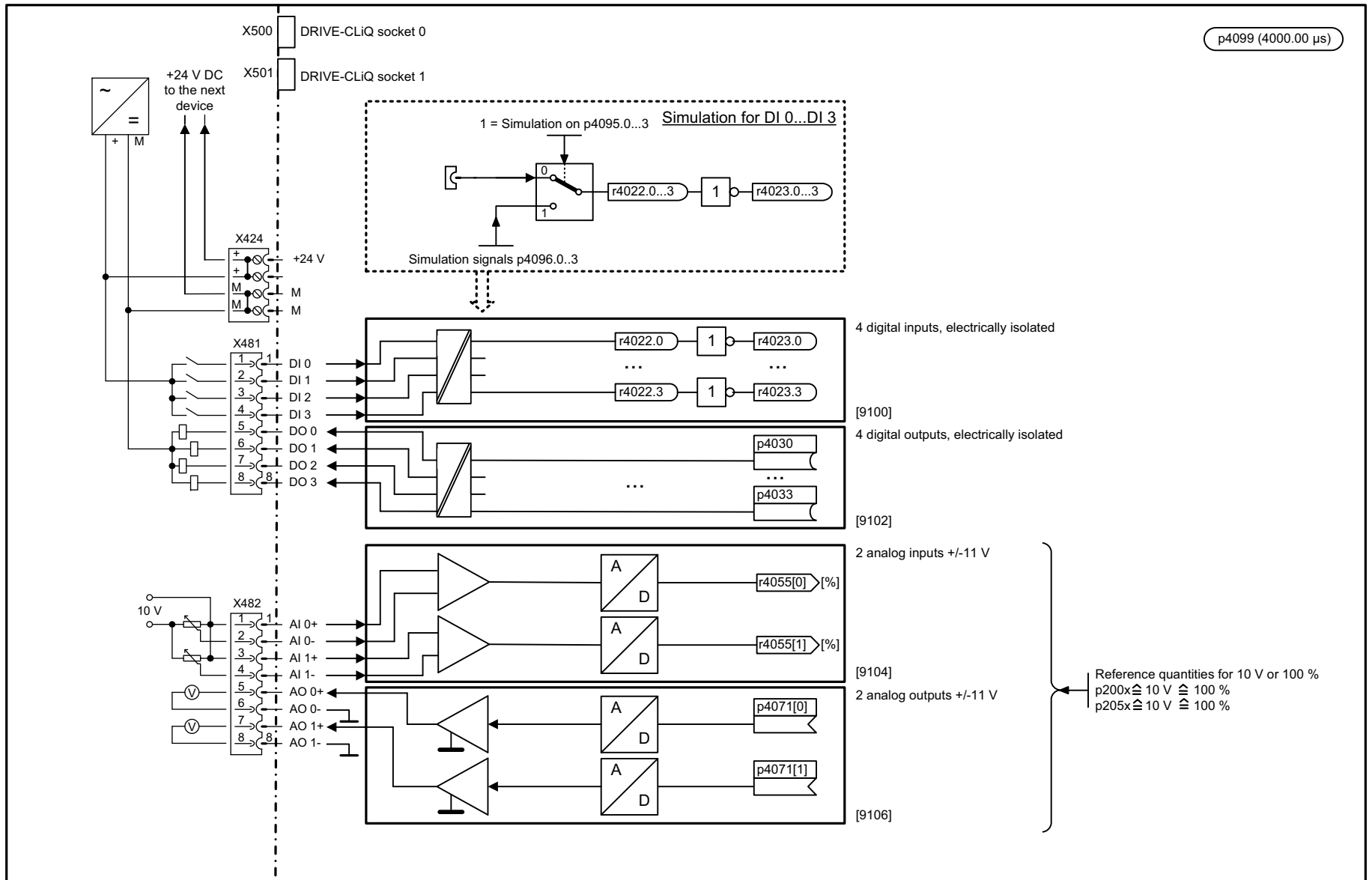
Fig. 2-15 1790 – Terminal Board 30 (TB30)
