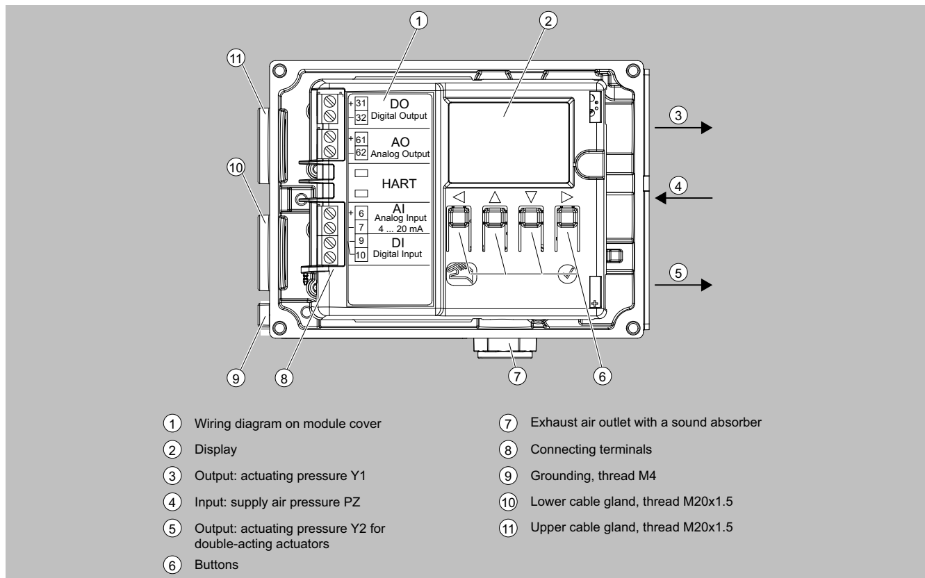
SIPART PS100, enclosure with open lid
