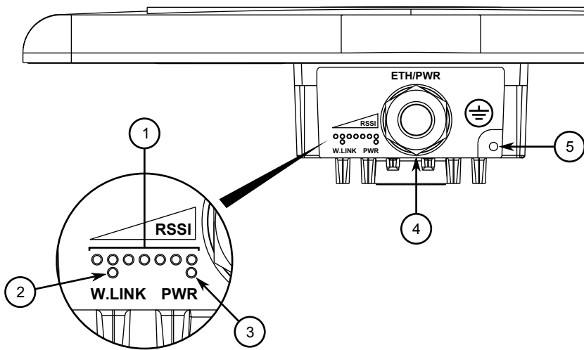
Figure 1: RUGGEDCOM WIN5258
