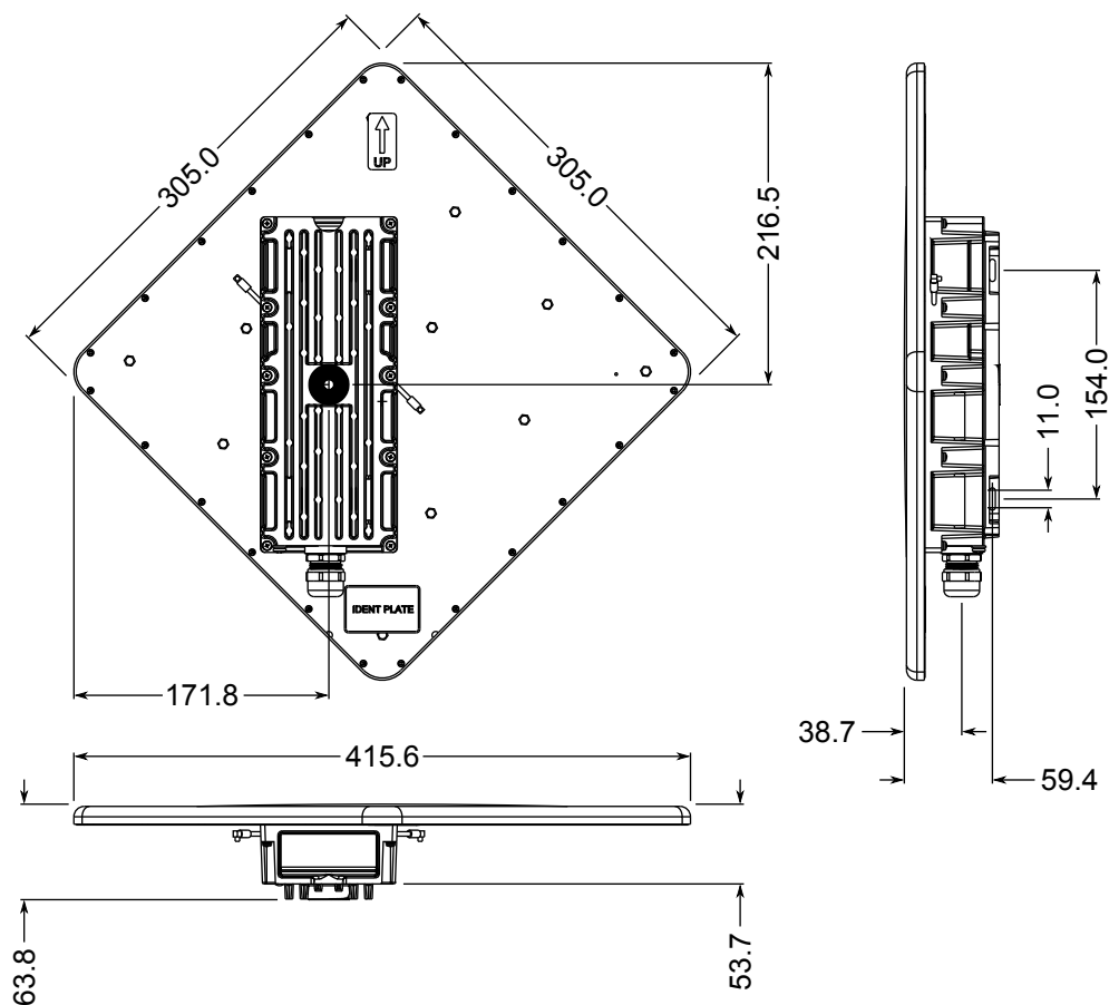
Figure 17: Overall Dimensions
