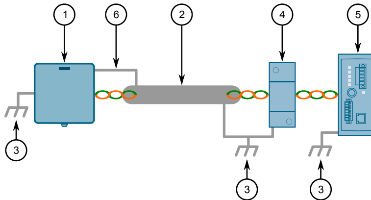
Figure 7: Typical Outdoor Installation
