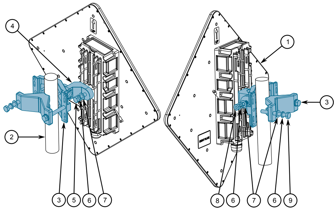
Figure 5: Mounting the Subscriber Station to a Small Pole
