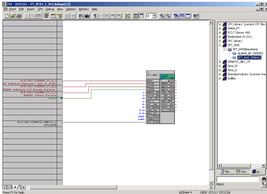
Fig. 5-1 Block SFTA in CFC
