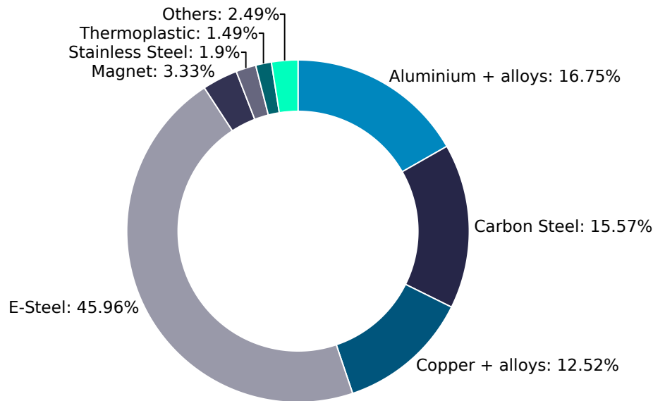
Product Weight 12.6 kg
