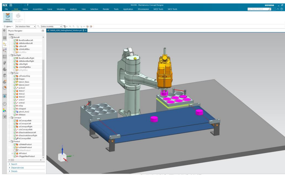
Figure 3-7 The MCD simulation is started
