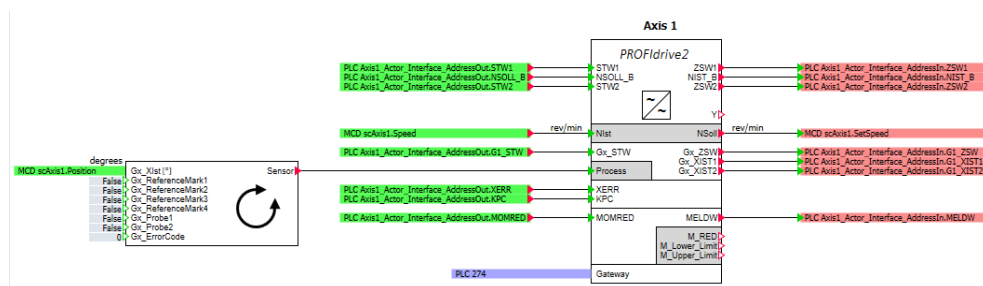
Figure 2-33 Interconnection of signals / SIMIT components of axes 1 and 2
