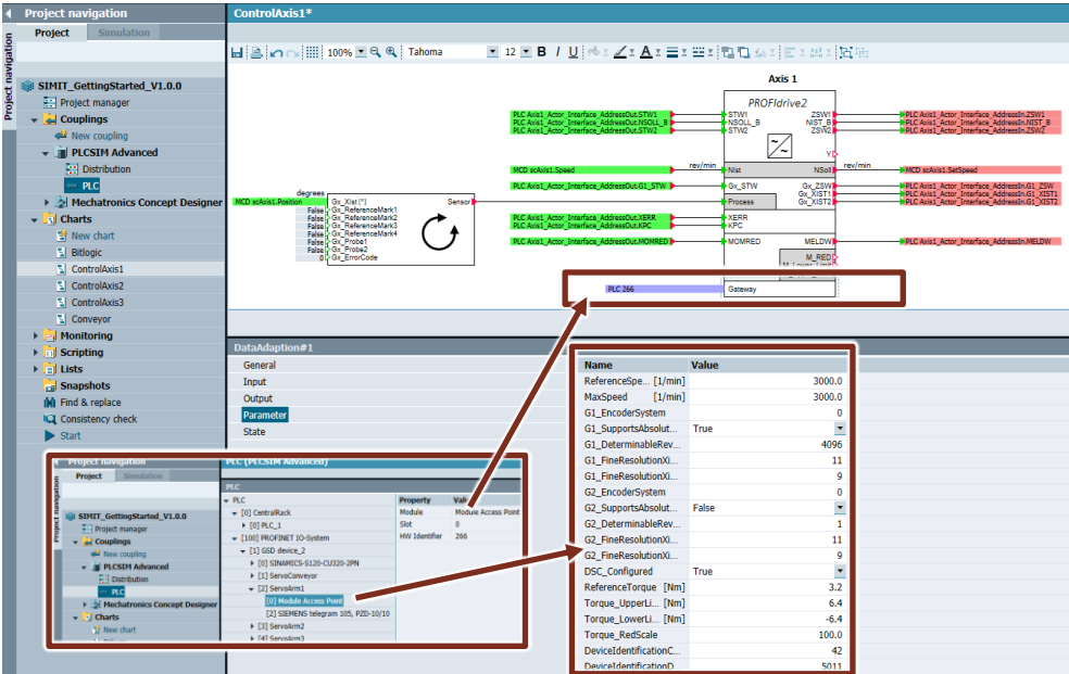
Figure 2-31 Setting the properties of the PROFIdrive block (data adaption) with S7-PLCSIM Advanced V6.0
