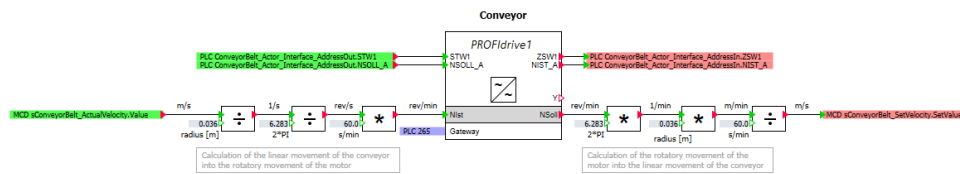
Figure 2-35 Interconnection of signals / SIMIT components of the conveyor
