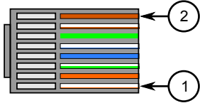
Figure 16: CAT-5e PoE Cable Pin-Out 1. Pin 1 2. Pin 8
