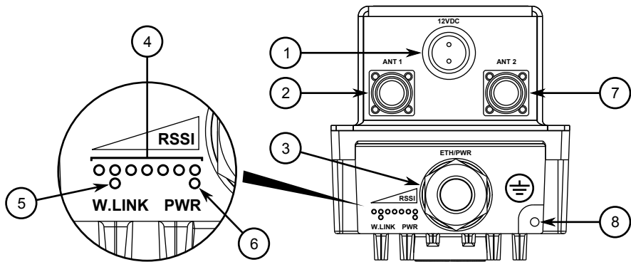
Figure 2: RUGGEDCOM WIN5118 (DC Model)
