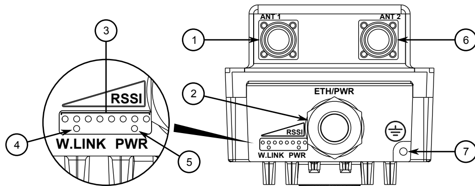
Figure 1: RUGGEDCOM WIN5118 (AC Model)
