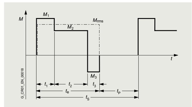
Torque diagram
