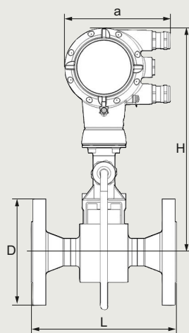
SITRANS FX330 (Vortex), Flanged version with pressure sensor, front view
