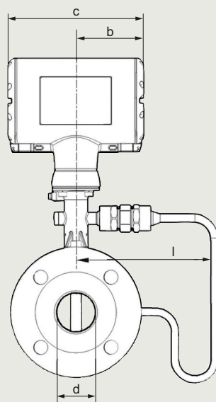
SITRANS FX330 (Vortex), Flanged version with pressure sensor, side view
